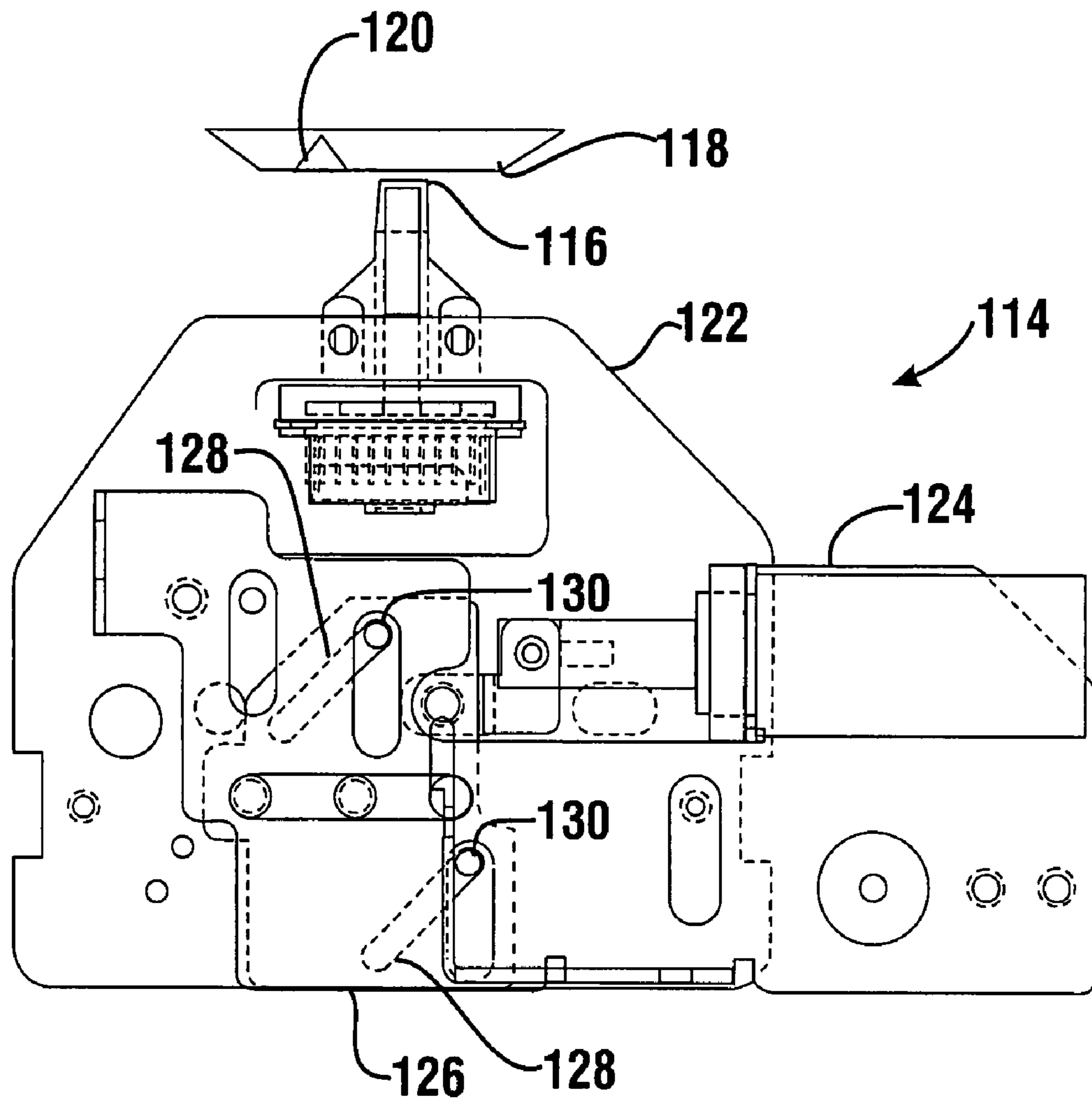
Printing Position
