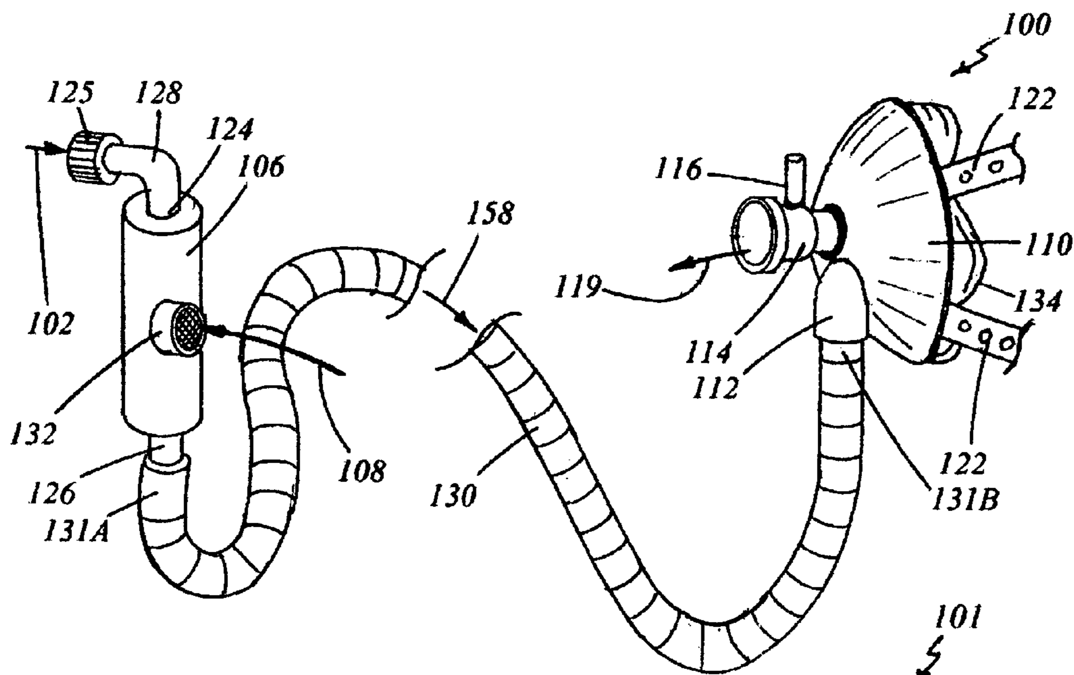
FIG. 1 PRIOR ART
