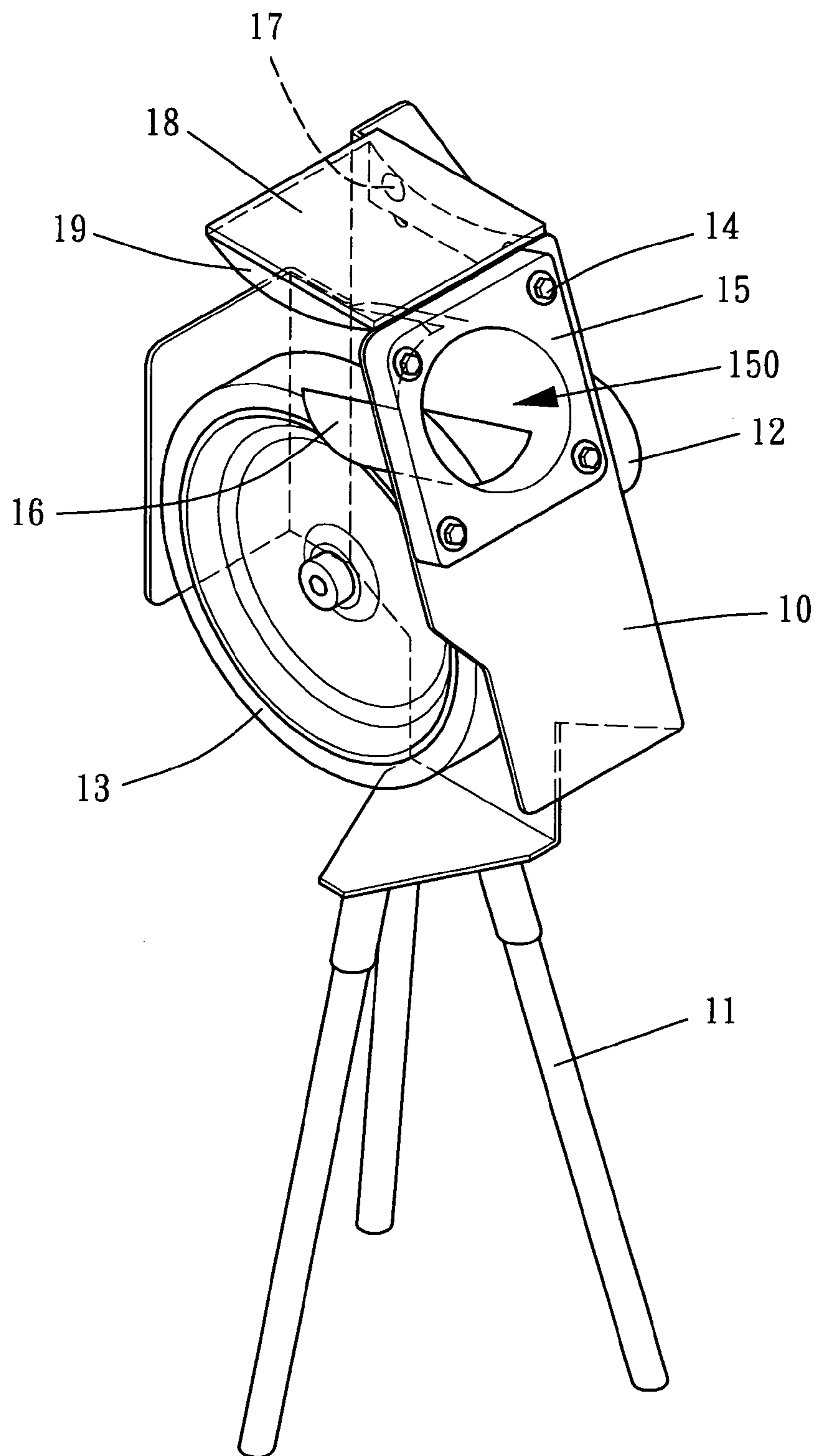
FIG. 7 (PRIOR ART)
