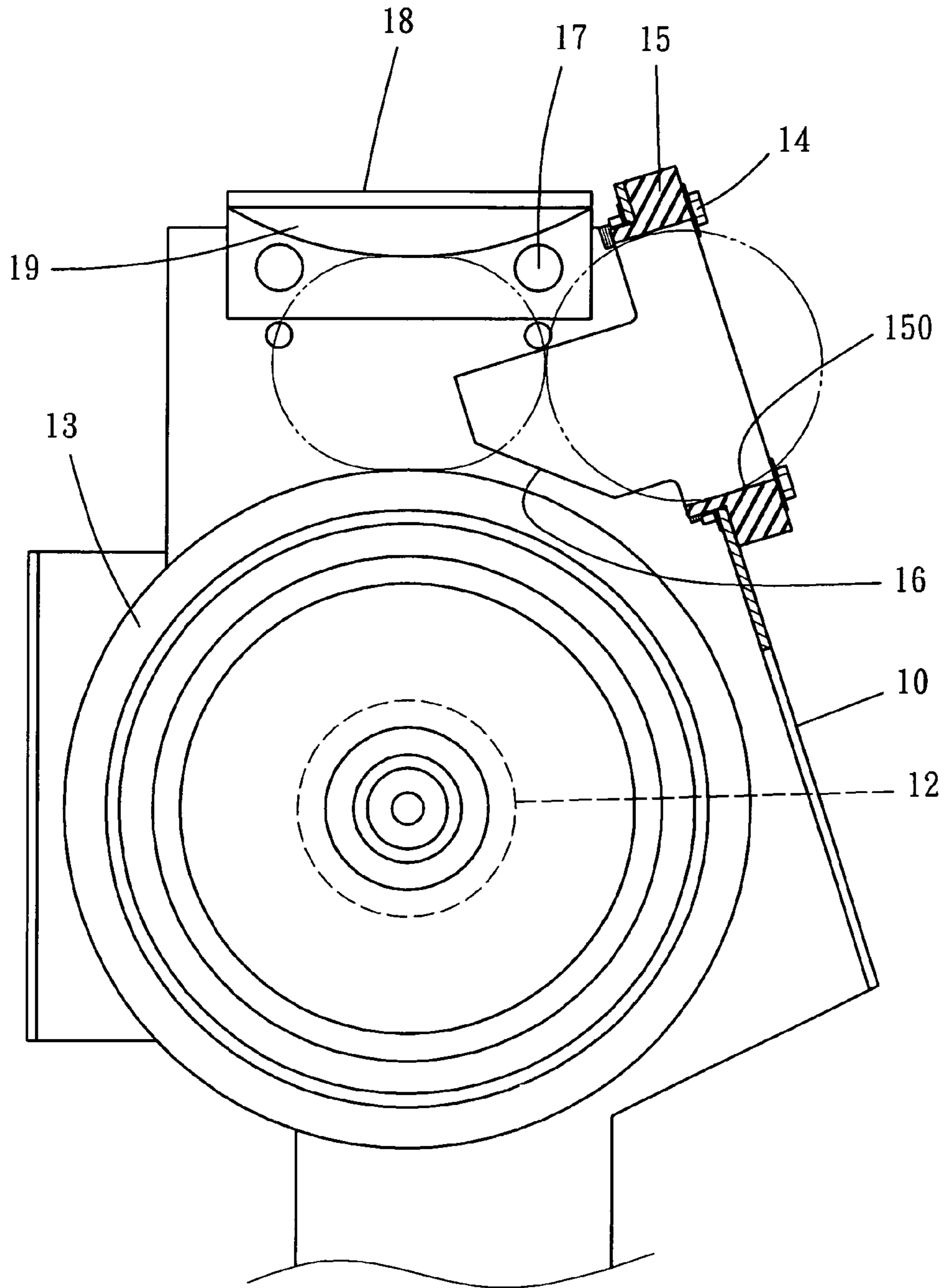
FIG. 8 (PRIOR ART)
