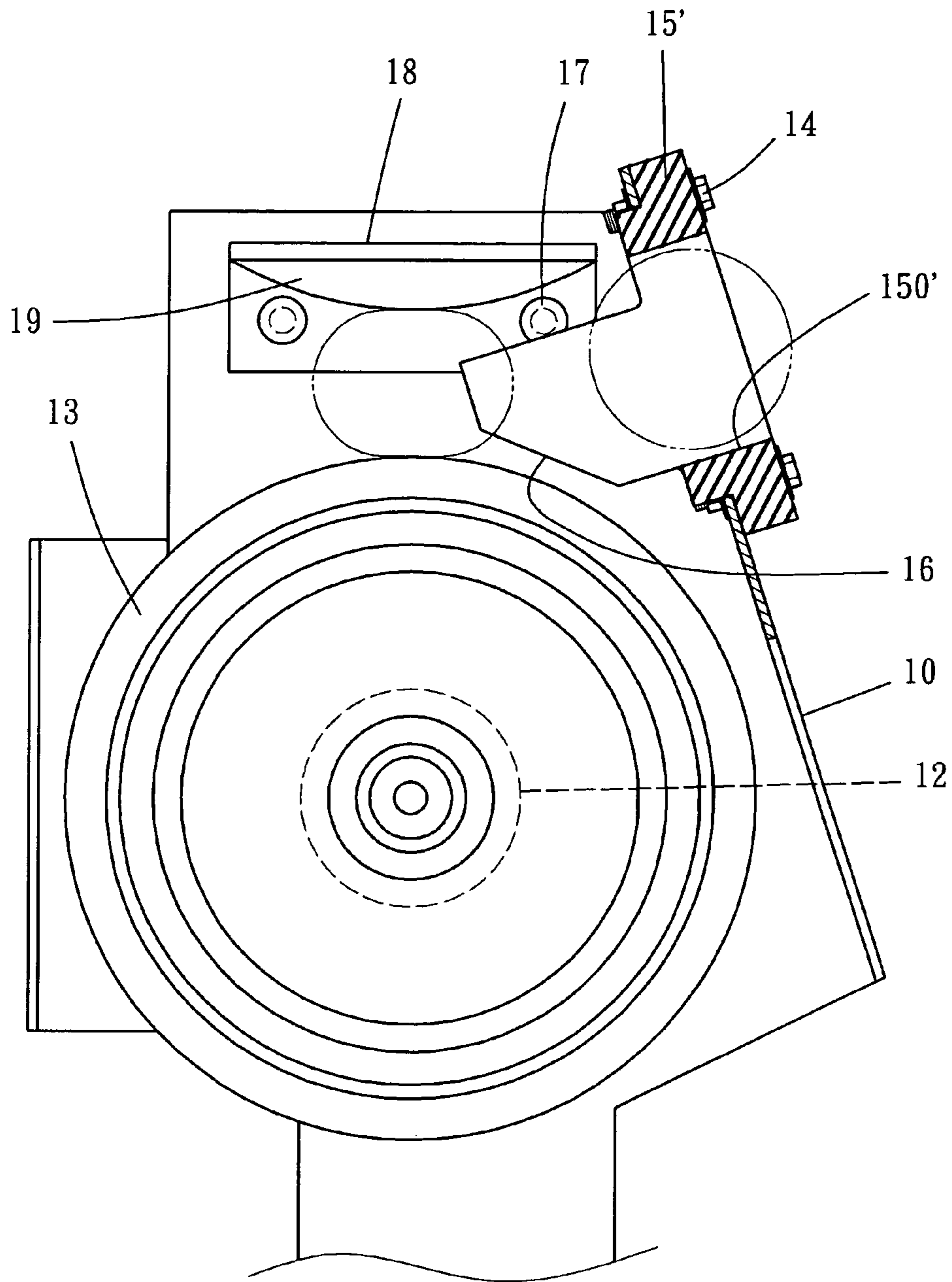
FIG. 9 (PRIOR ART)
