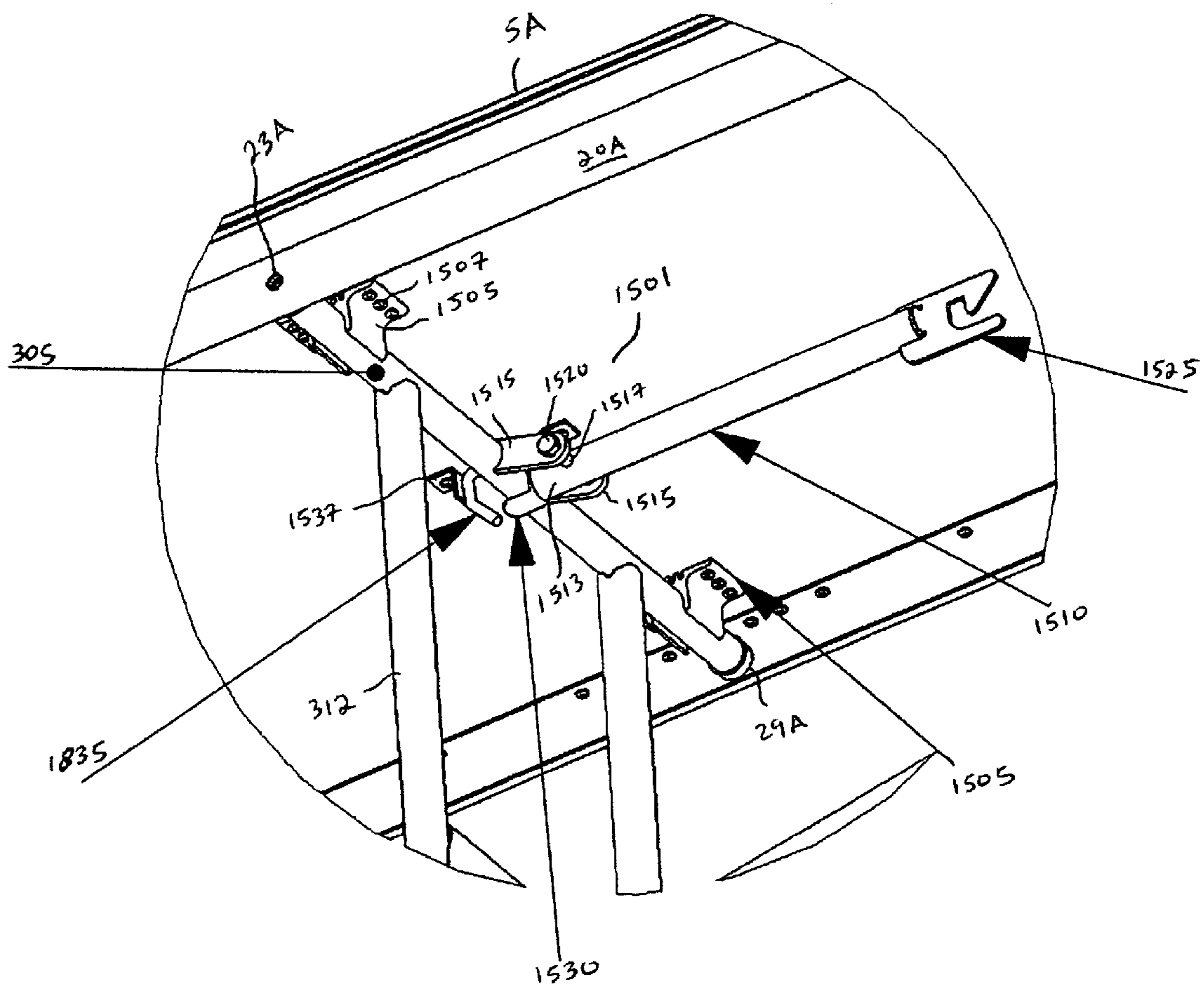
FIG. 15B - Detail D
