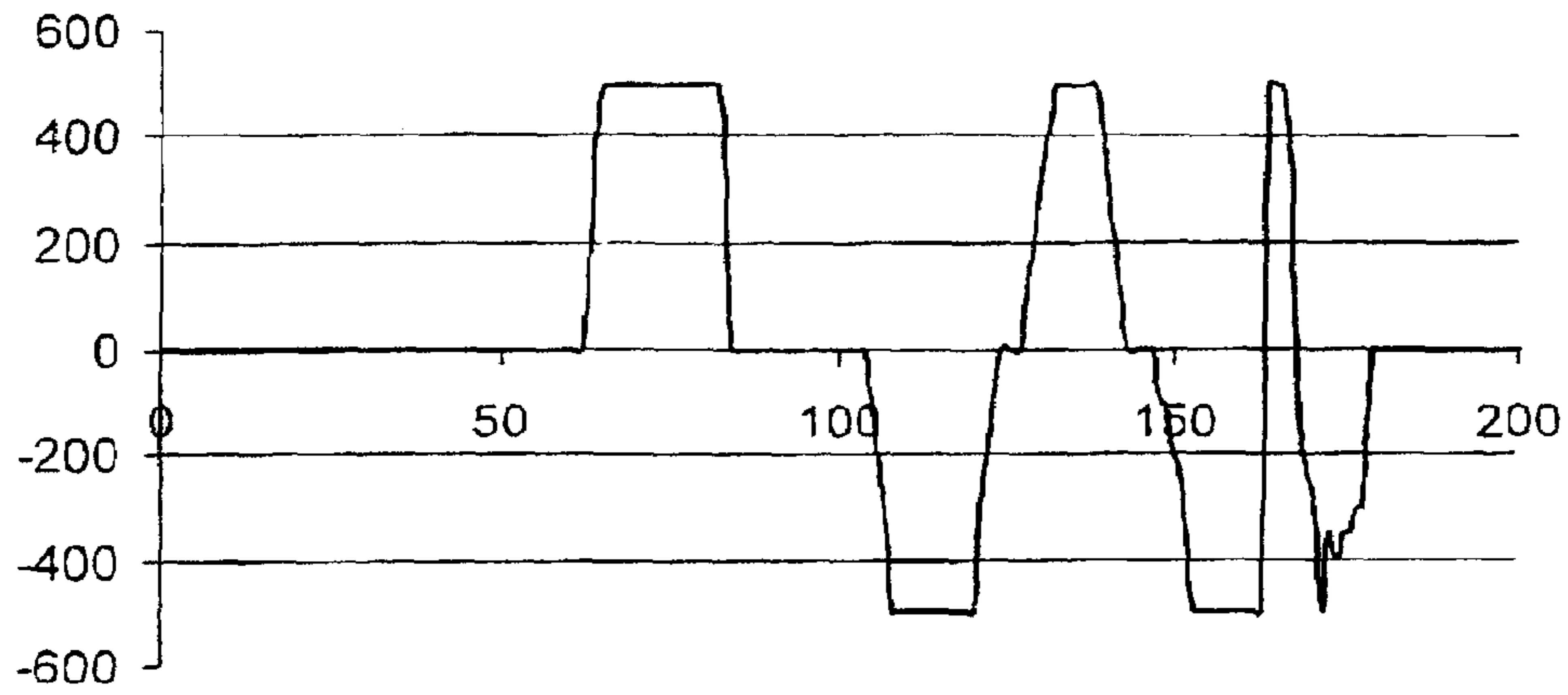
FIG. 8C charge power
