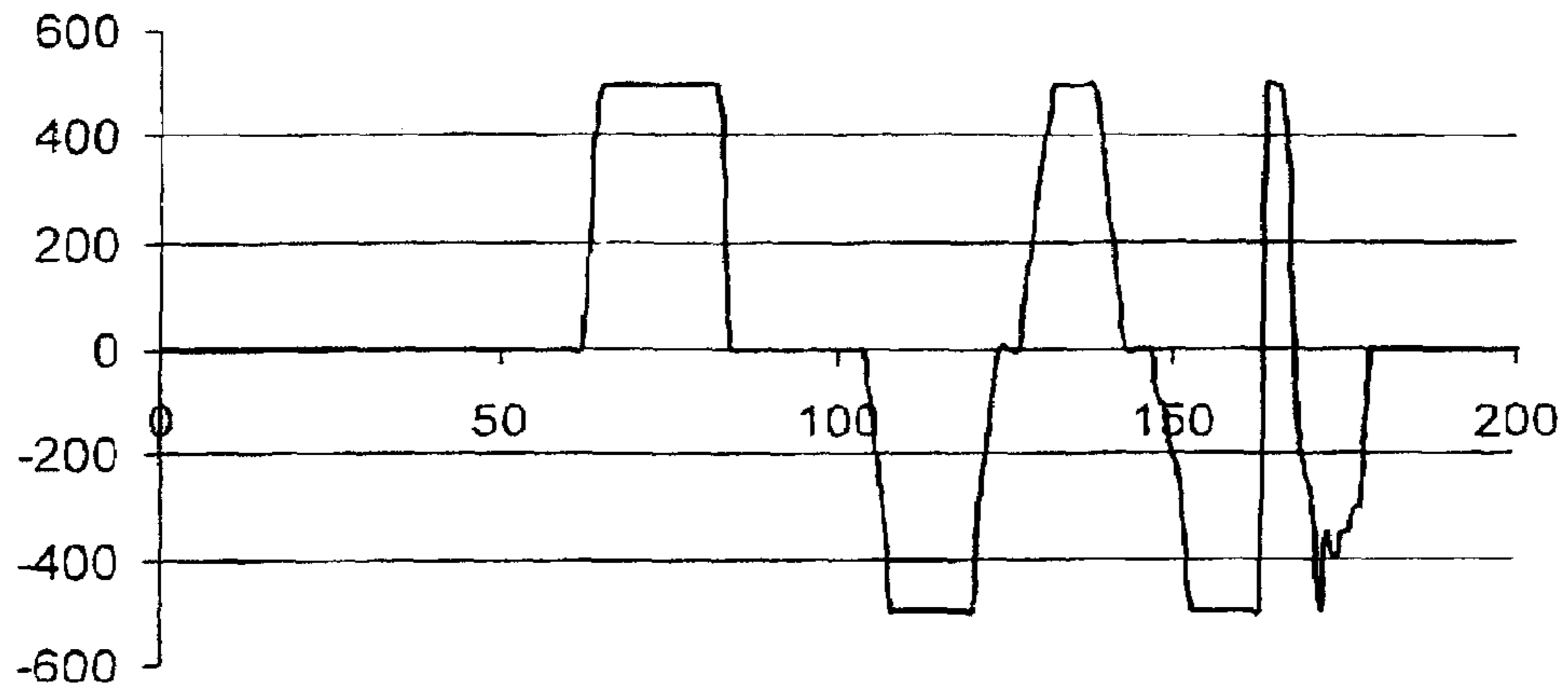
FIG. 8C charge power
