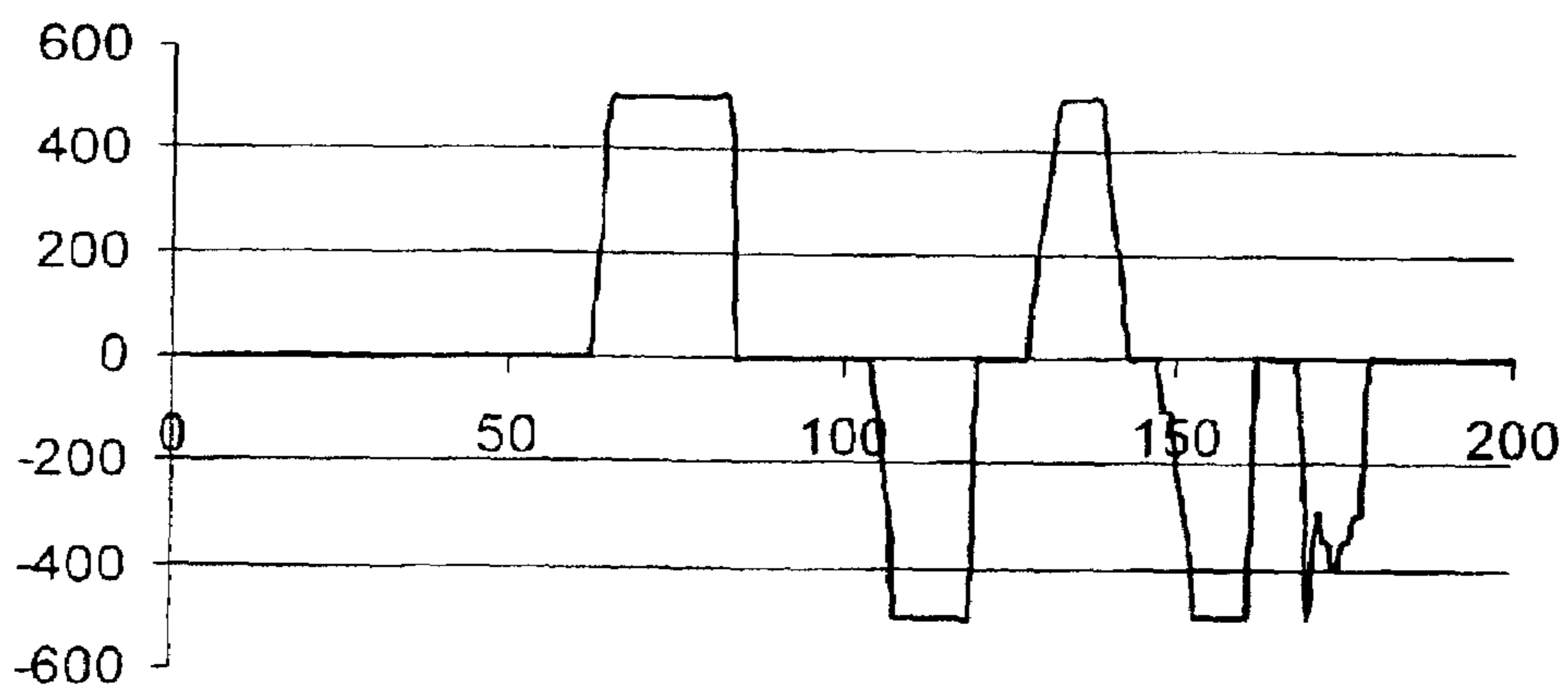
FIG. 7C charge power
