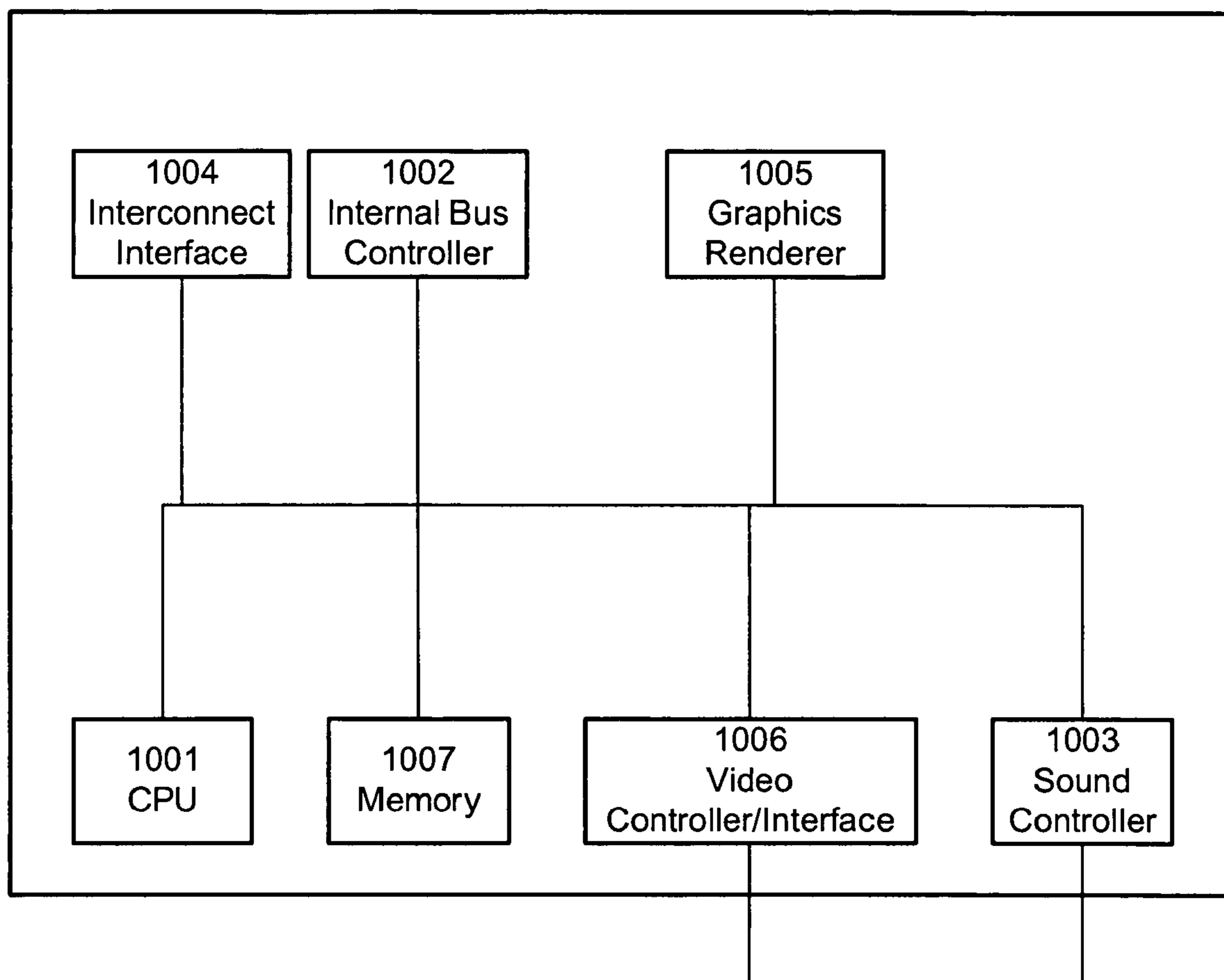
FIG. 10: HID Single Chip Implementation
