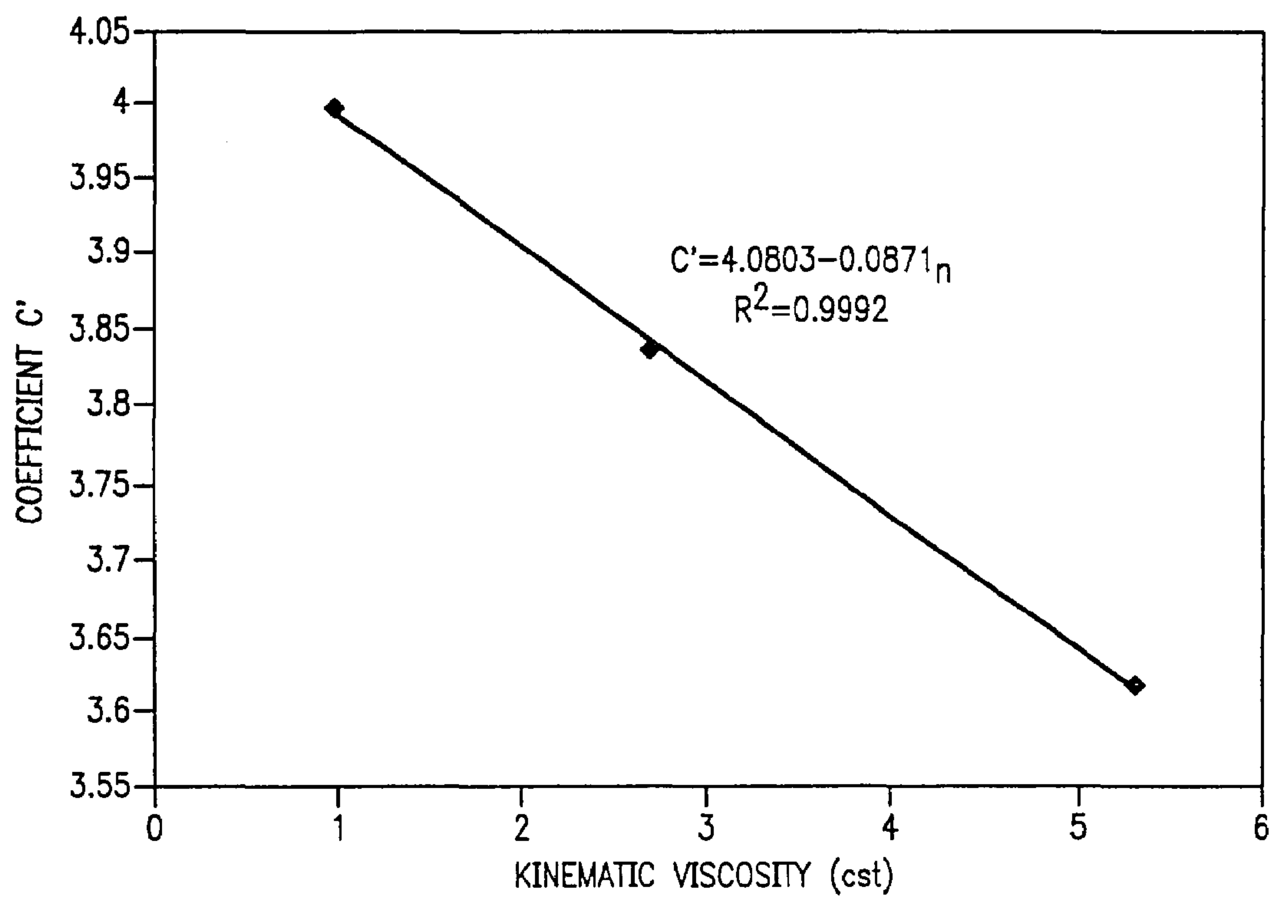
CALIBRATION CURVE COEFFICIENT C' vs KINEMATIC VISCOSITY FOR FLUTE 6UVT2 (1/4")
