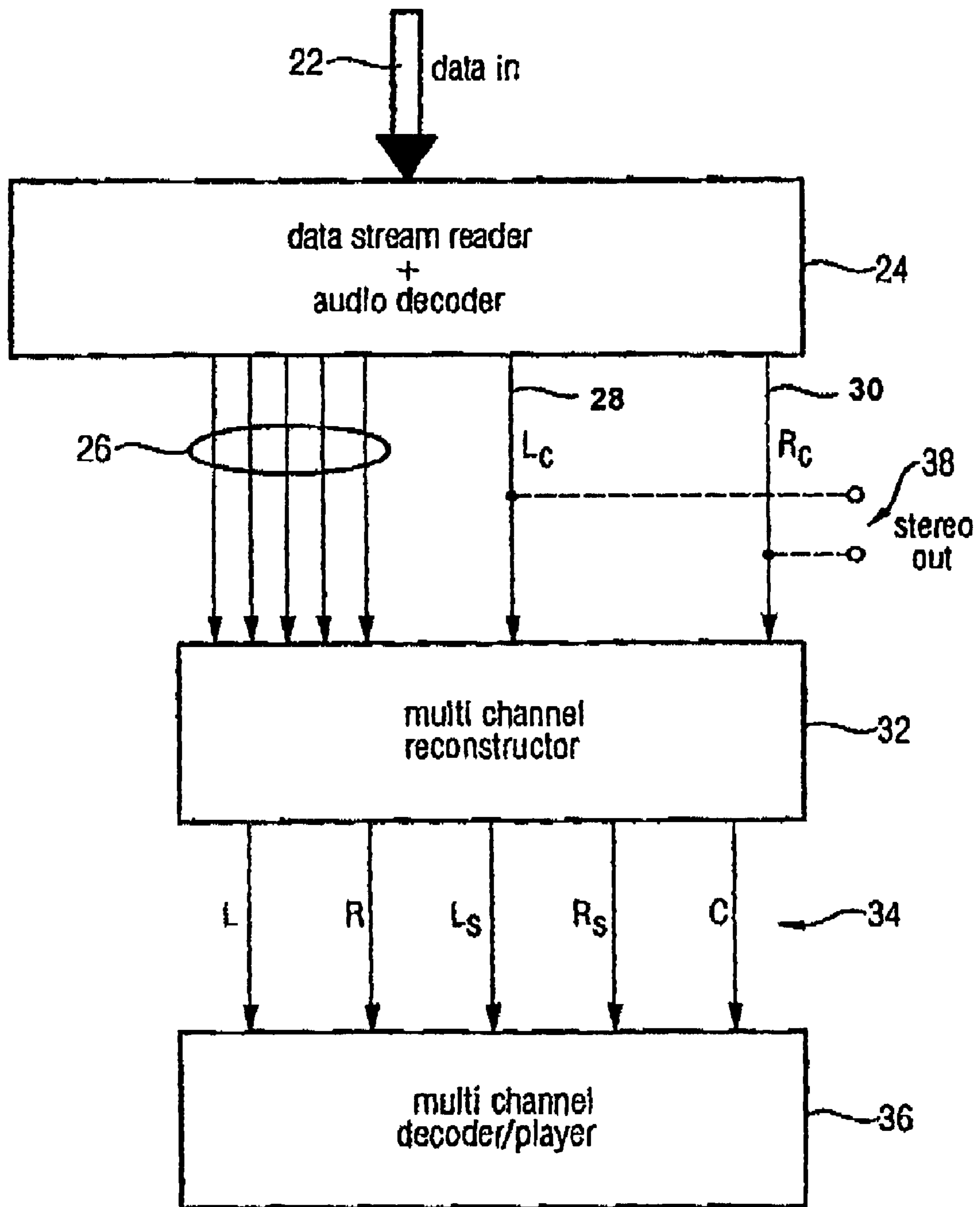
FIG 2 (Decoder)
