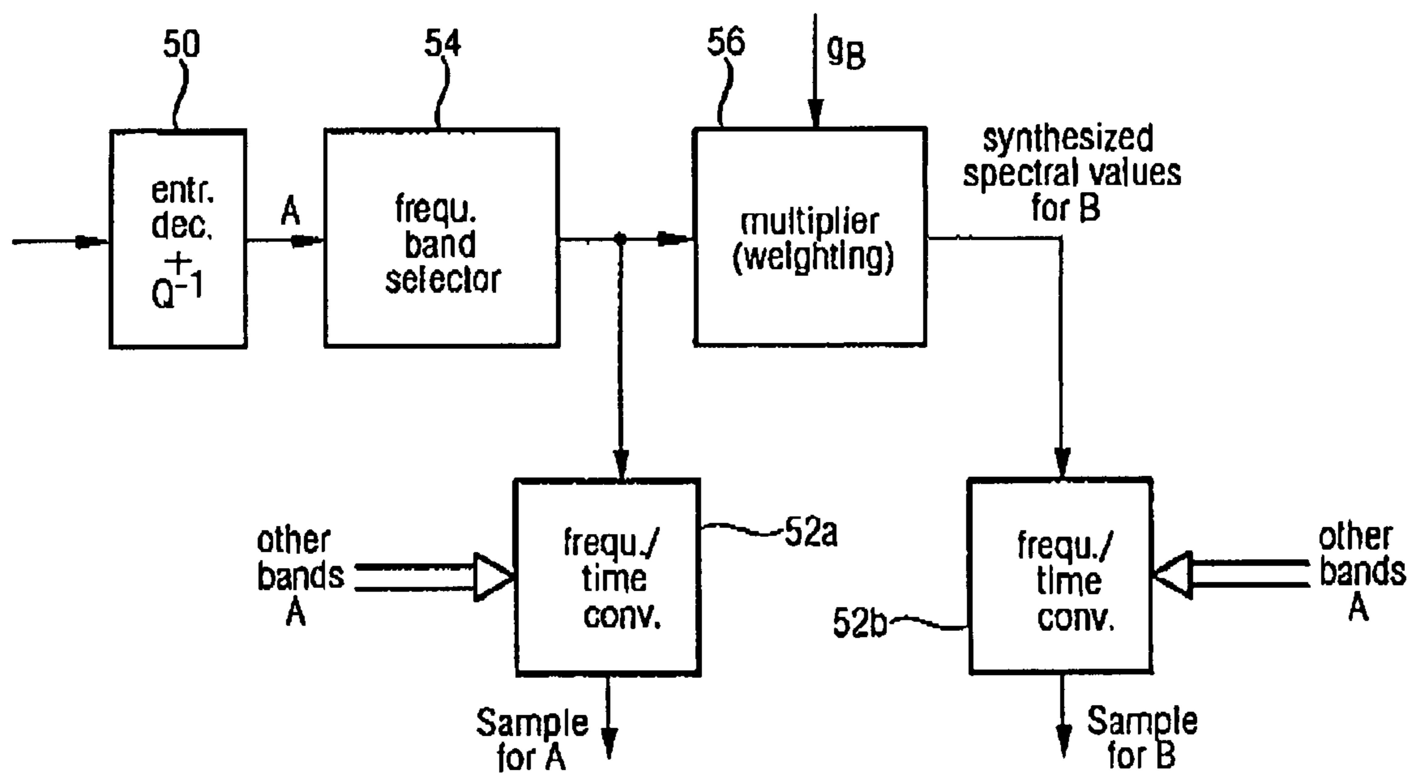
FIG 5 (decoder side)
