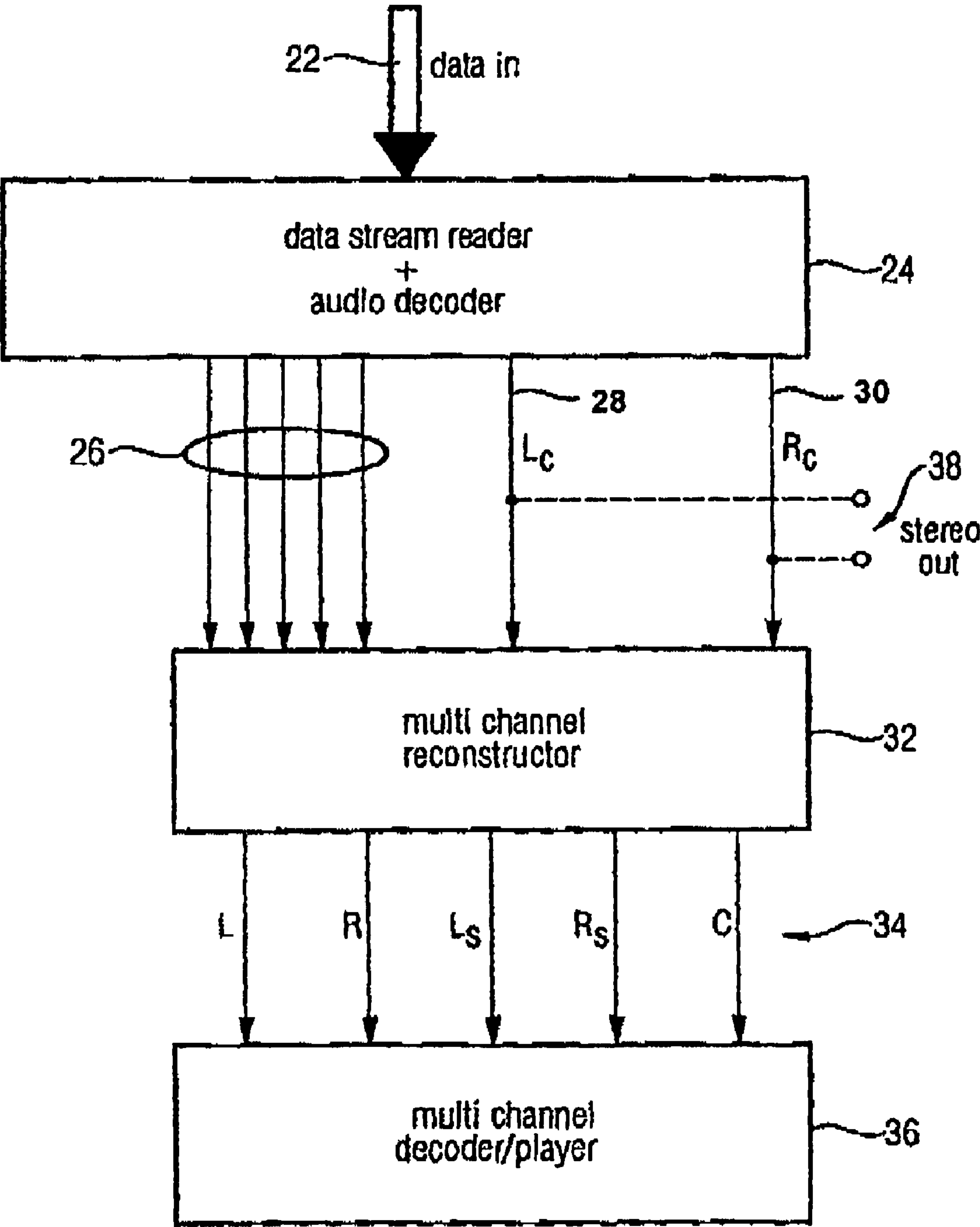
FIG 2 (Decoder)
