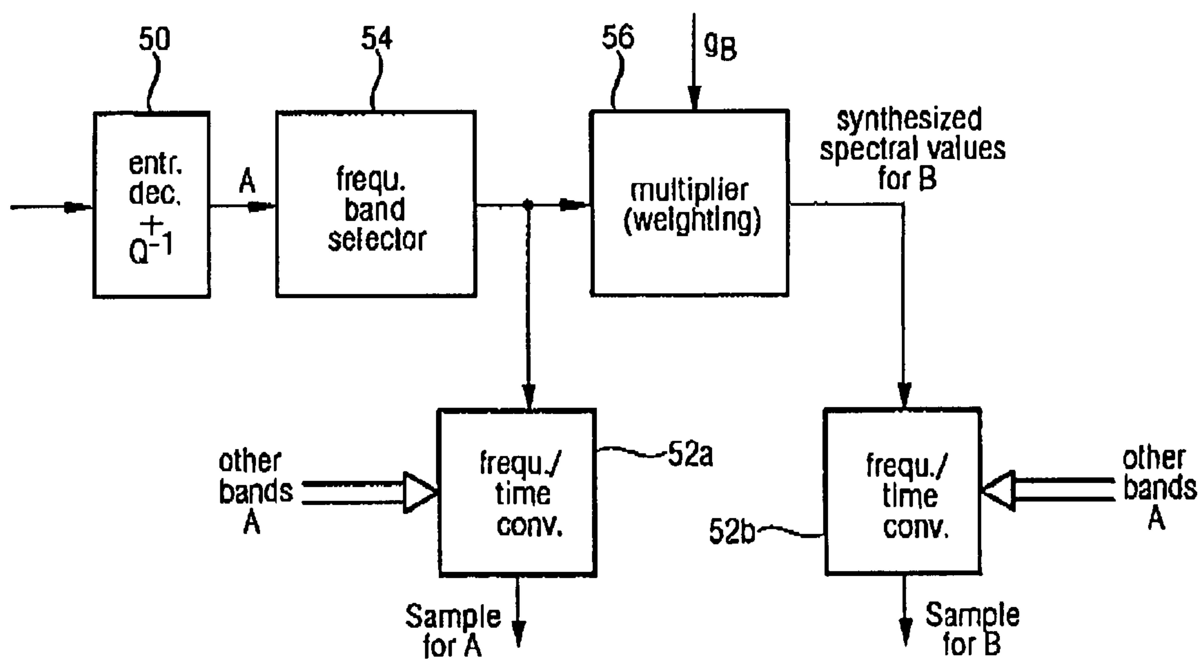
FIG 5 (decoder side)
