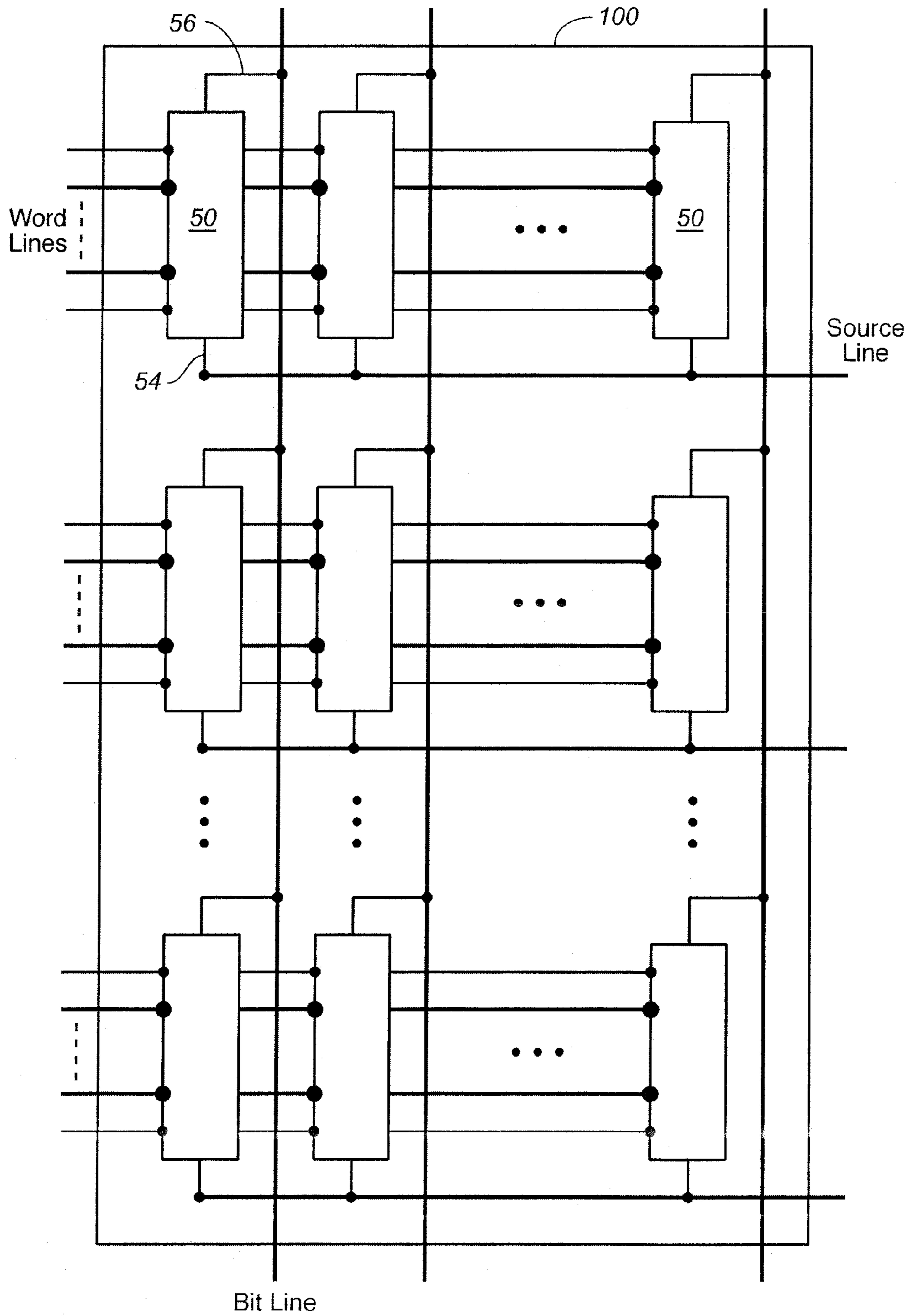
FIG. 3 (PRIOR ART)
