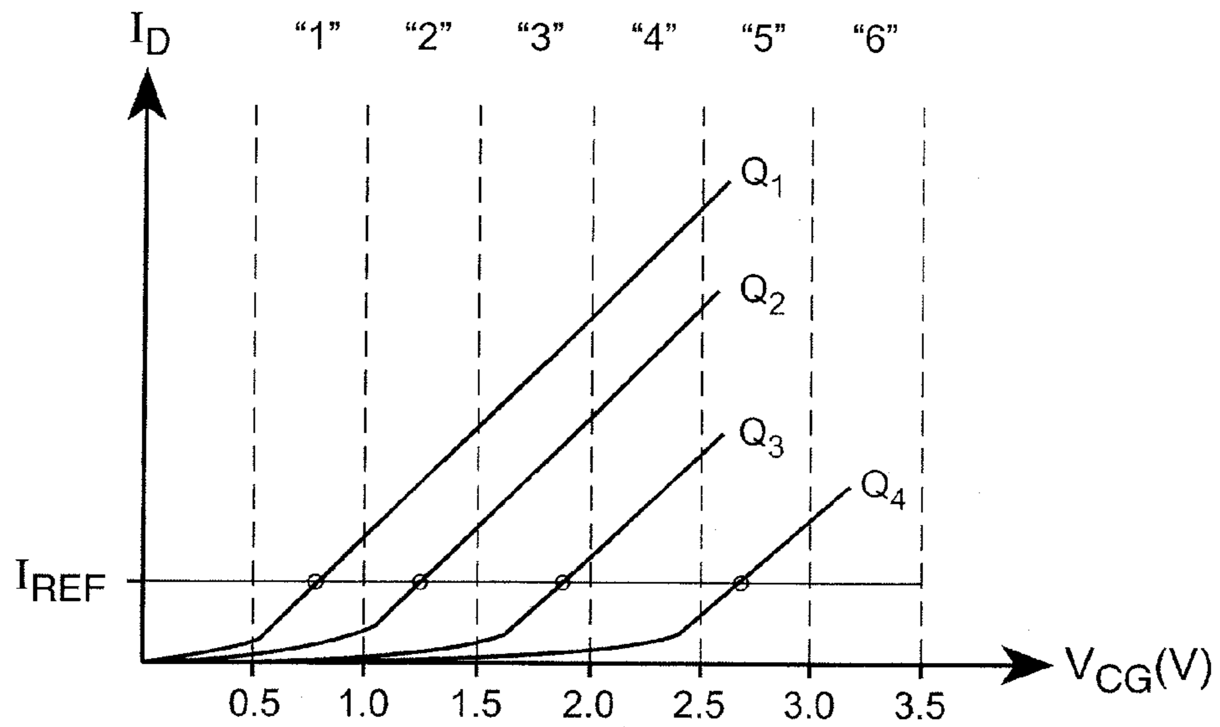
FIG. 4 (PRIOR ART)
