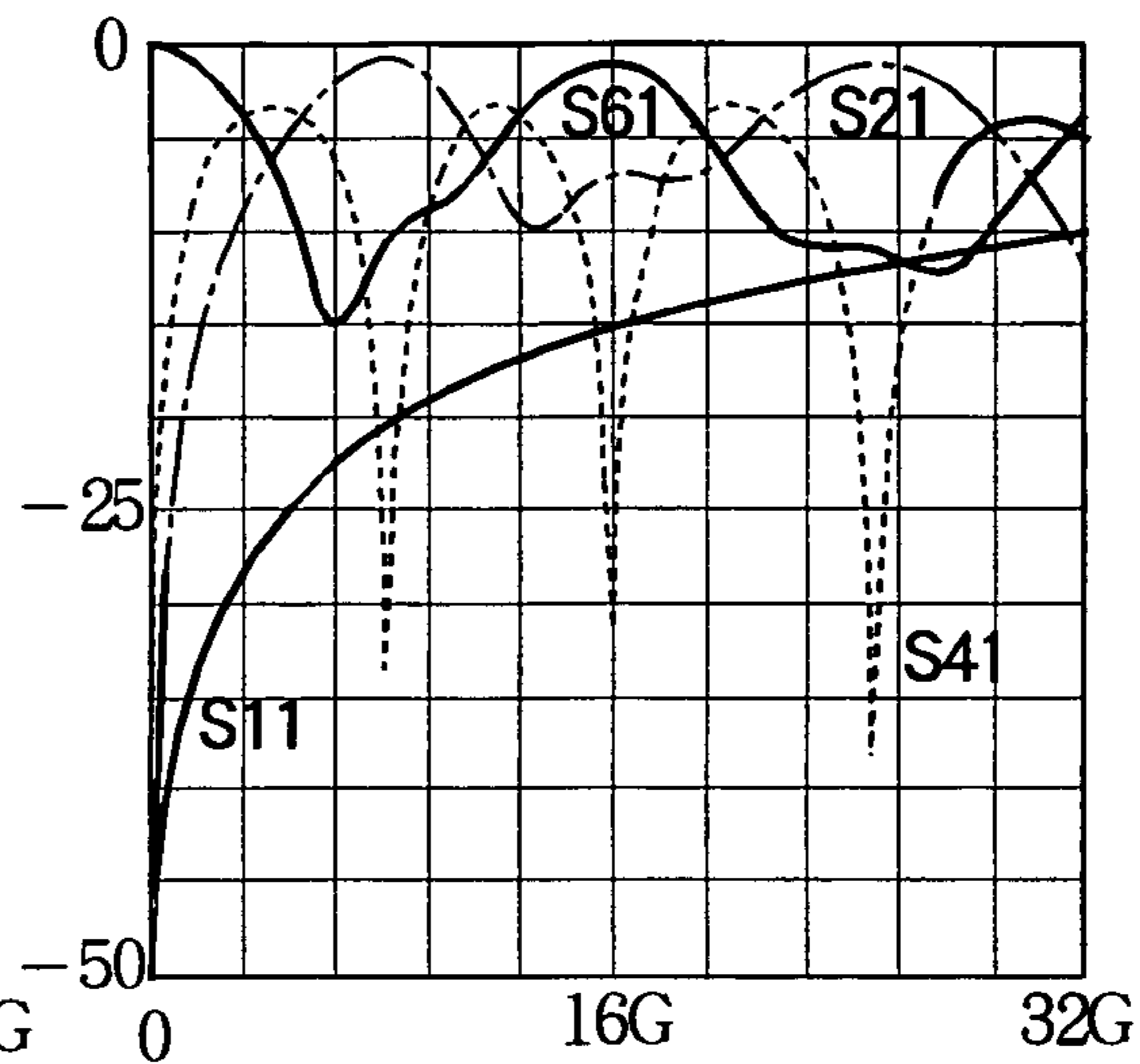
SINEWAVE FREQUENCY (Hz) L/S=1/0.5
