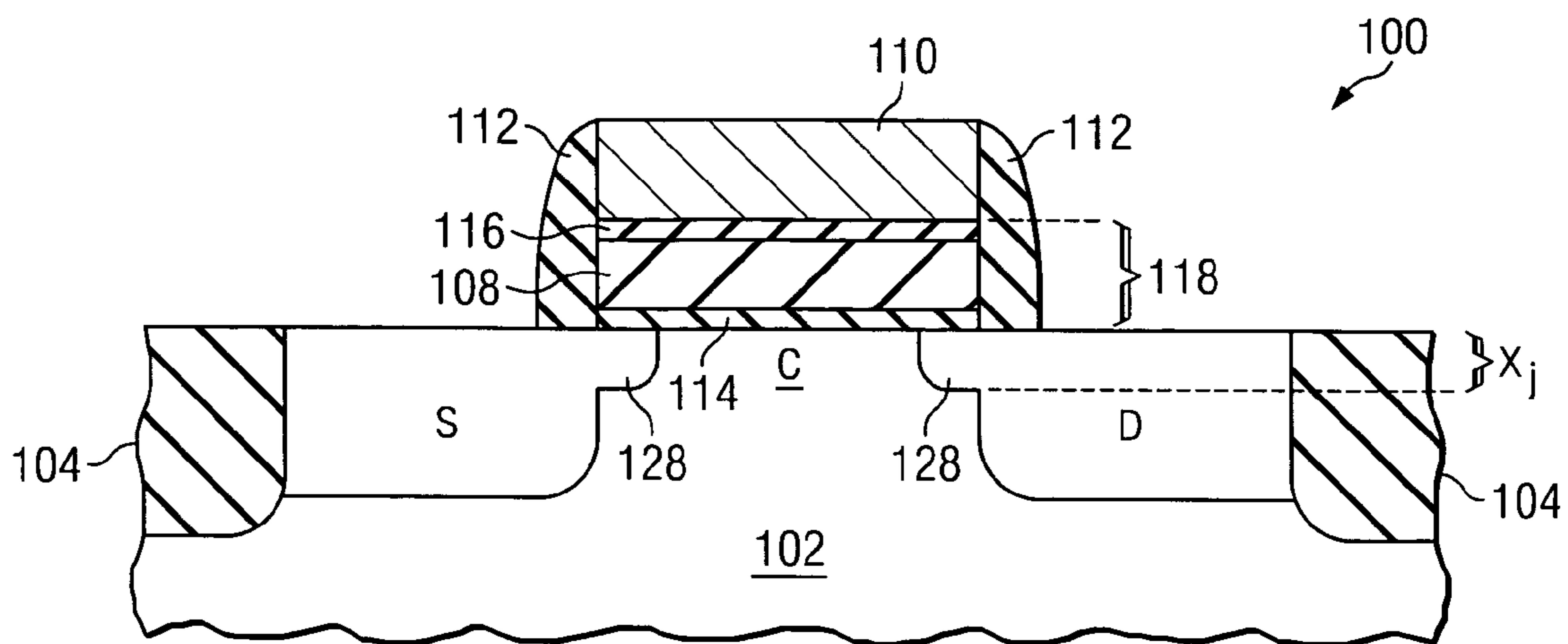
FIG. 1 (PRIOR ART)
