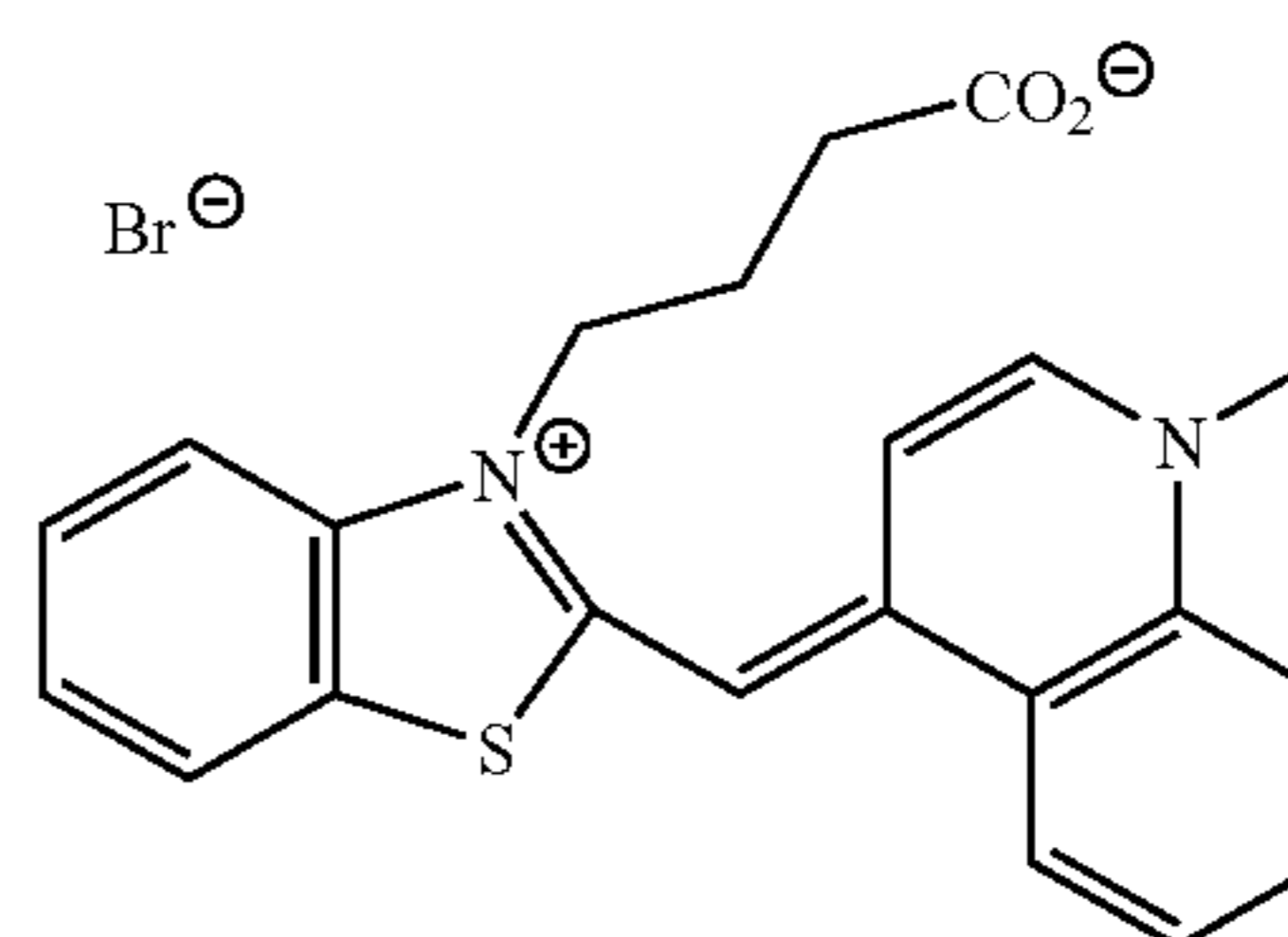
Example 19
