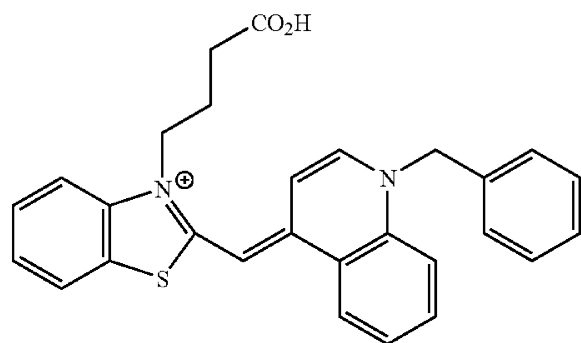
Compound 33
