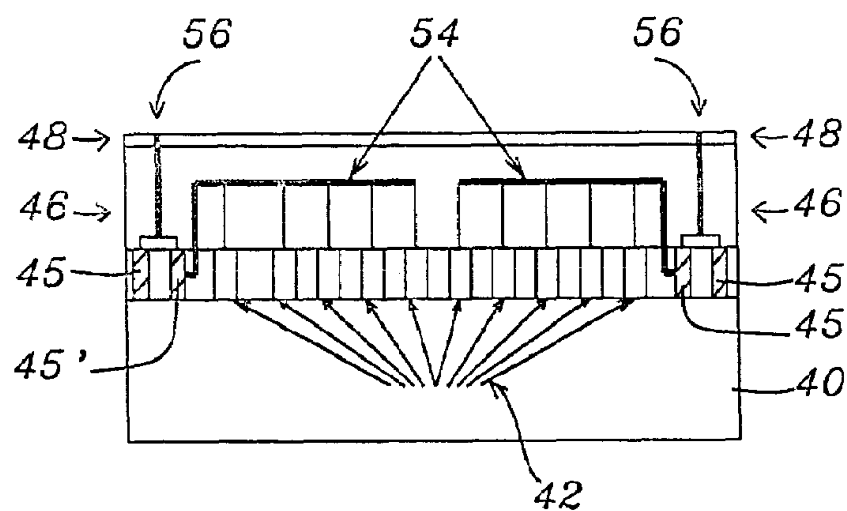
FIG. 2 - Prior Art
