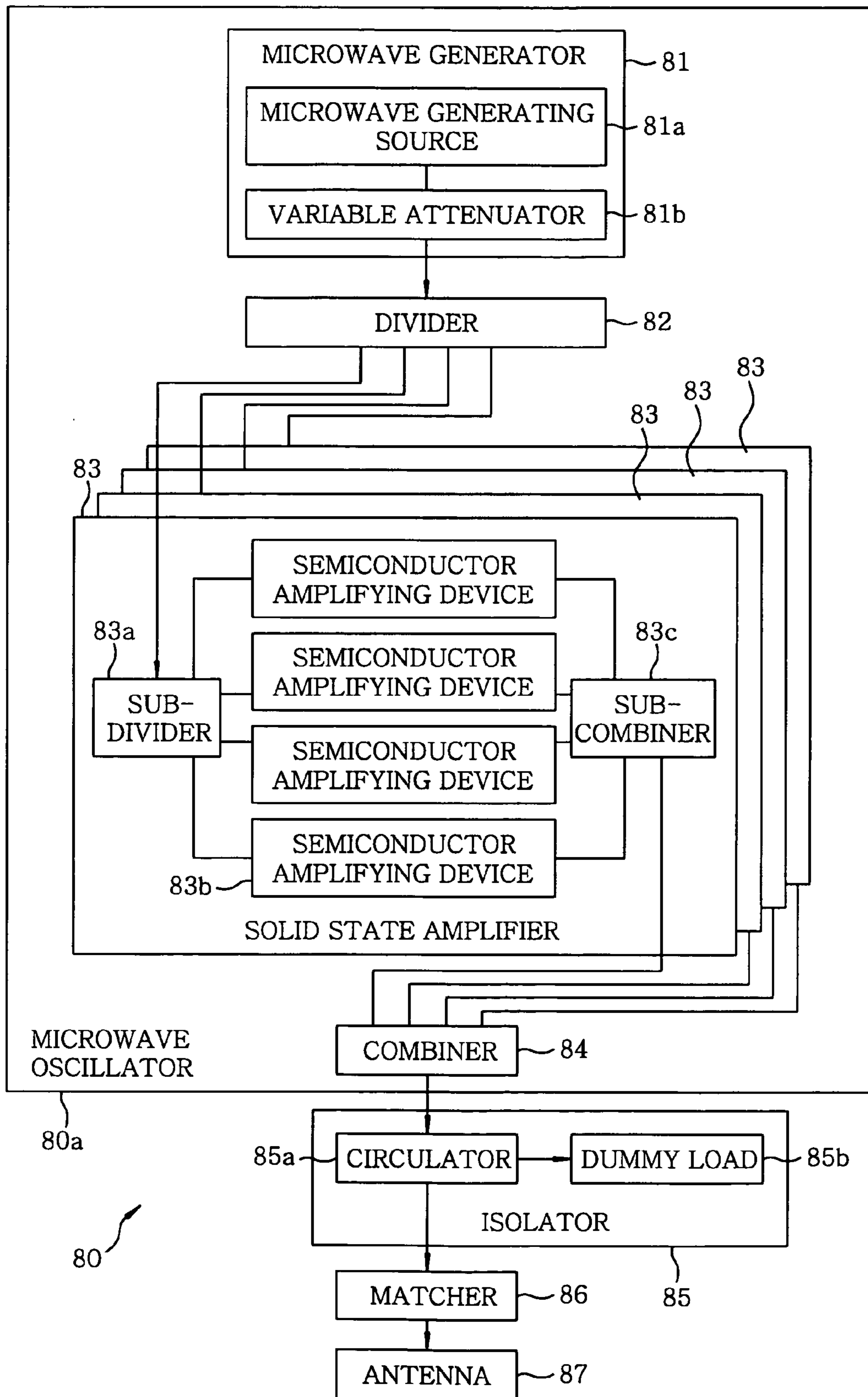
FIG. 7 (PRIOR ART)
