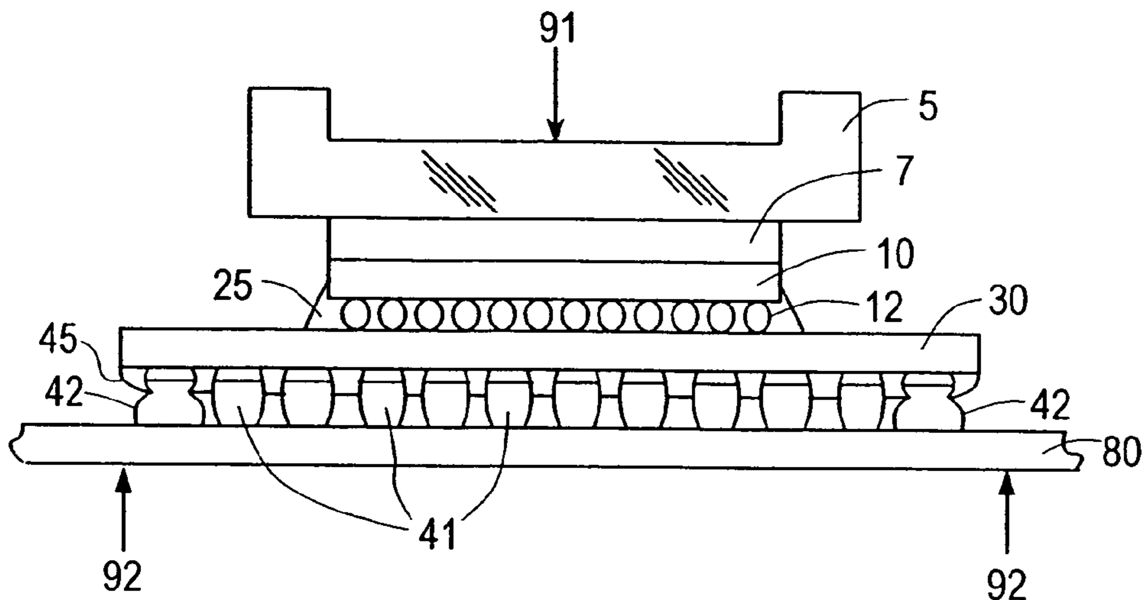
Fig. 1C PRIOR ART
