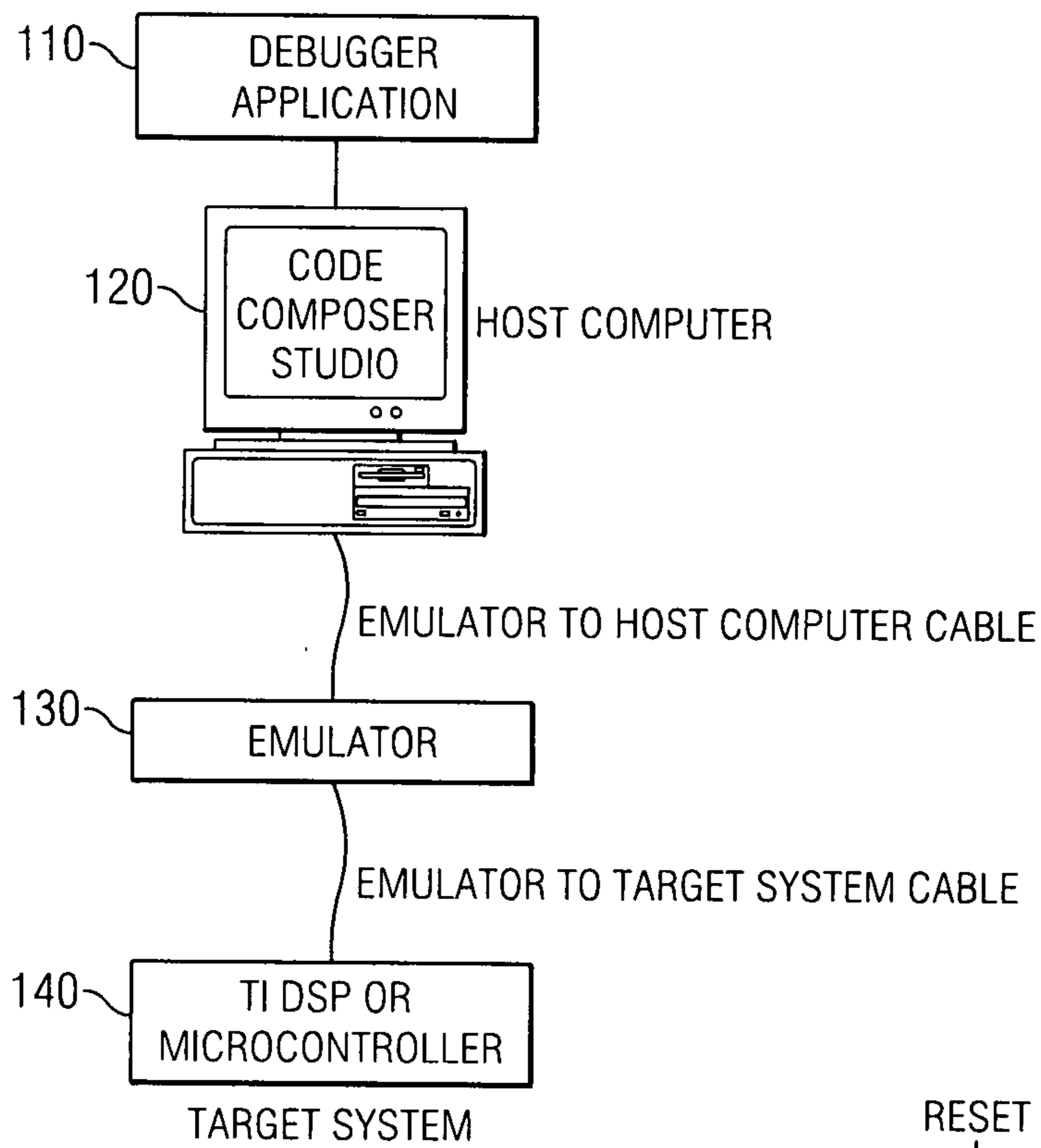
FIG. 2 (PRIOR ART)
