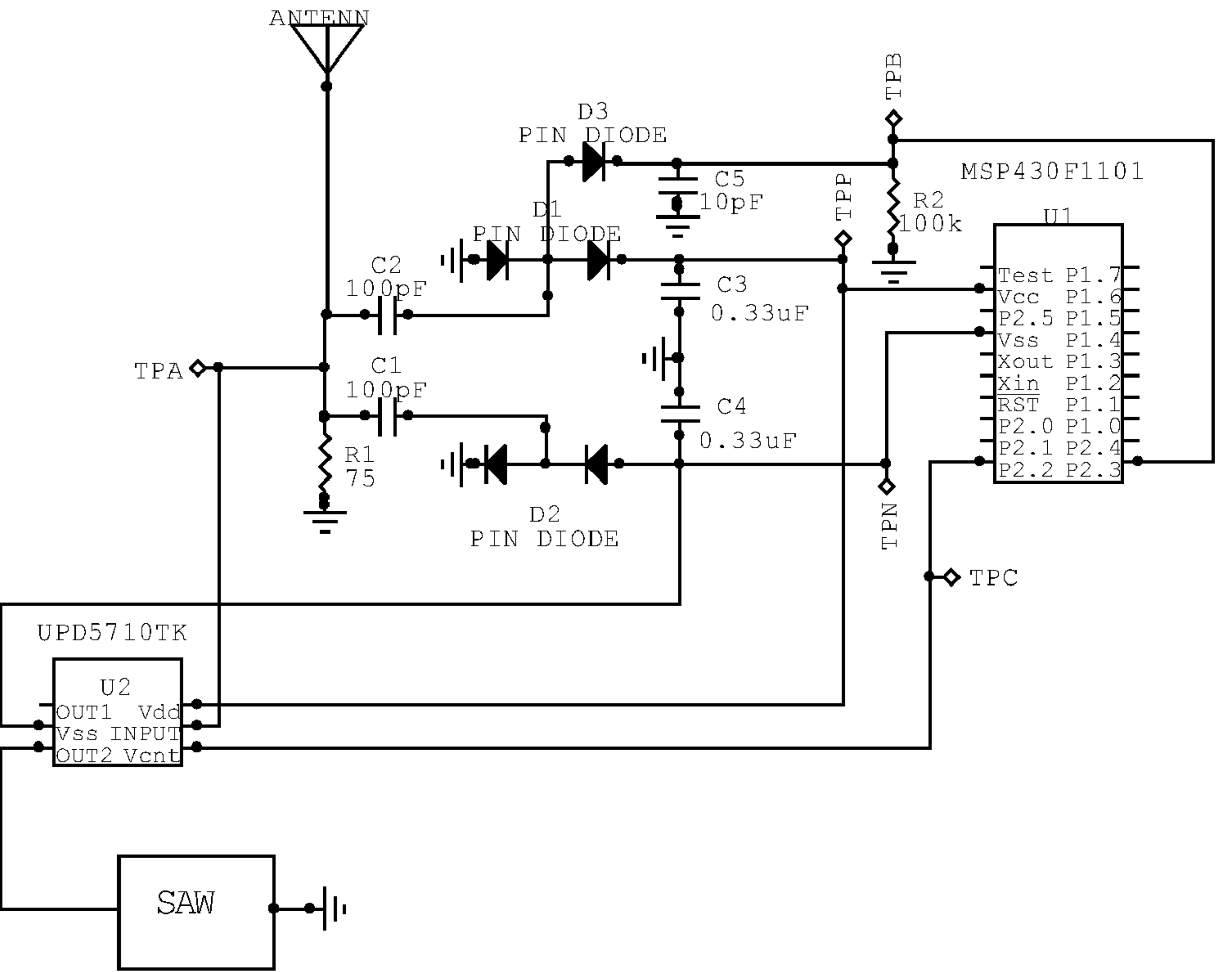
Transponder for TPM uVall
