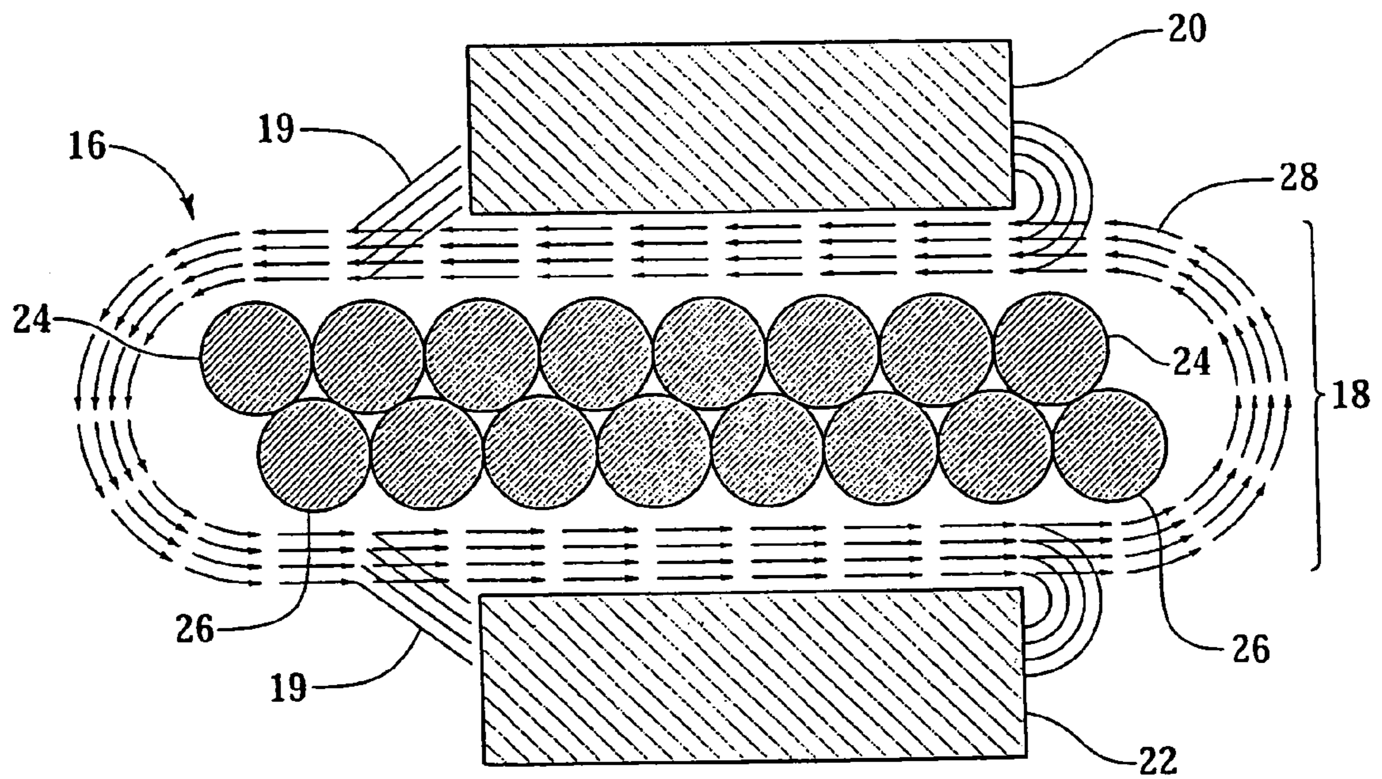
Fig. 2 (PRIOR ART)
