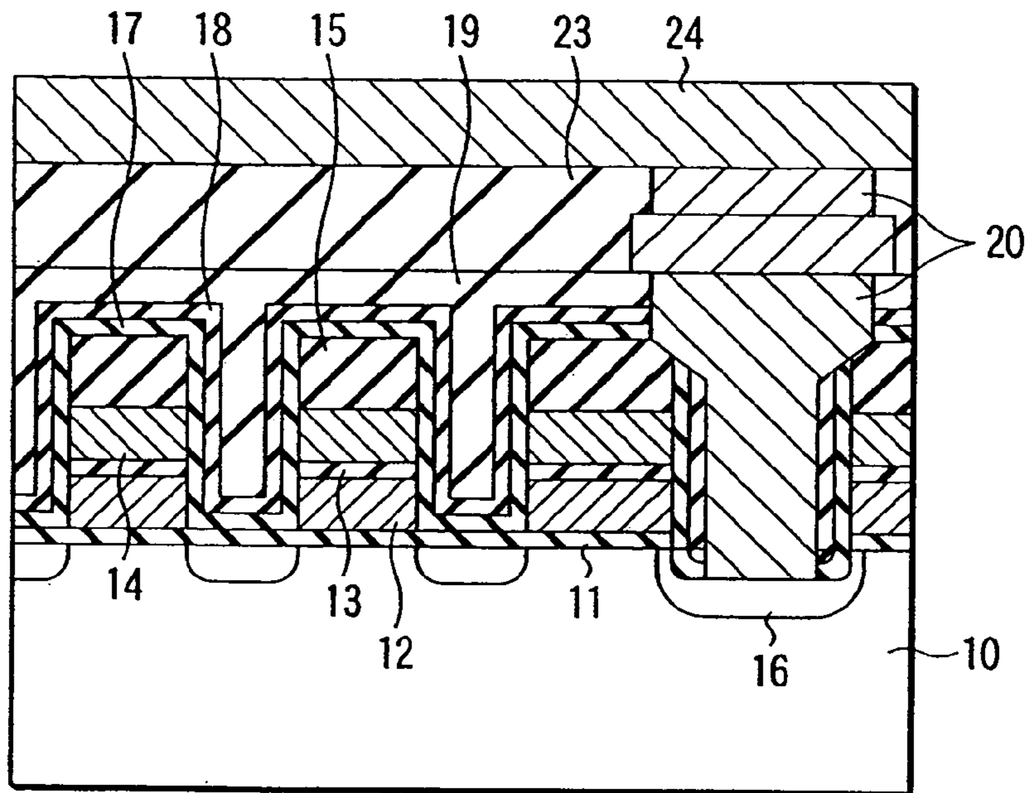
Memory cell array
