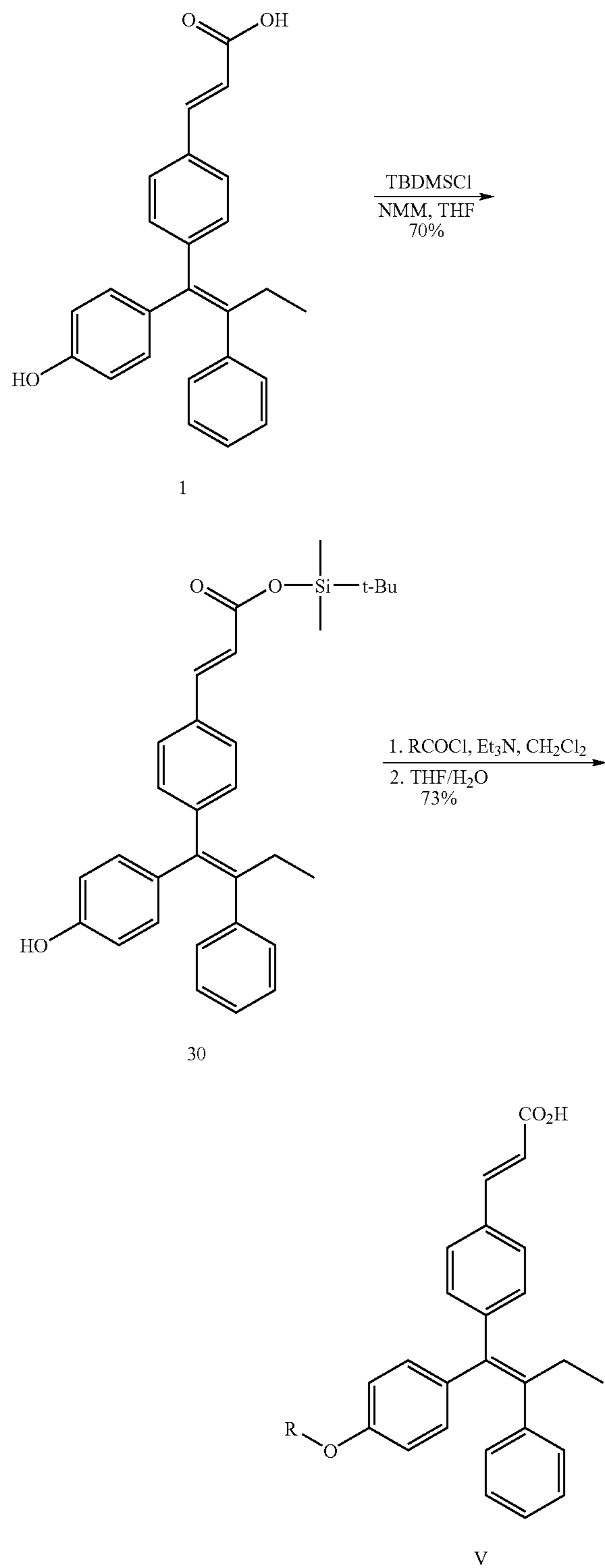
Scheme 5. Preparation of Ester Prodrugs of Compound 1 - Method D
