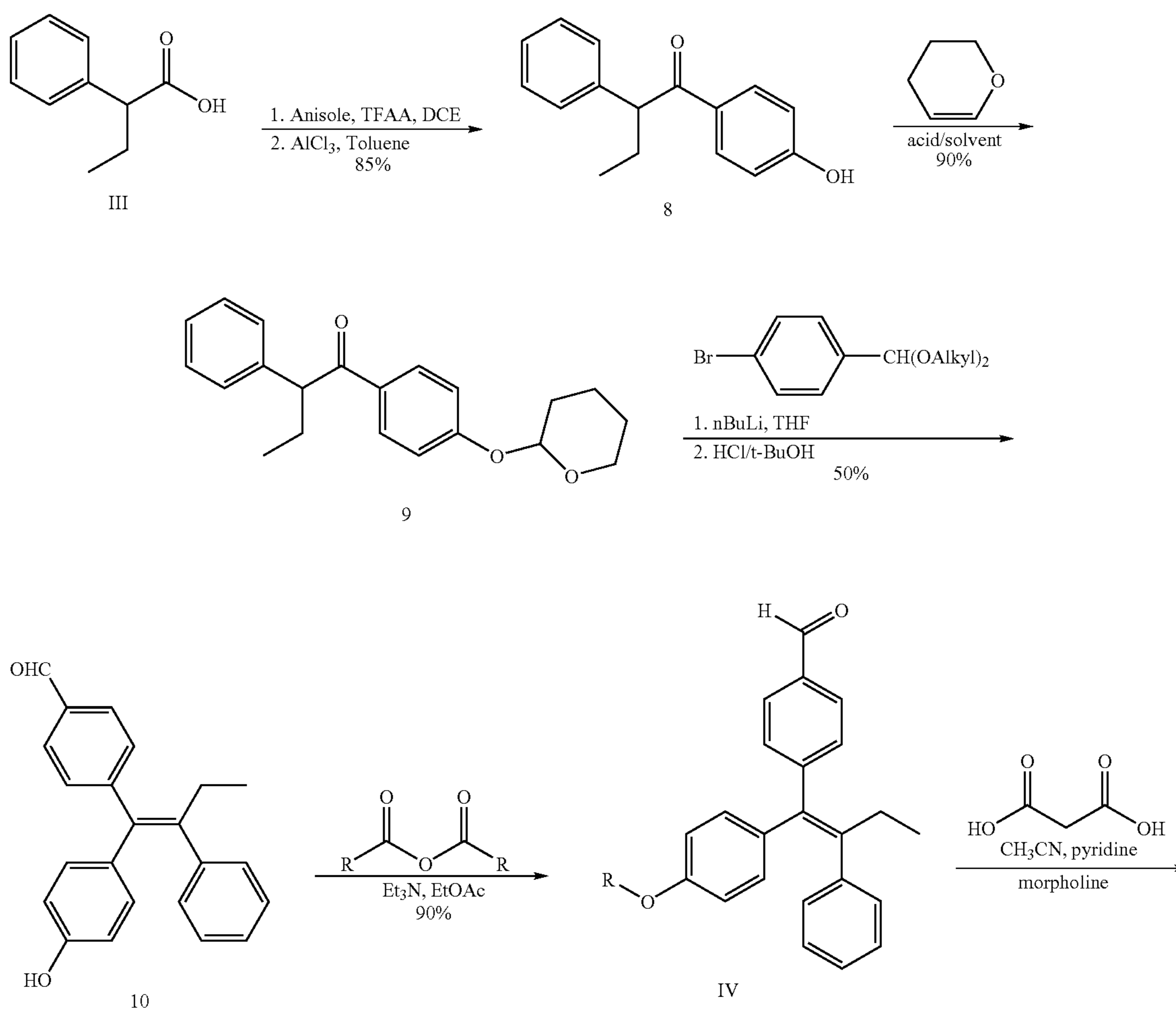
Scheme 2. Preparation of Ester Prodrugs of Compound 1 - Method A
