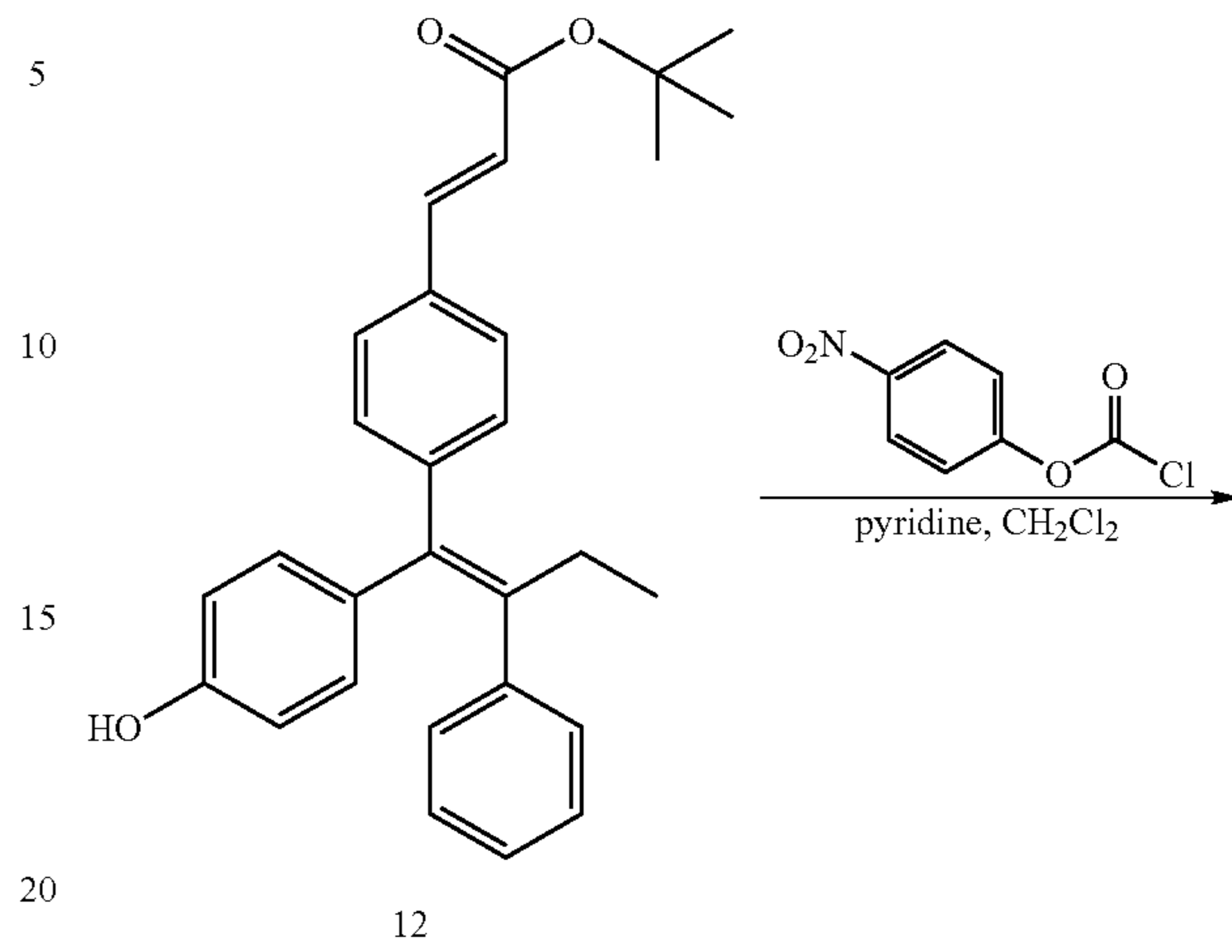
Scheme 8. Preparation of Carbonate Prodrugs of Compound 1 (Method A)
