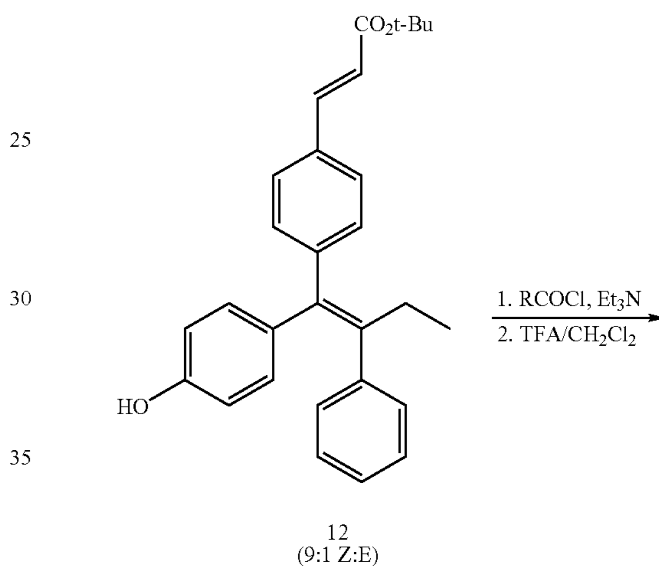
Scheme 4. Preparation of Ester Prodrugs of Compound 1 - Method C
