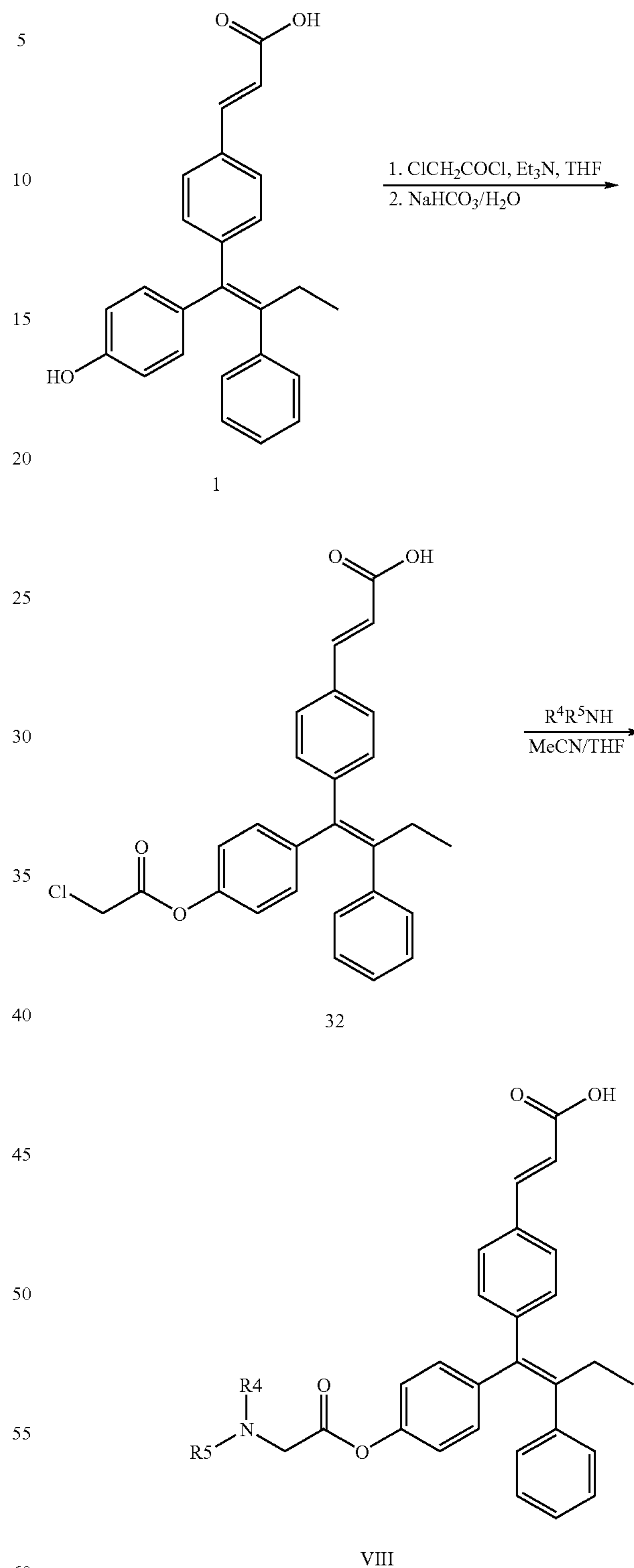
Scheme 6. Preparation of Substituted Glycine Ester Prodrugs
