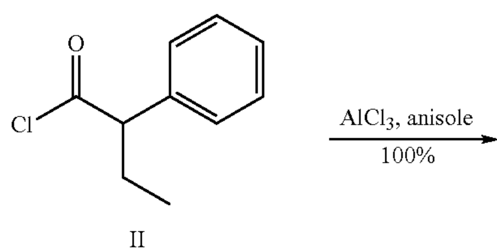
Scheme 1. Preparation of Compound 1
