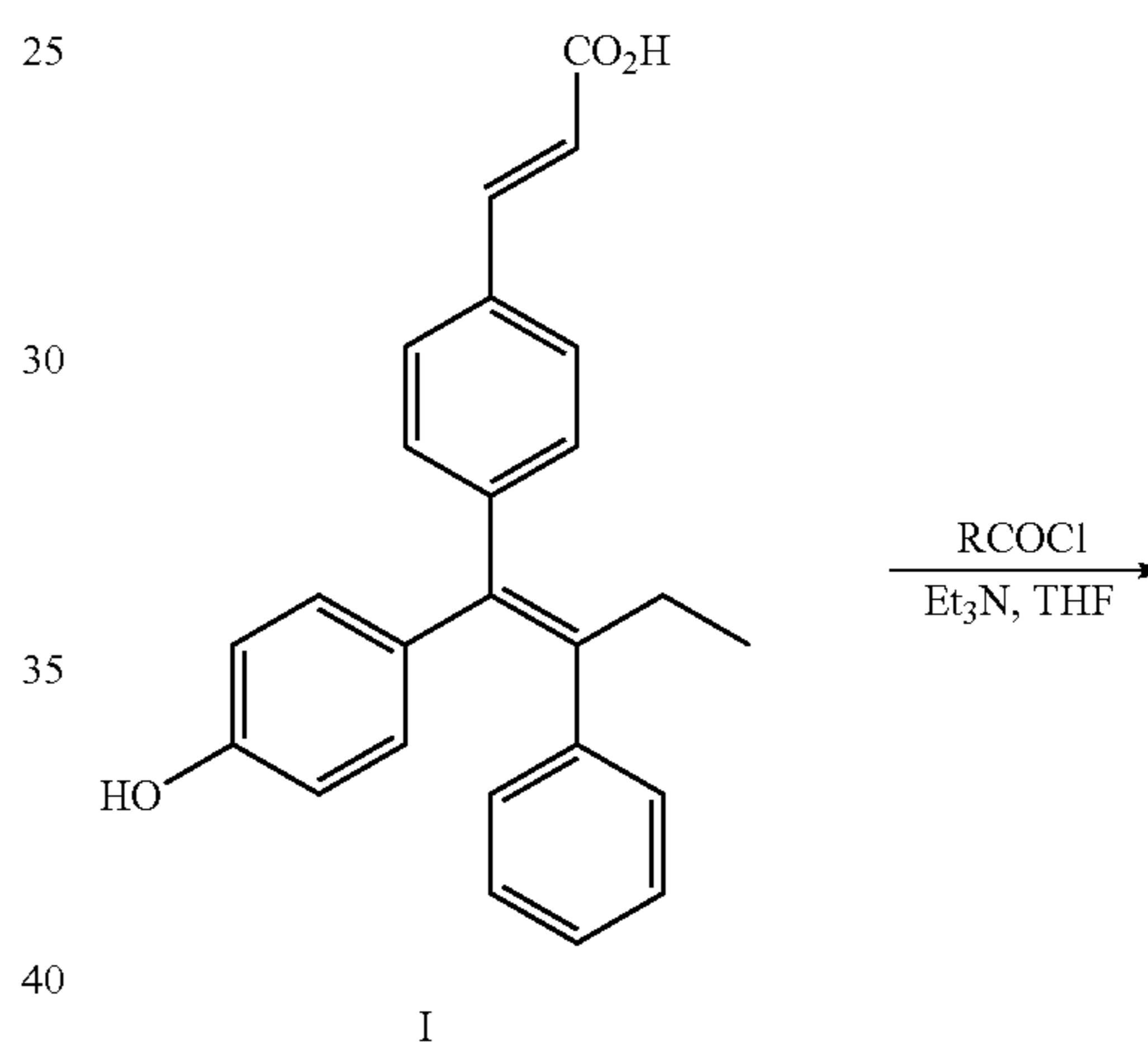
Scheme 3. Preparation of Ester Prodrugs of Compound 1 - Method B
