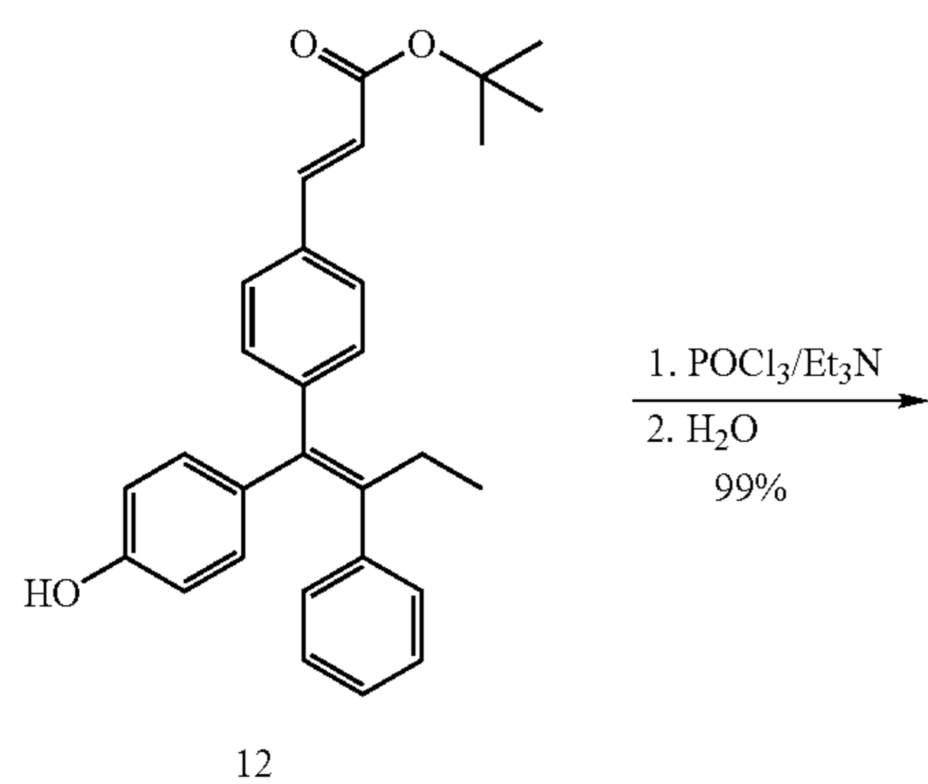
Scheme 7. Preparation of a Phosphate Prodrug of Compound 1
