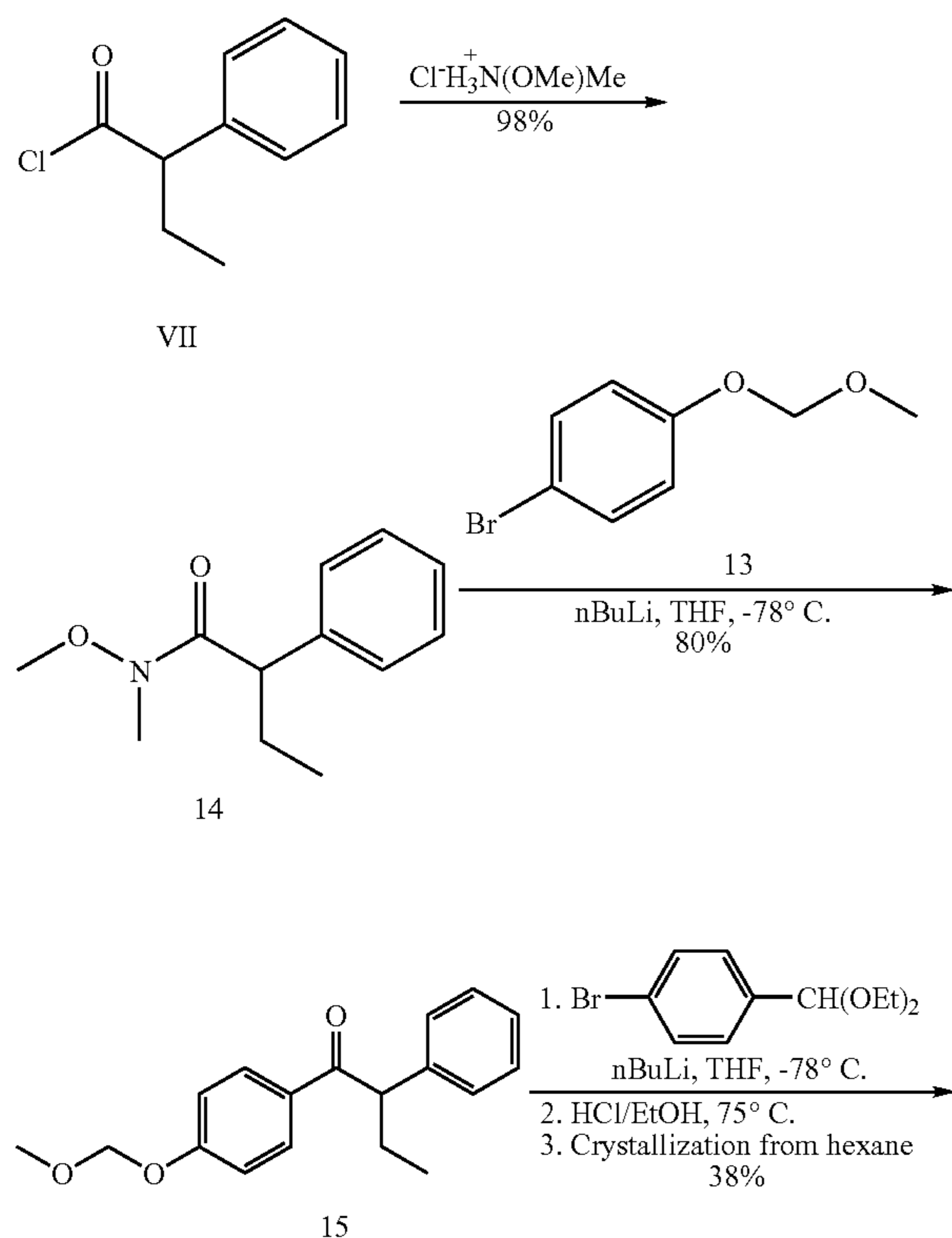
Scheme 4. Preparation of Ester Prodrugs of Compound 1 - Method C
