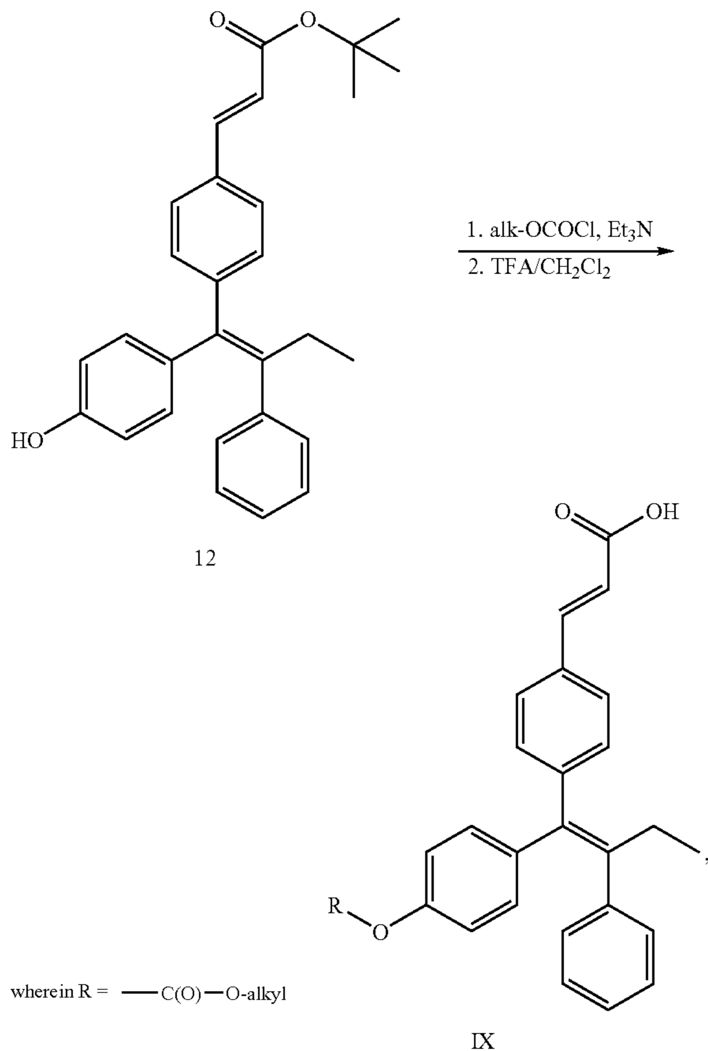
Scheme 9. Preparation of Carbonate Prodrugs of Compound 1 (Method B)
