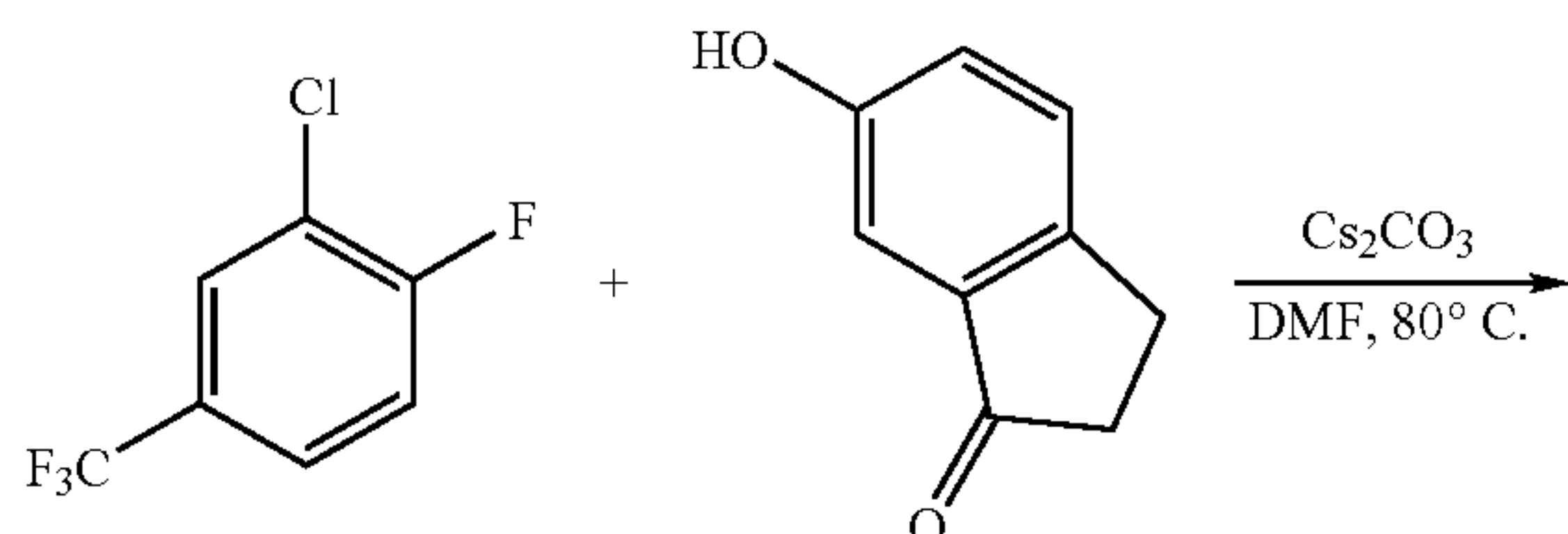
Scheme 8: Biaryl Indanones
