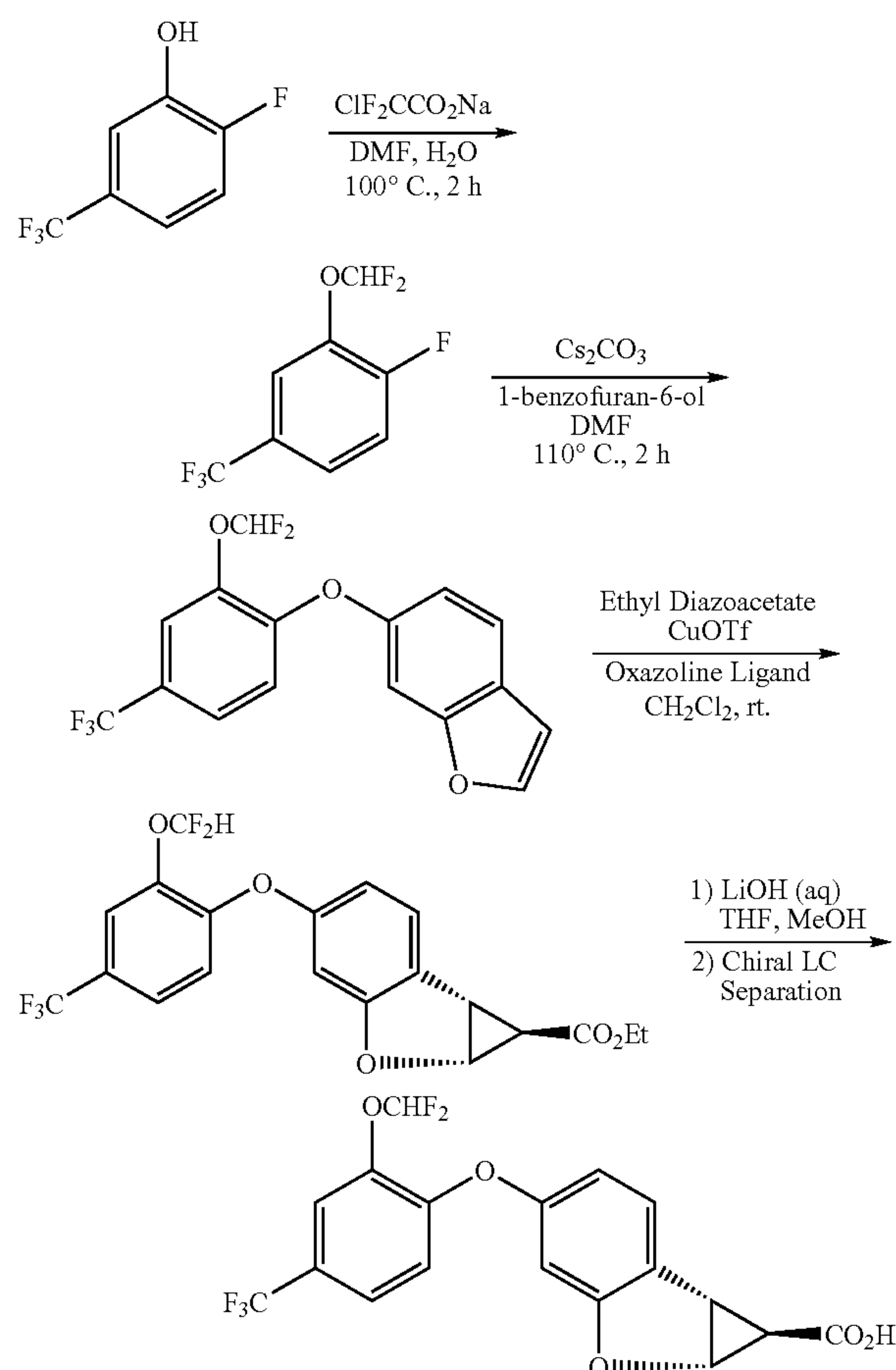
Scheme 3: Asymmetric Cyclopropanation
