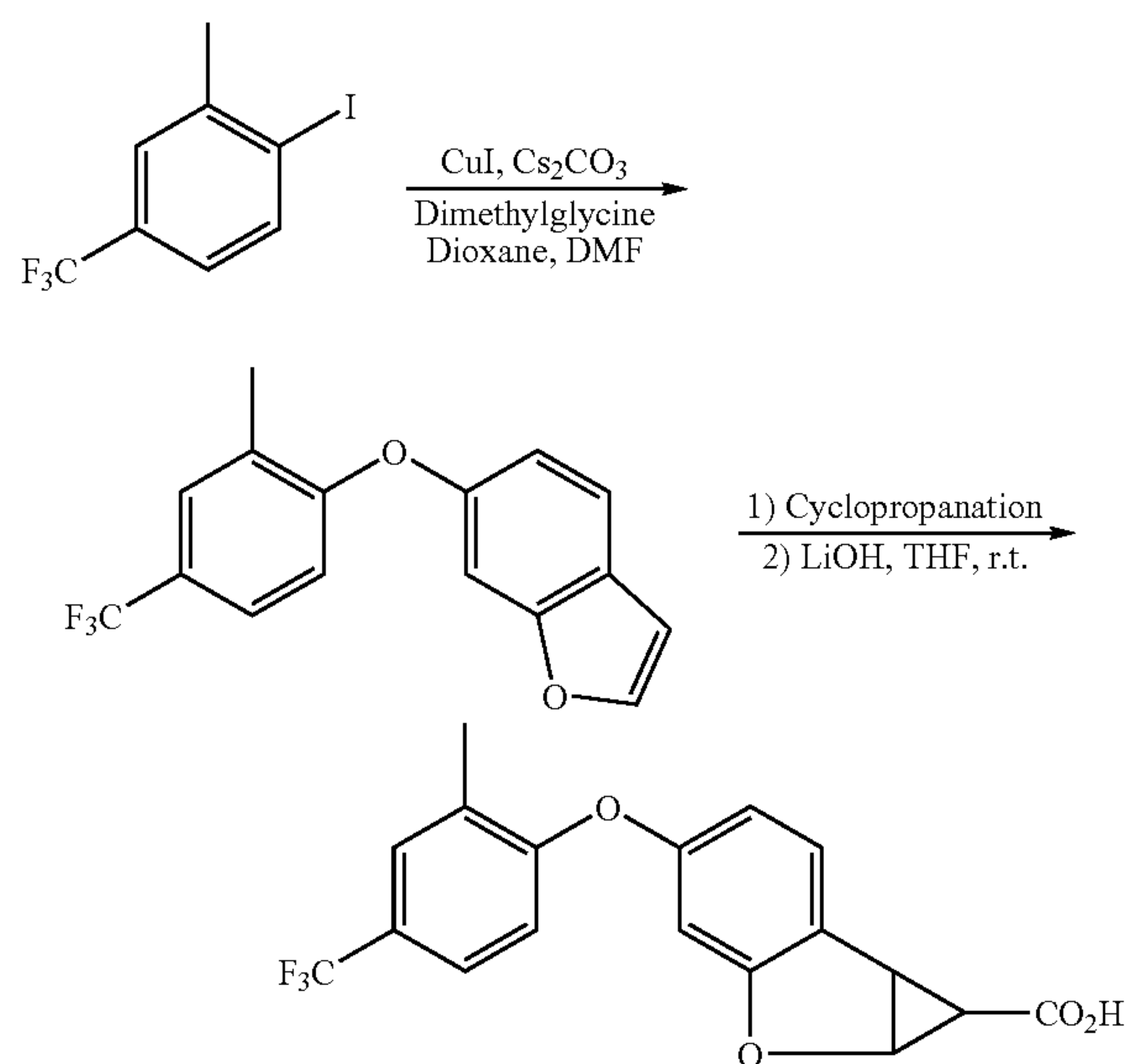
Scheme 2: Copper Coupling
