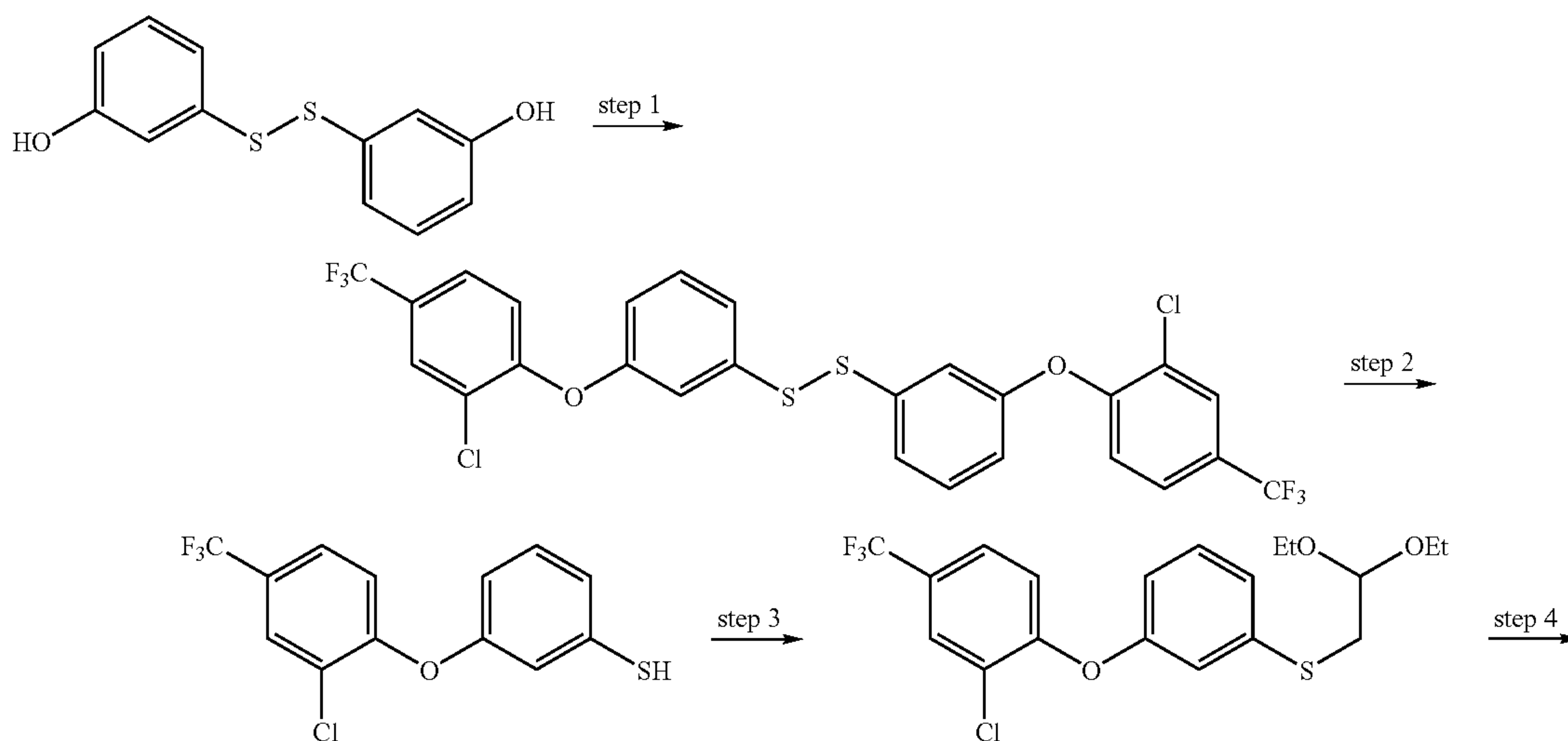
Scheme 10: Benzothiophene Derivatives
