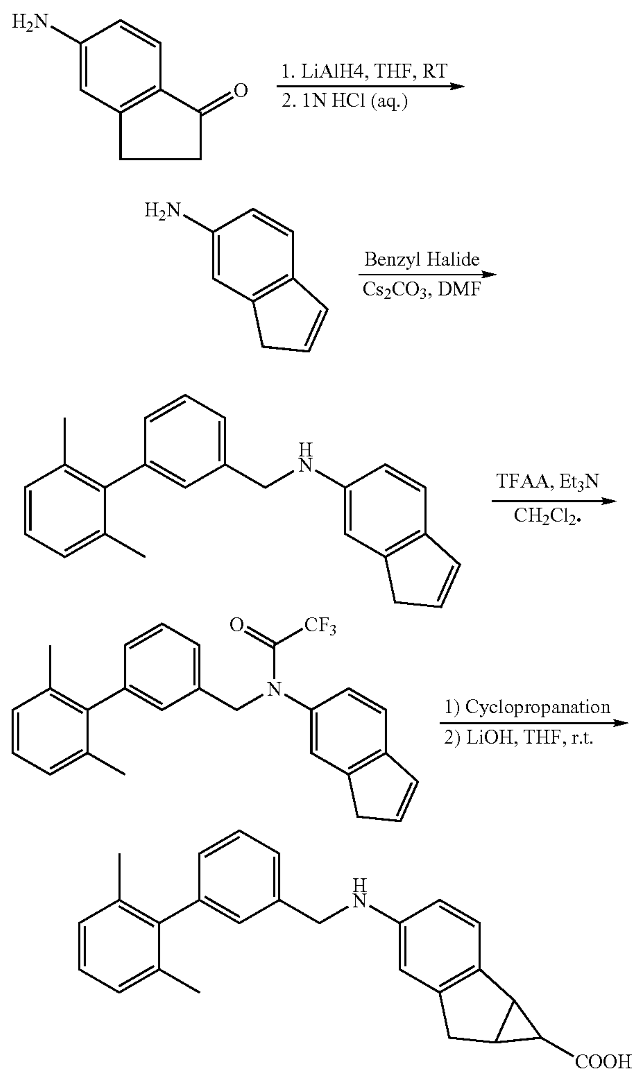
Scheme 9: Aminoindane Derivatives
