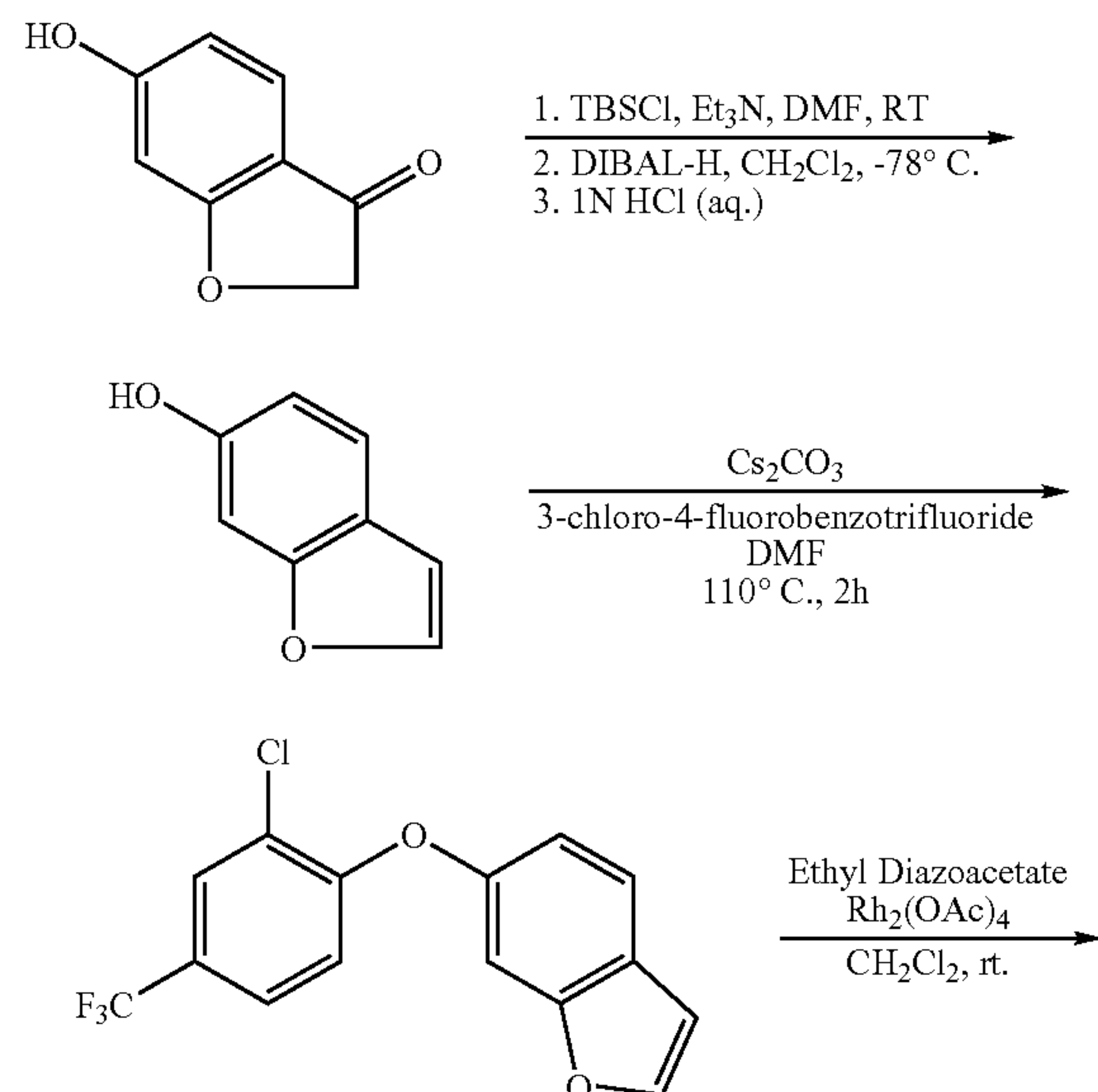
Scheme 1: Biaryl Ethers
