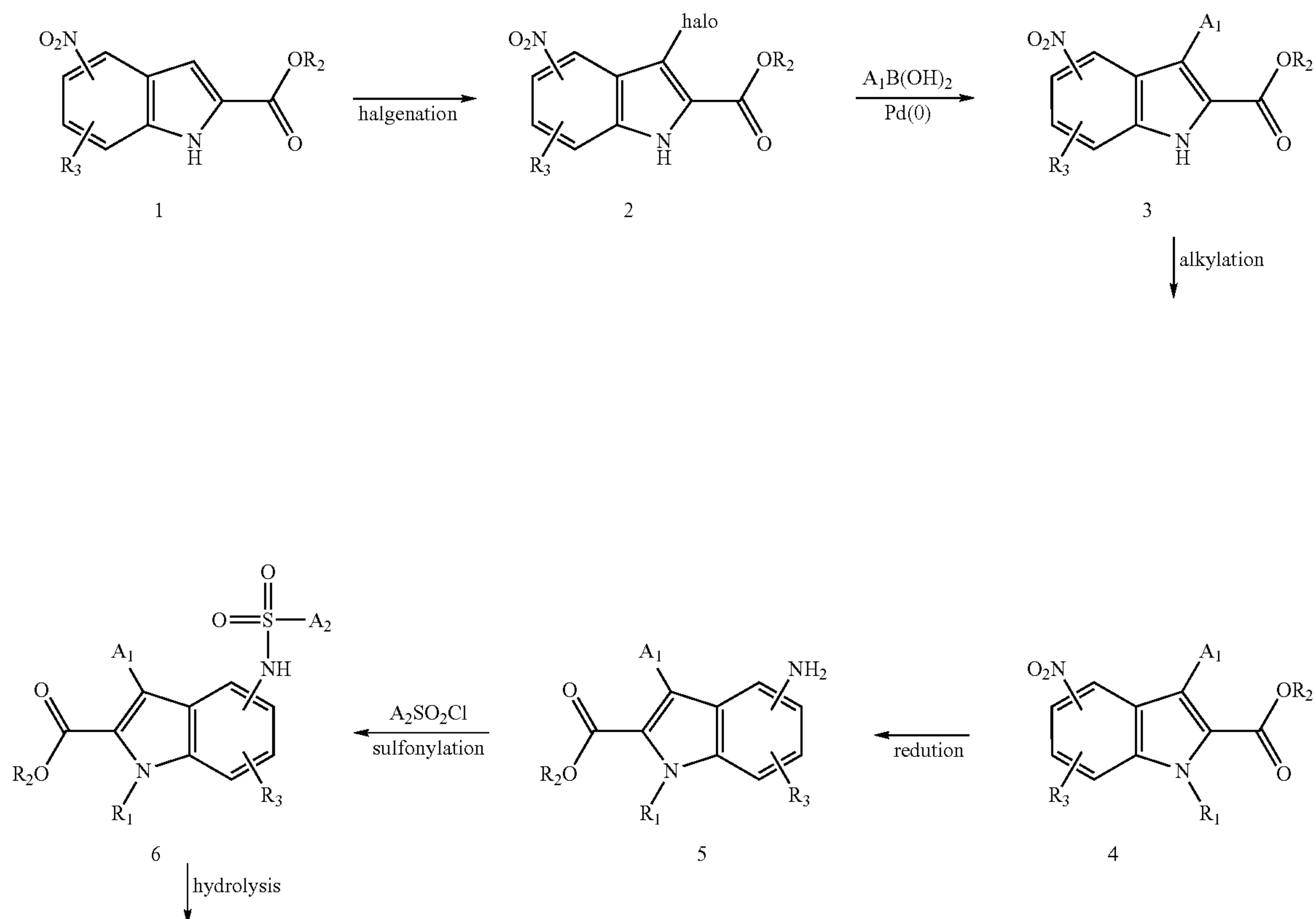
Scheme 1
