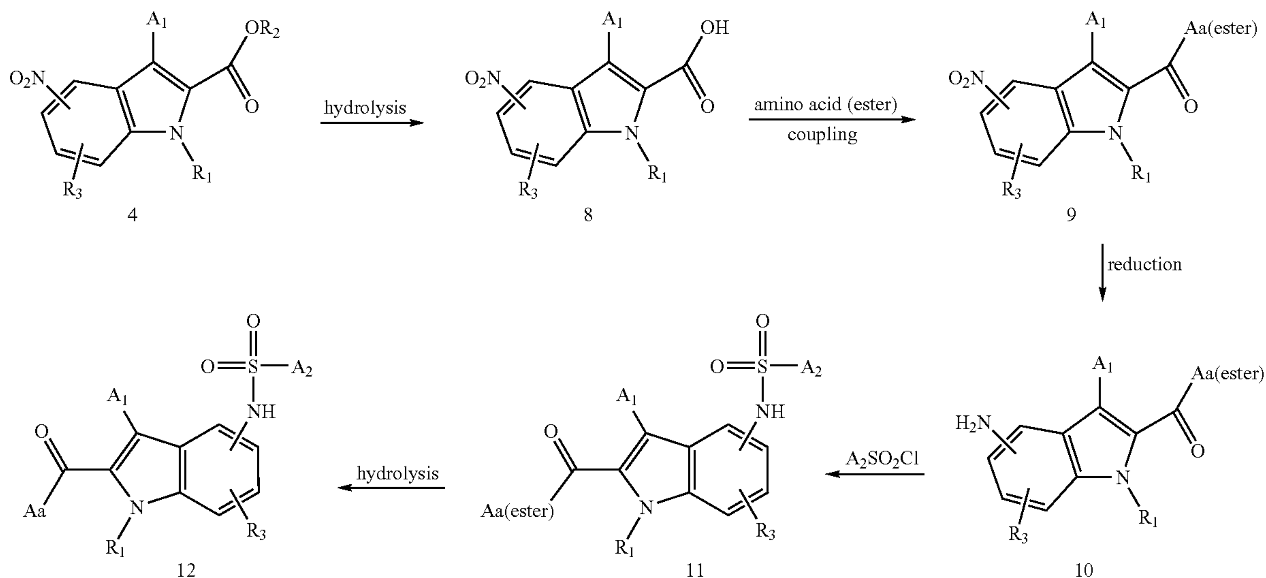
Scheme 2
