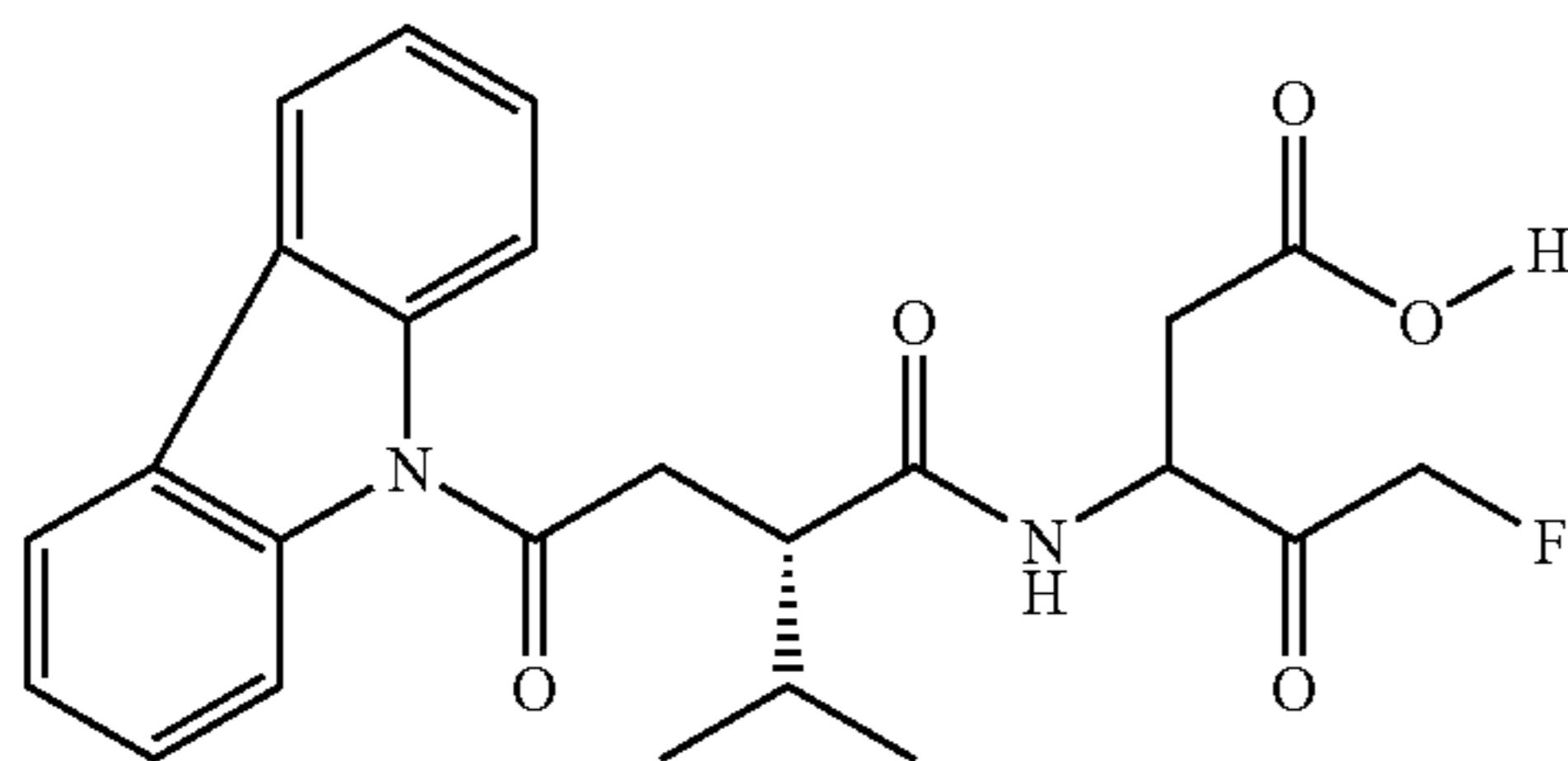
[3S/R(2S)]-3-[2-(2-Carbazol-9-yl-2-oxo-ethyl)-3-methyl-butrylamino]-5-fluoro-4-oxo-pentanoic acid
