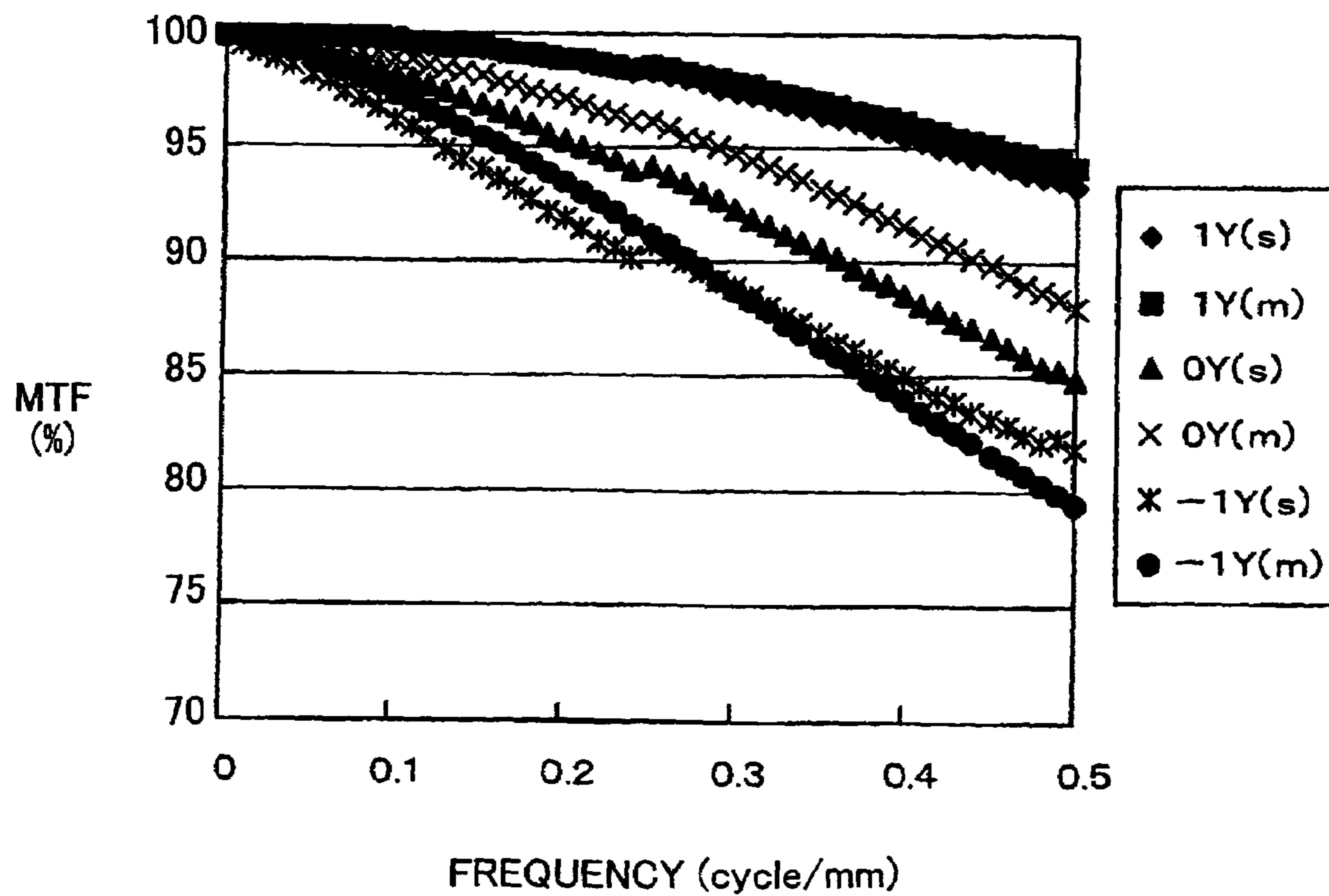
MTF CHARACTERISTICS 1 X=0
