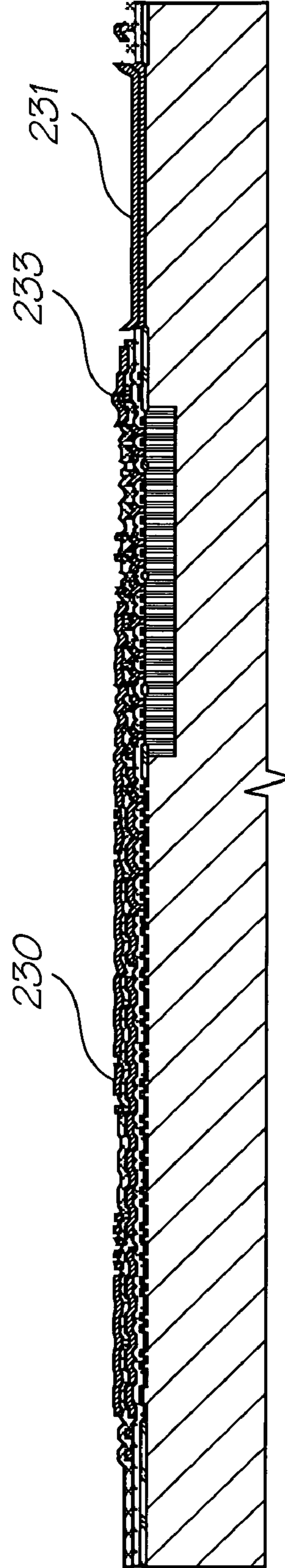
Deposit metal 2
