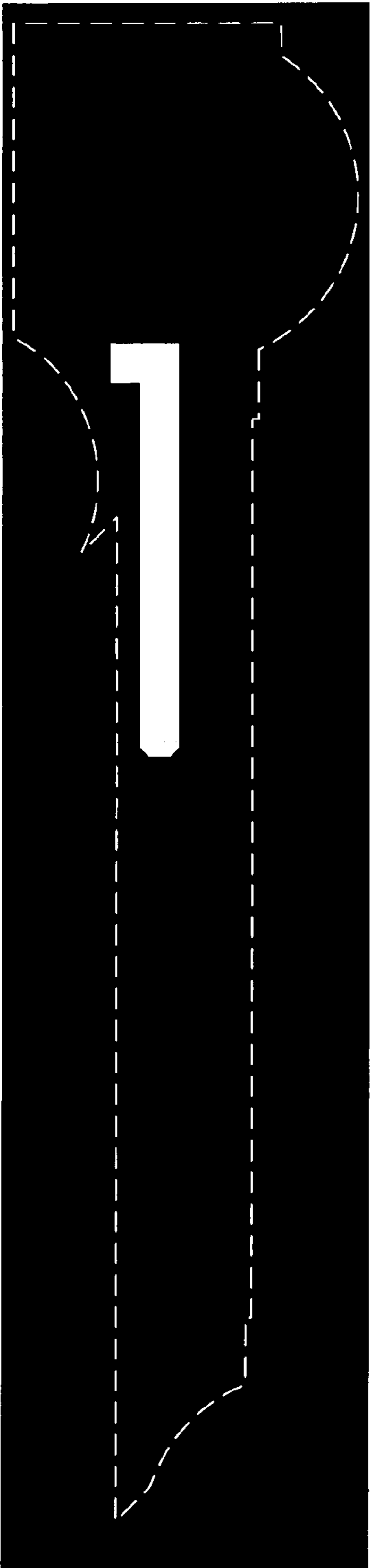
N-Well mask
