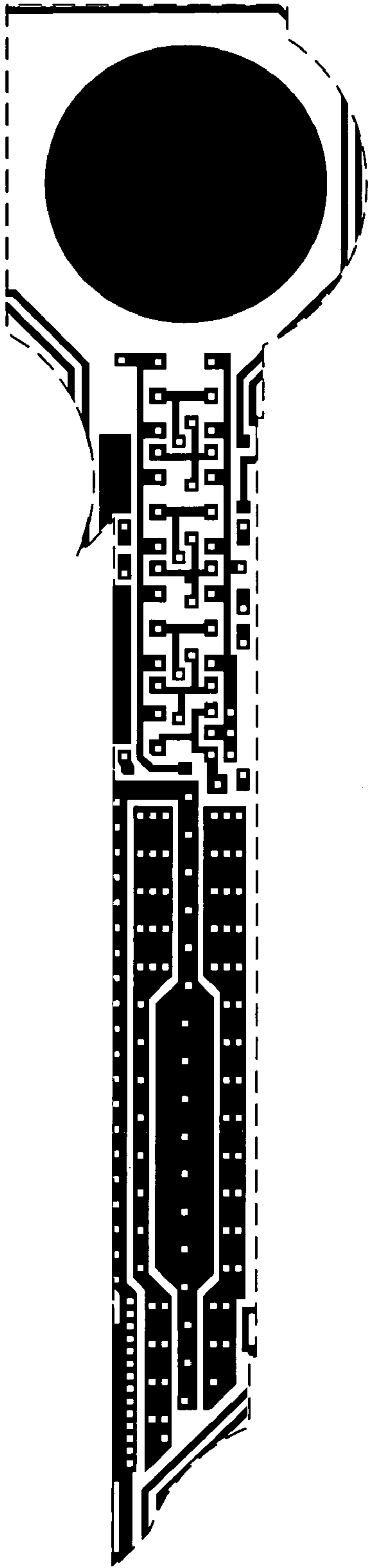
Metal 1 mask
