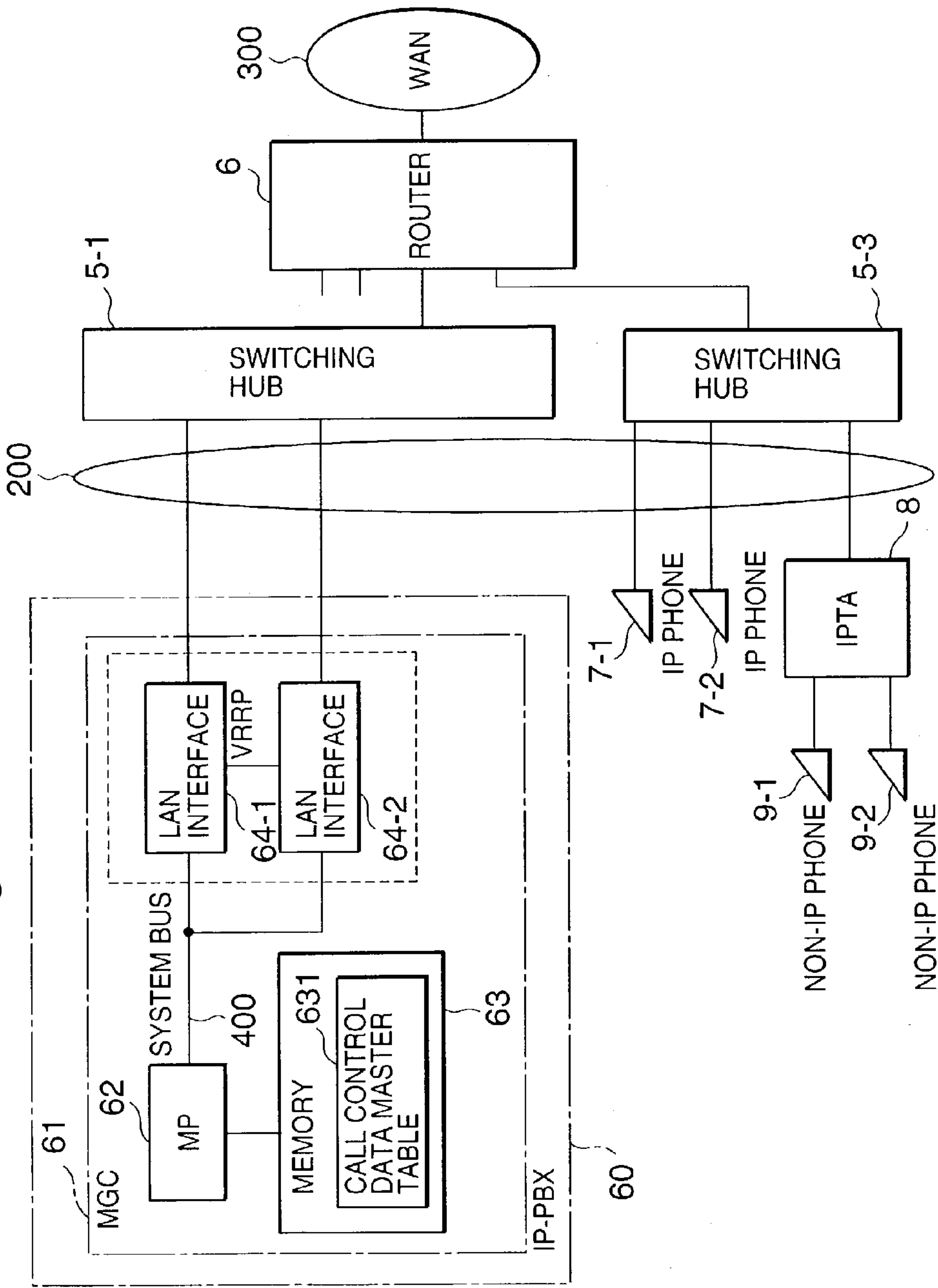
Fig. 12 (PRIOR ART)
