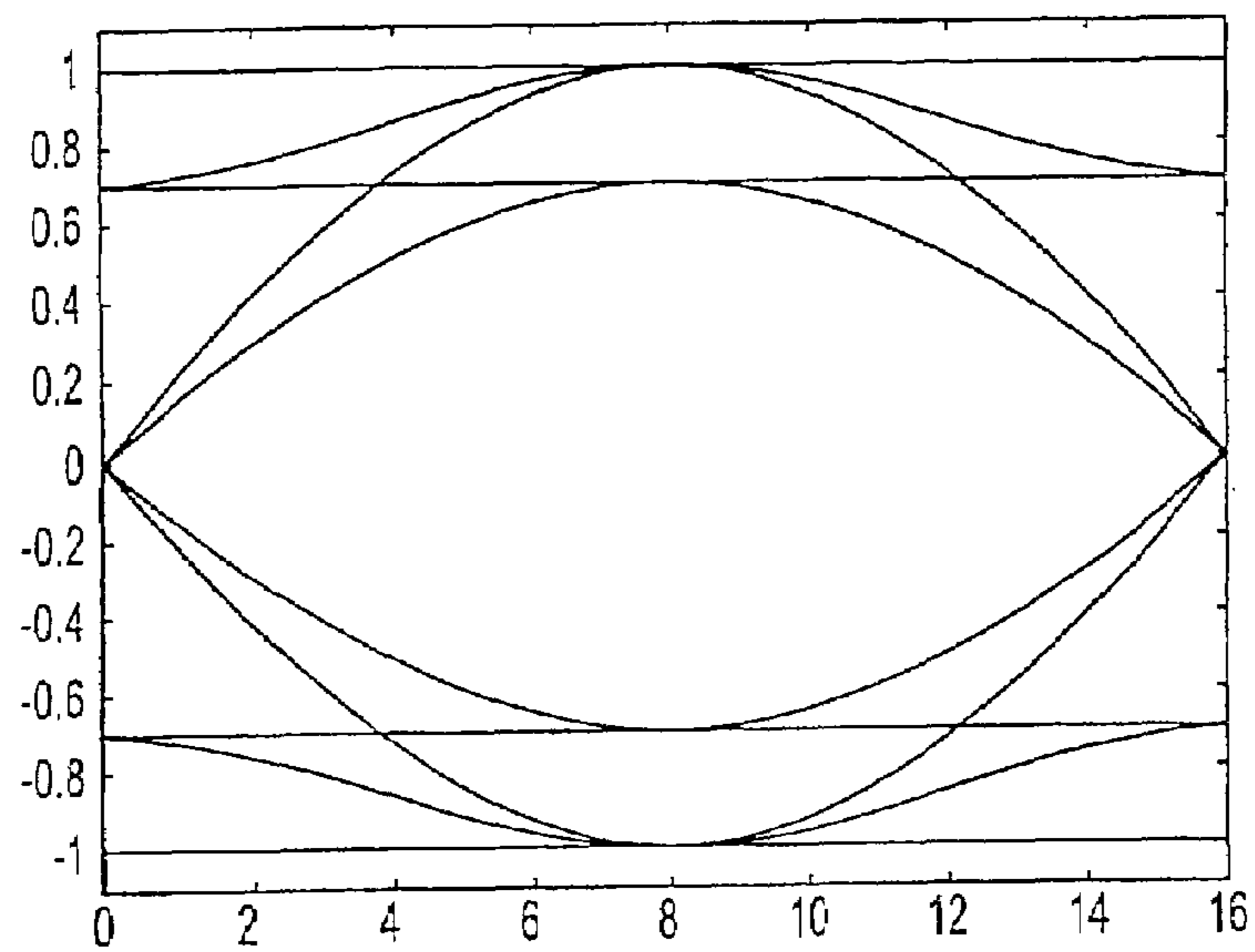
FQPSK COMPUTER. GENER. A=0.7, NO POST TCS FILTERING
