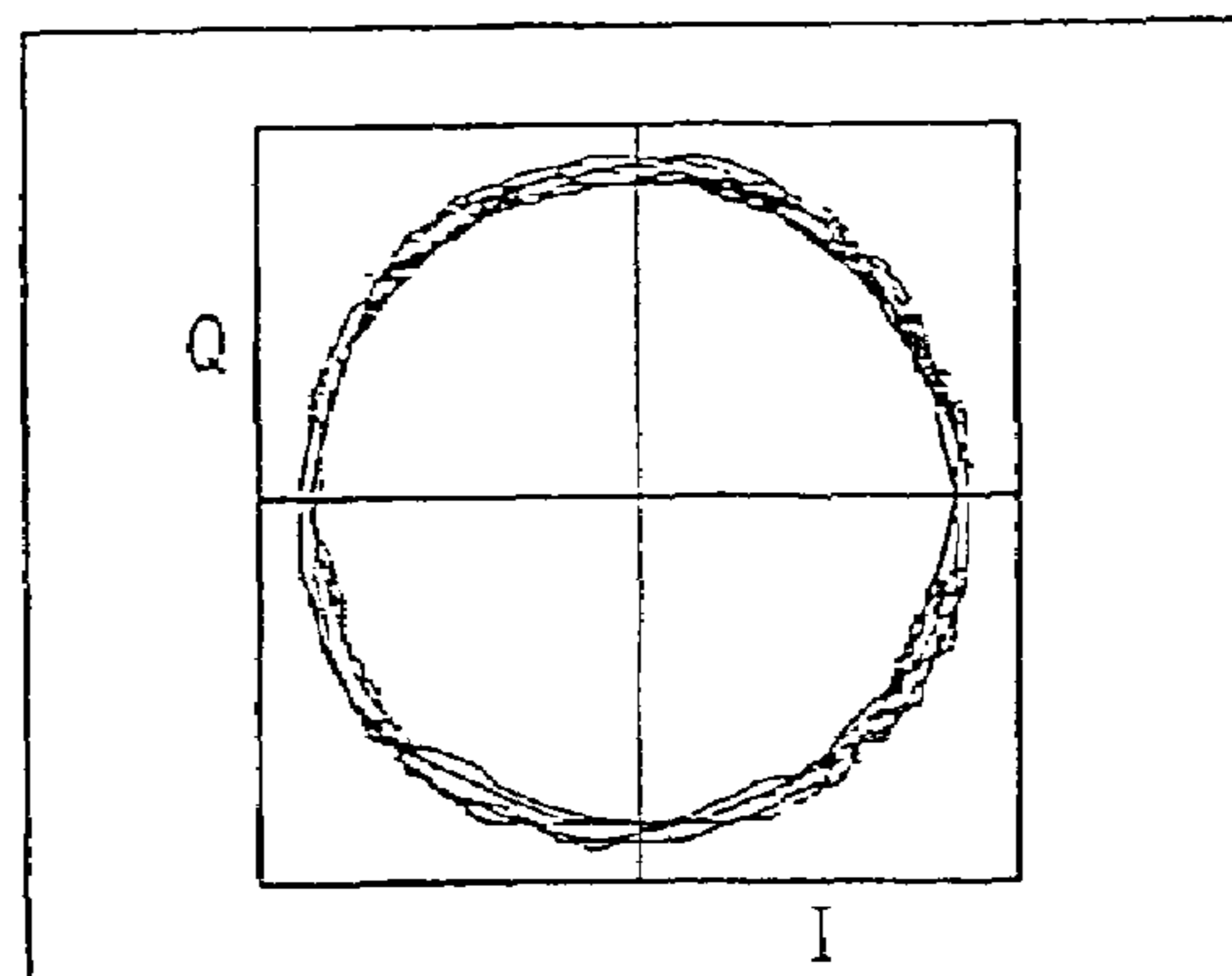
FQPSK-B. VECTOR CONSTELLATION
