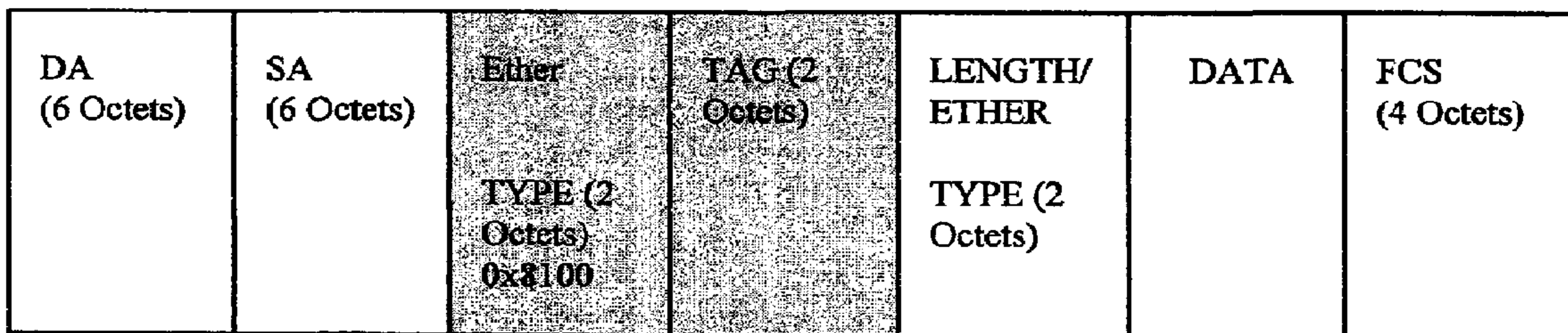
FIG. 3 (PRIOR ART)
