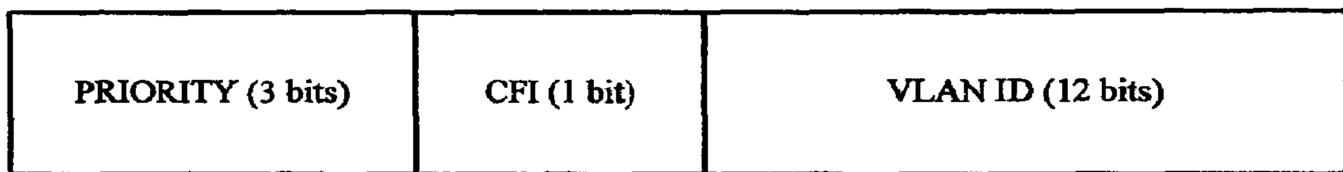
FIG. 4 (PRIOR ART)
