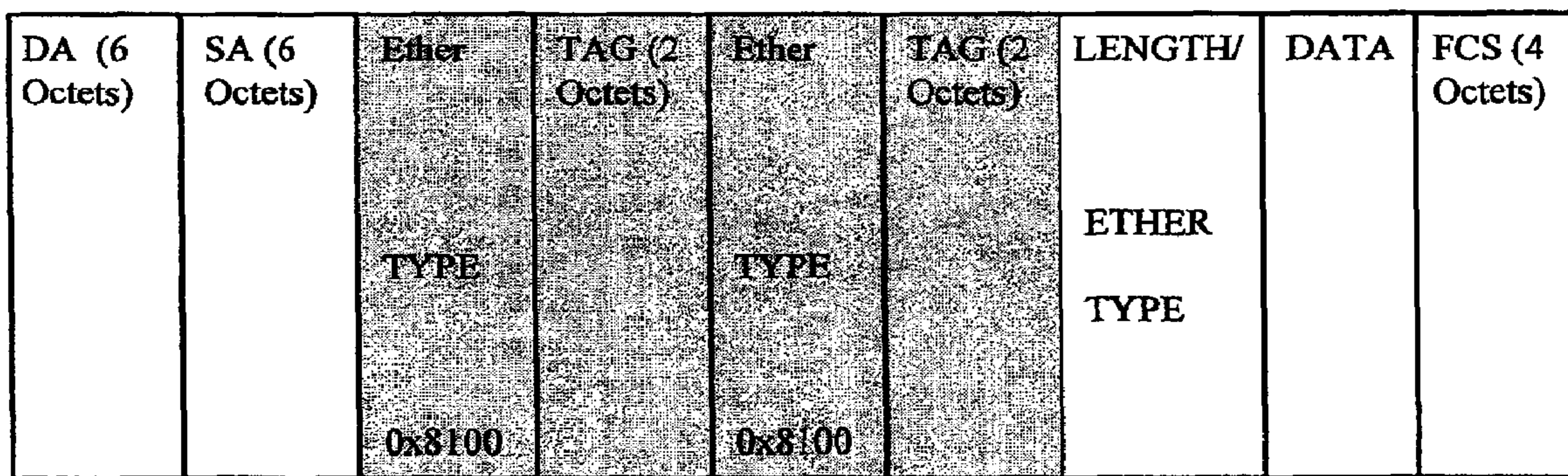
FIG. 5 (PRIOR ART)
