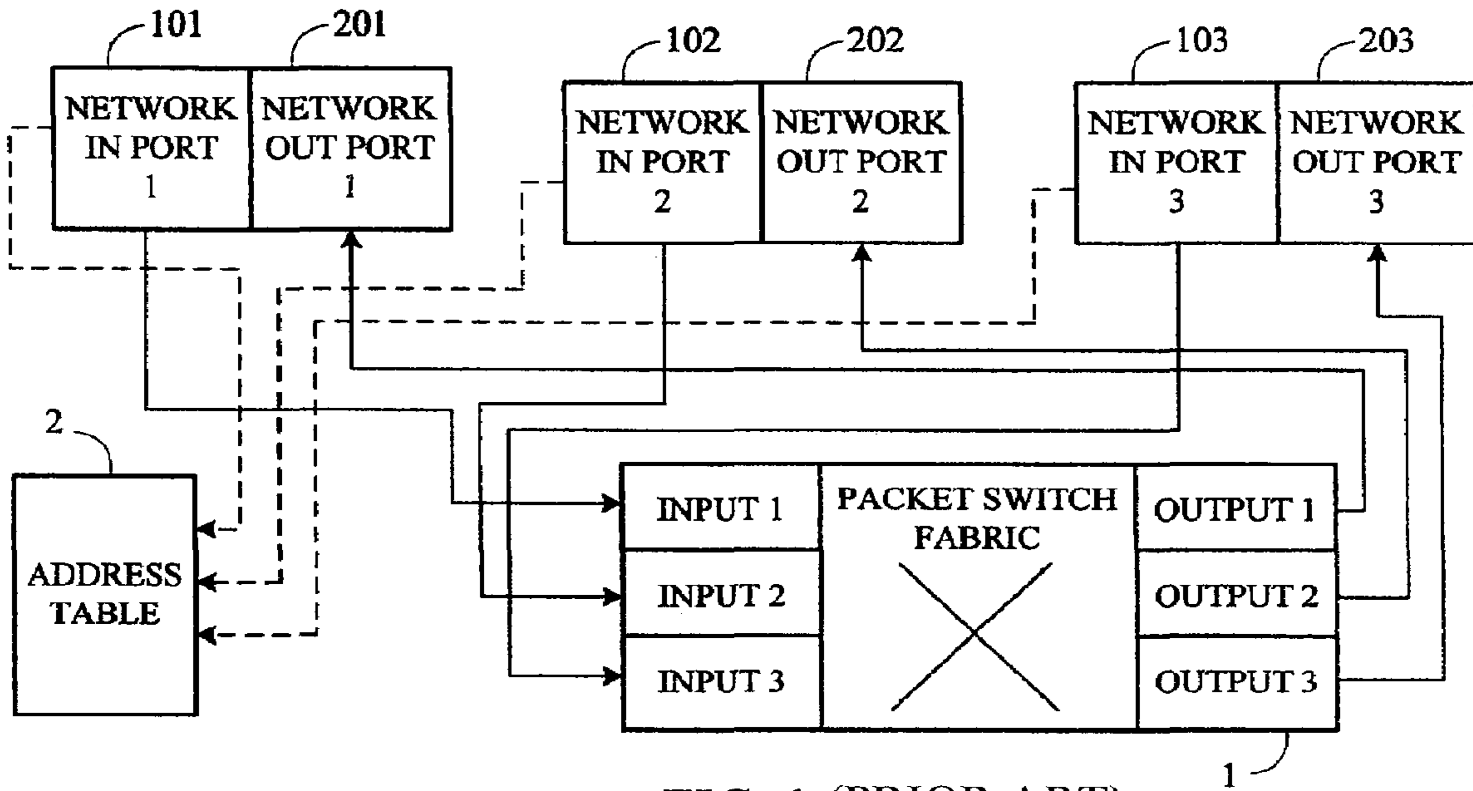
FIG. 1 (PRIOR ART)
