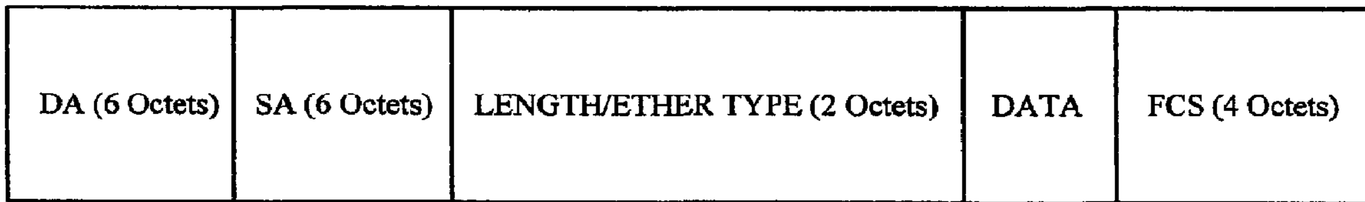
FIG. 2 (PRIOR ART)
