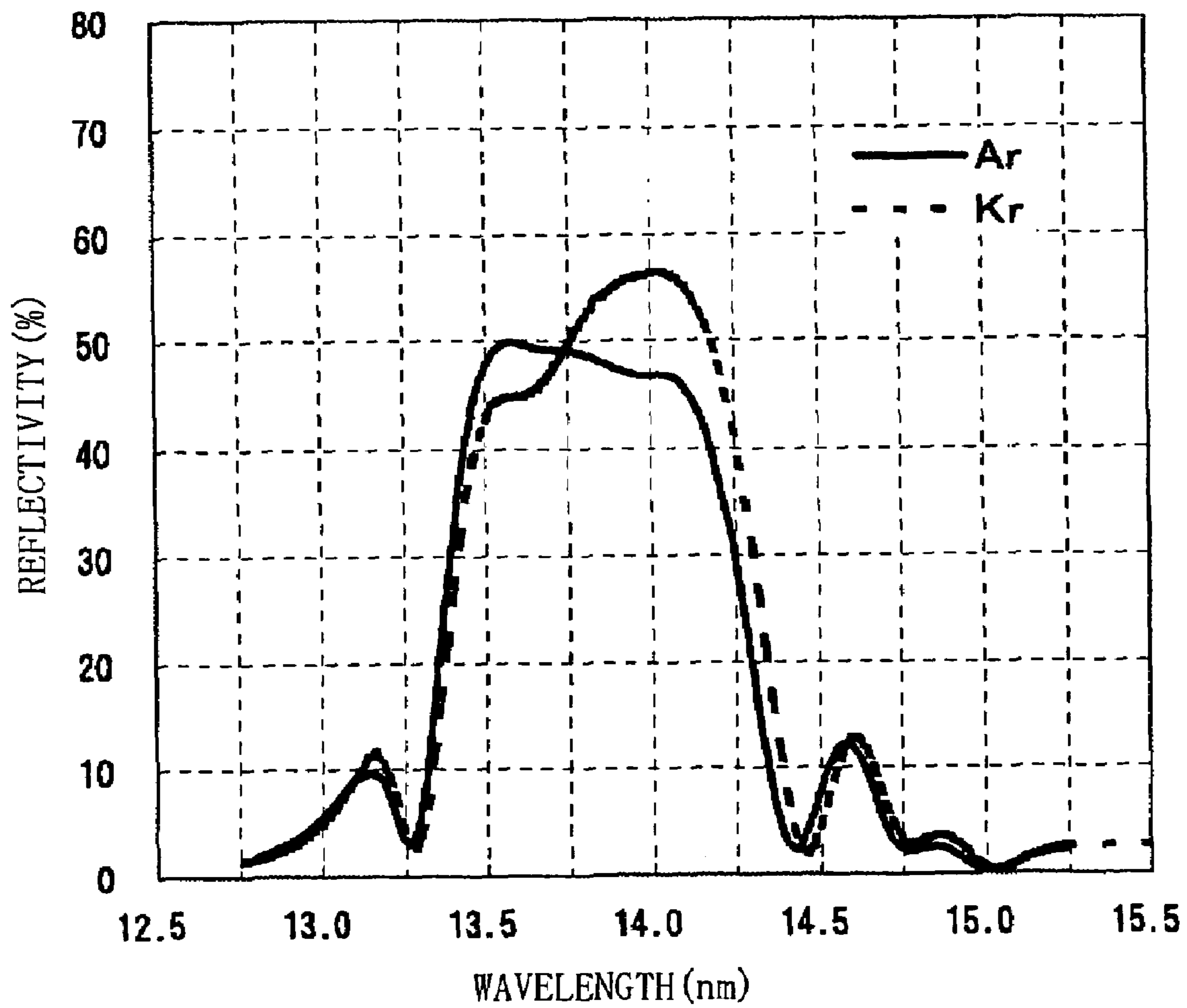
SPECTRAL REFLECTIVITY (AT VERTICAL INCIDENCE)
