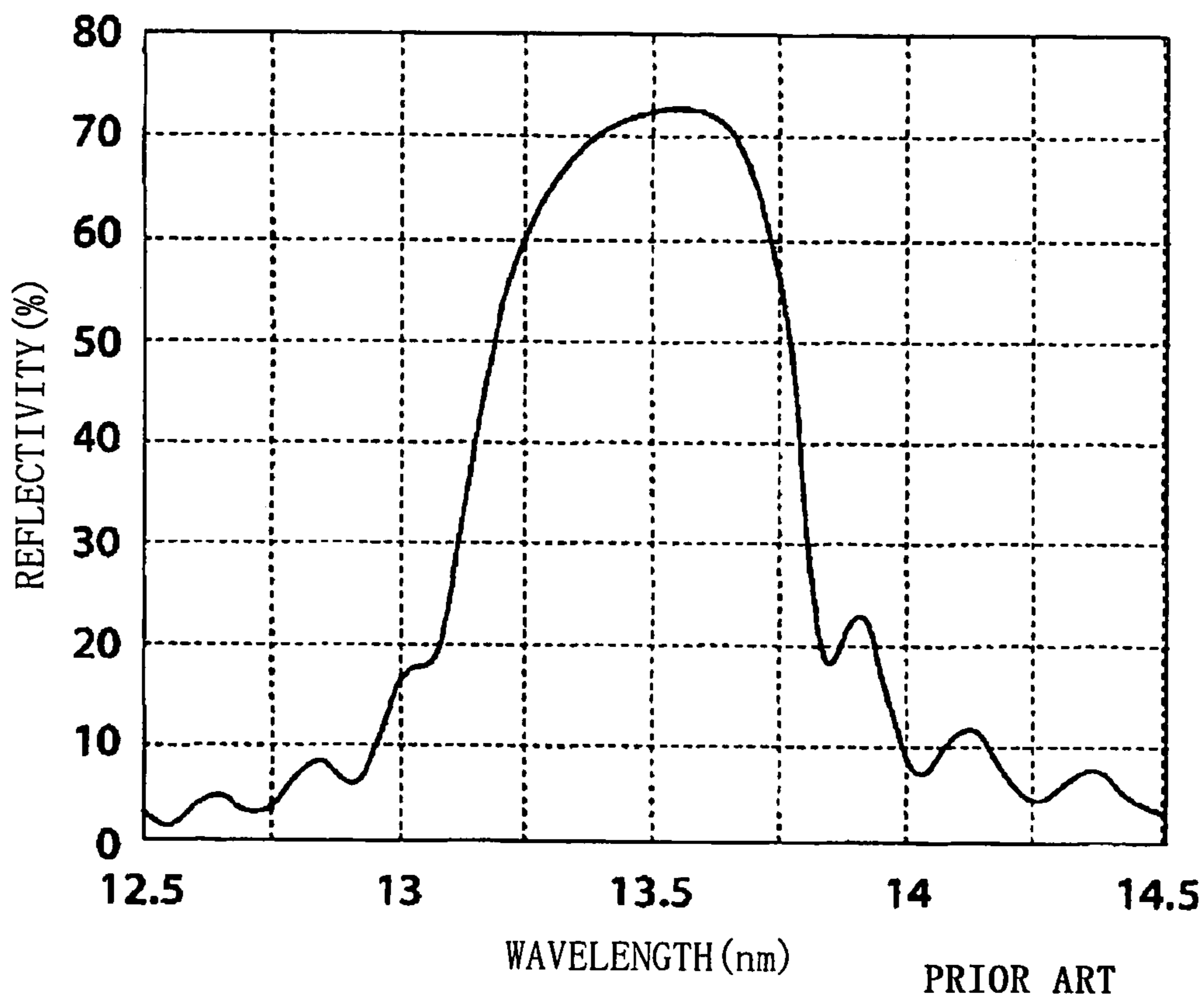
SPECTRAL REFLECTIVITY OF PRIOR ART MULTILAYER (AT VERTICAL INCIDENCE)
