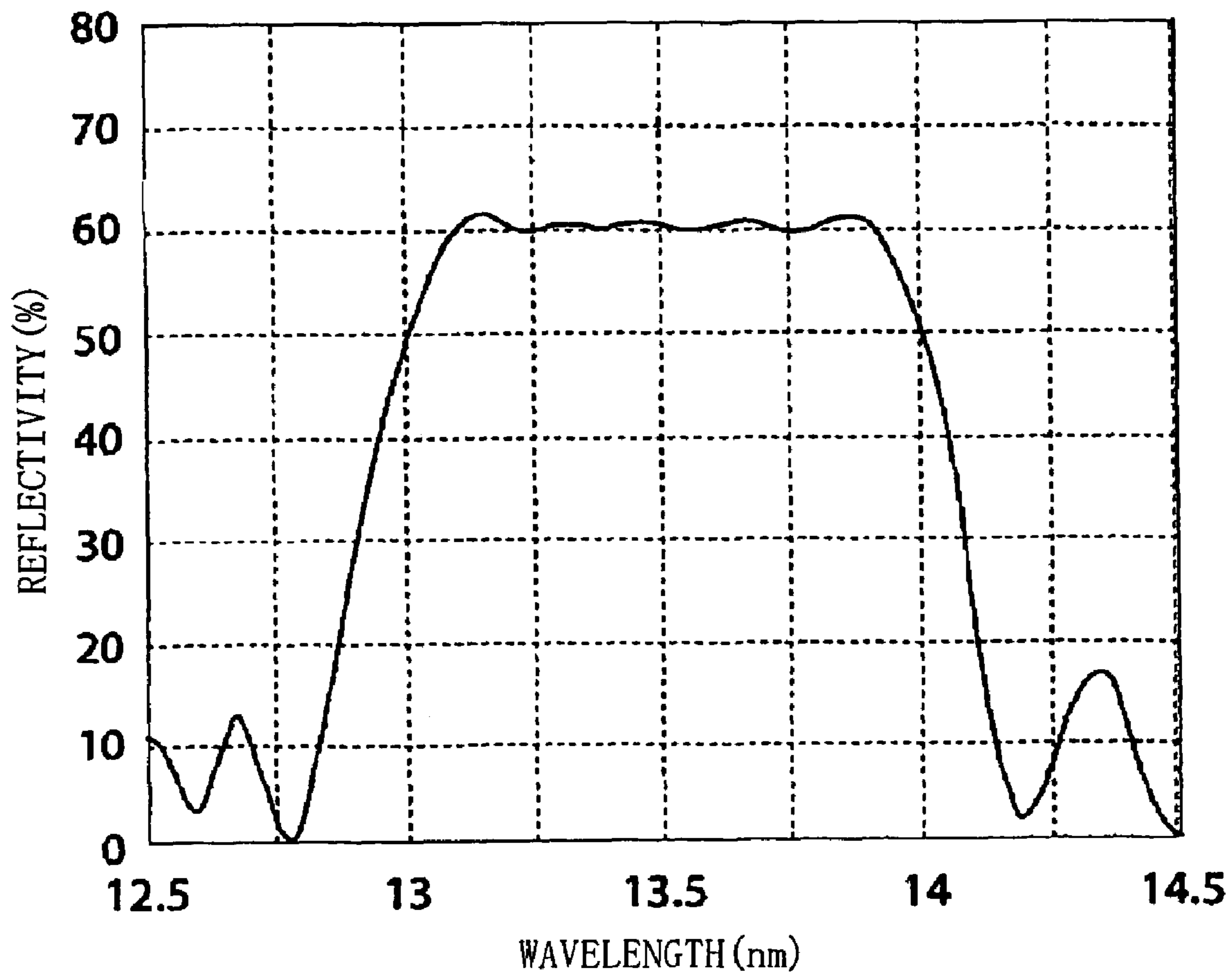
SPECTRAL REFLECTIVITY (AT VERTICAL INCIDENCE)
