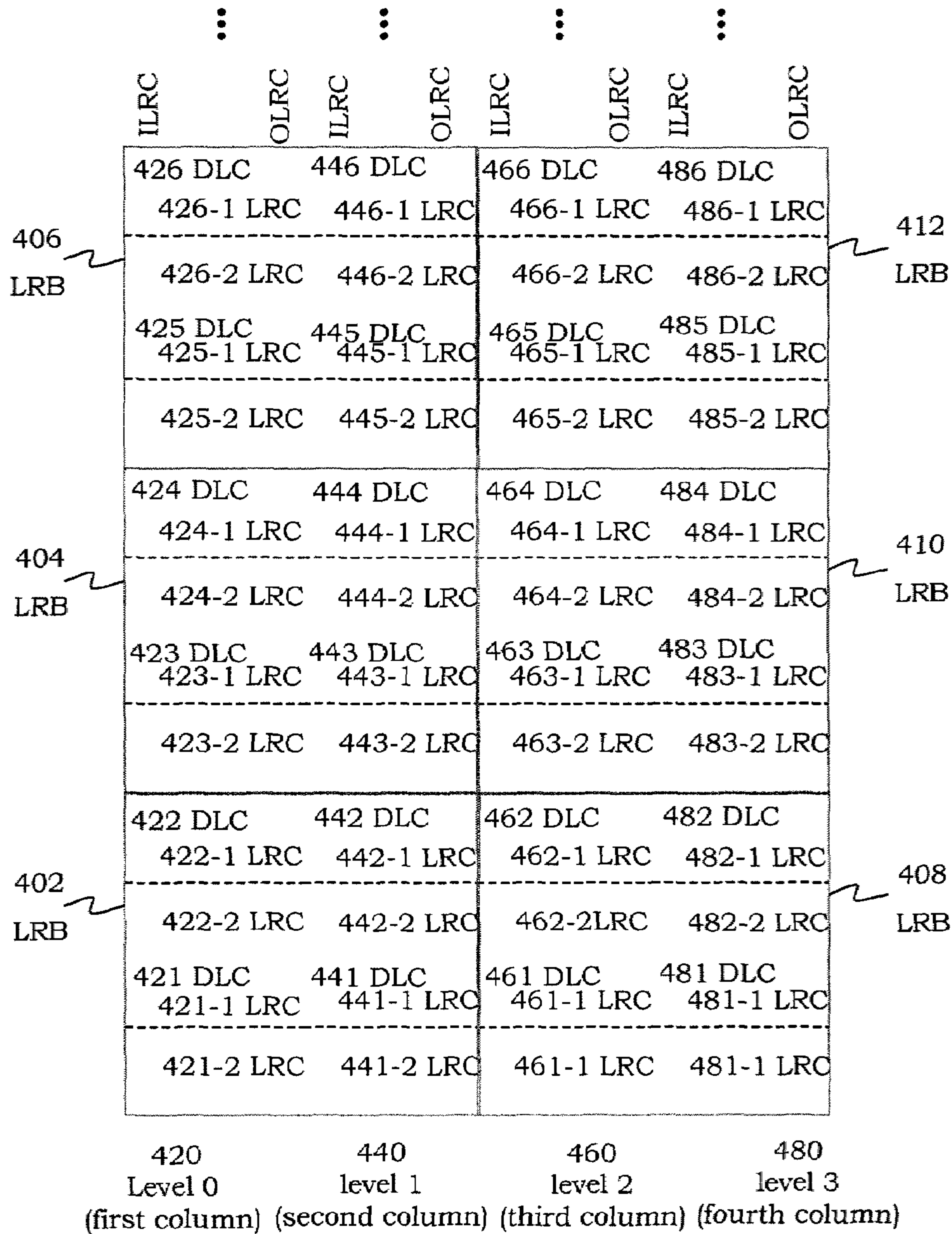
400 programmable logic chip levels of DLC 420 Level 0 (first column) 440 level 1 (second column) 460 level 2 (third column) 480 level 3 (fourth column)
