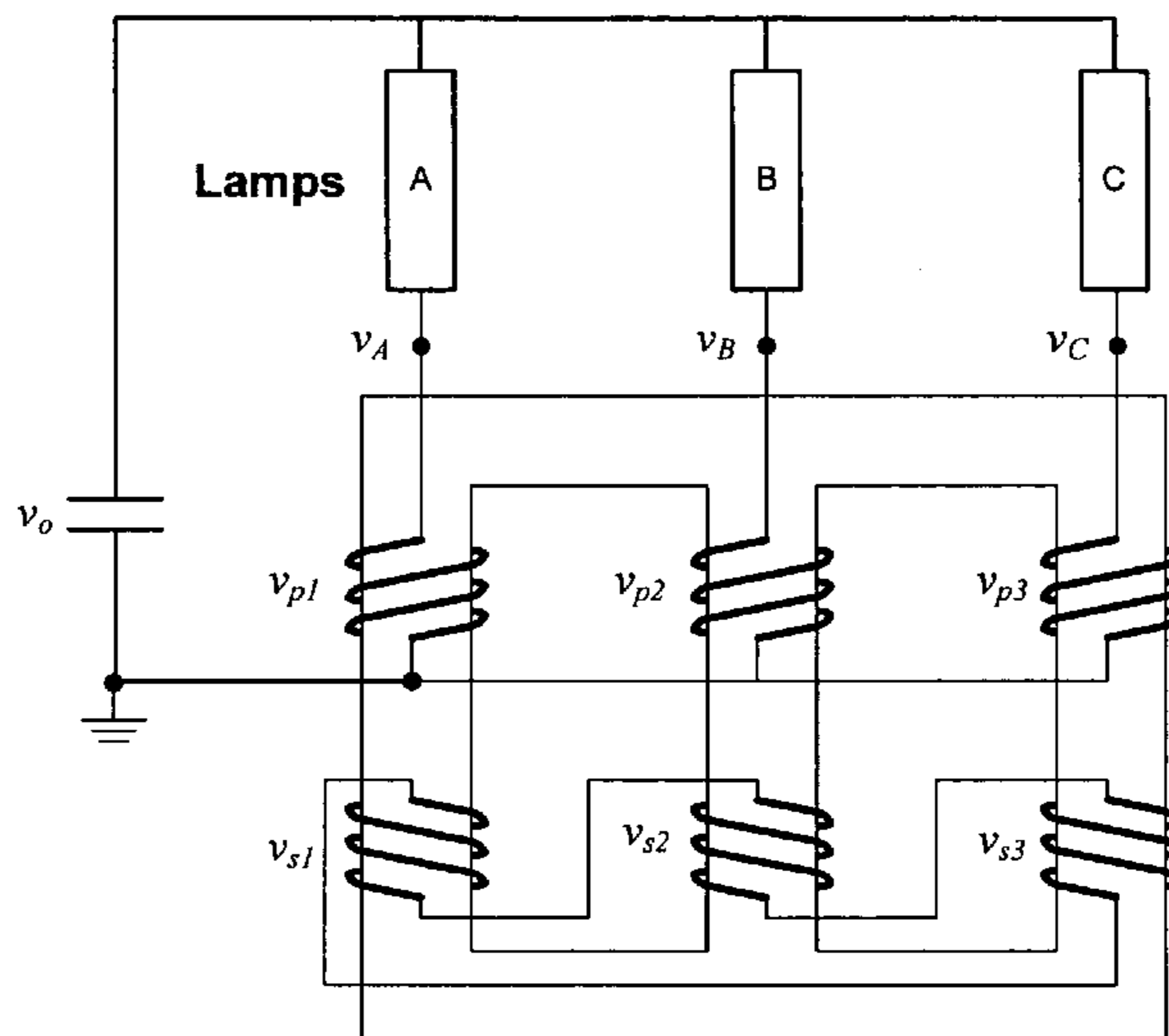
Integrated magnetic core with star-delta configuration.
