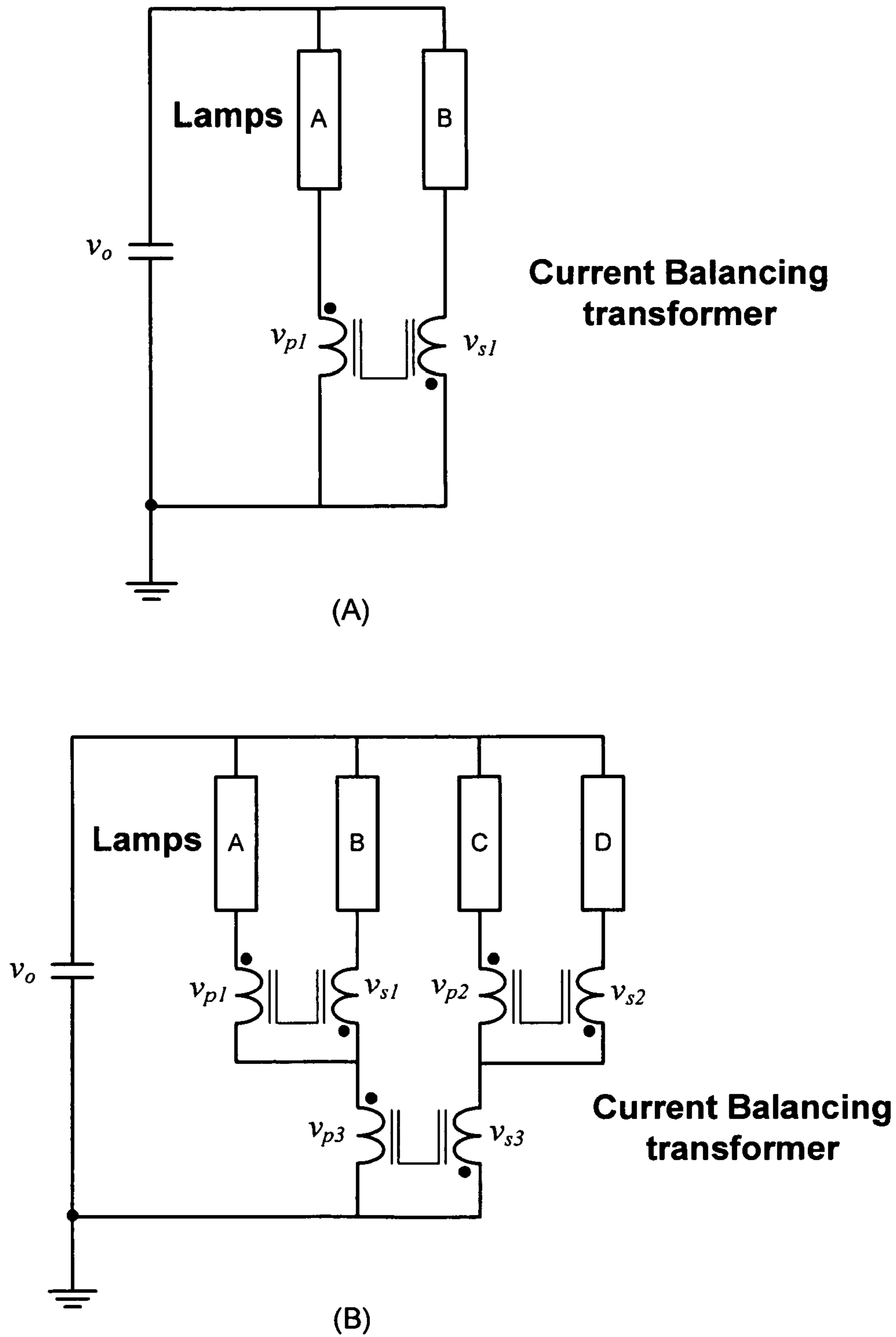
Available current balancing techniques.
