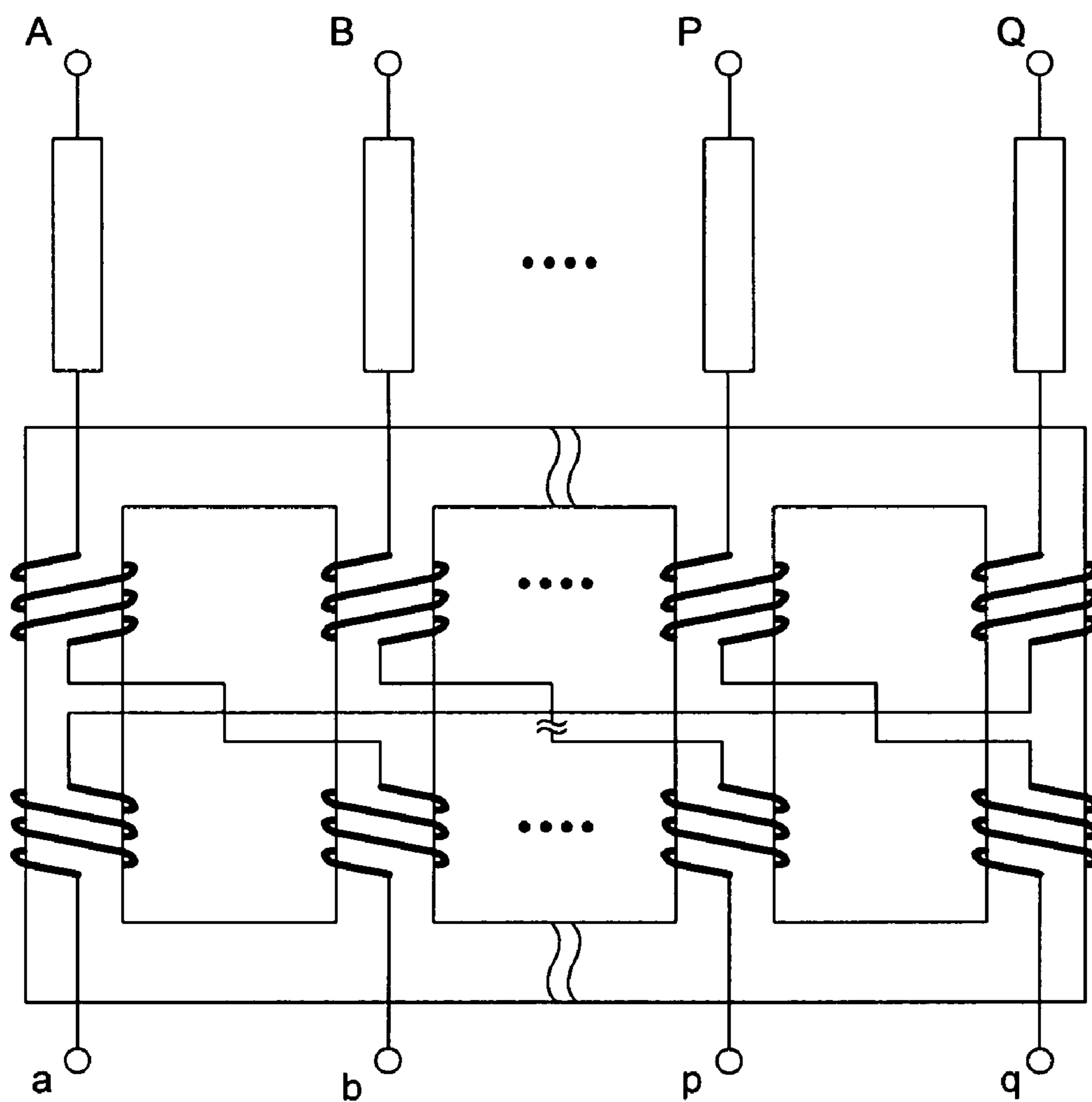
Multi-leg magnetic core with zig-zag connection.
