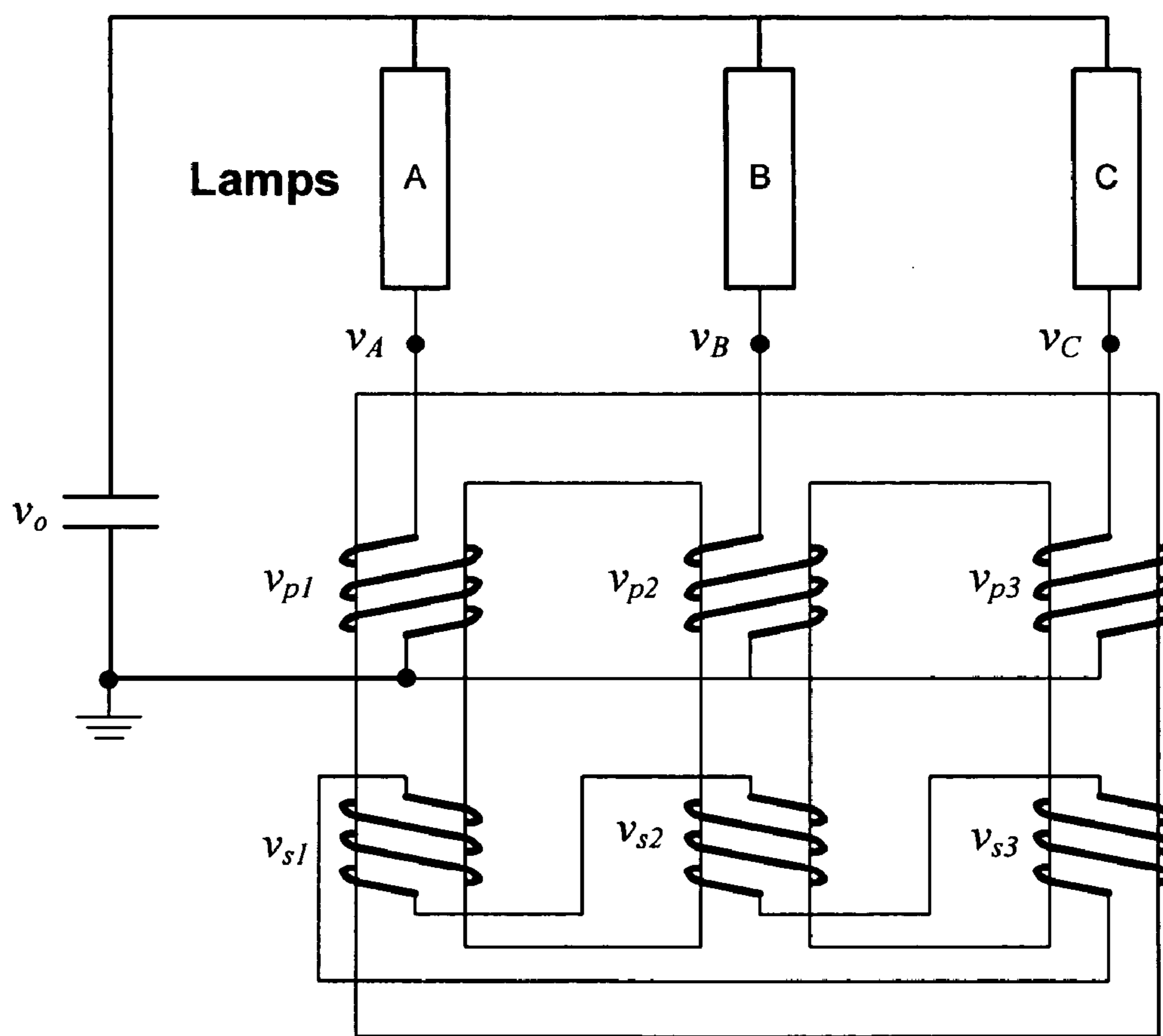
Integrated magnetic core with star-delta configuration.
