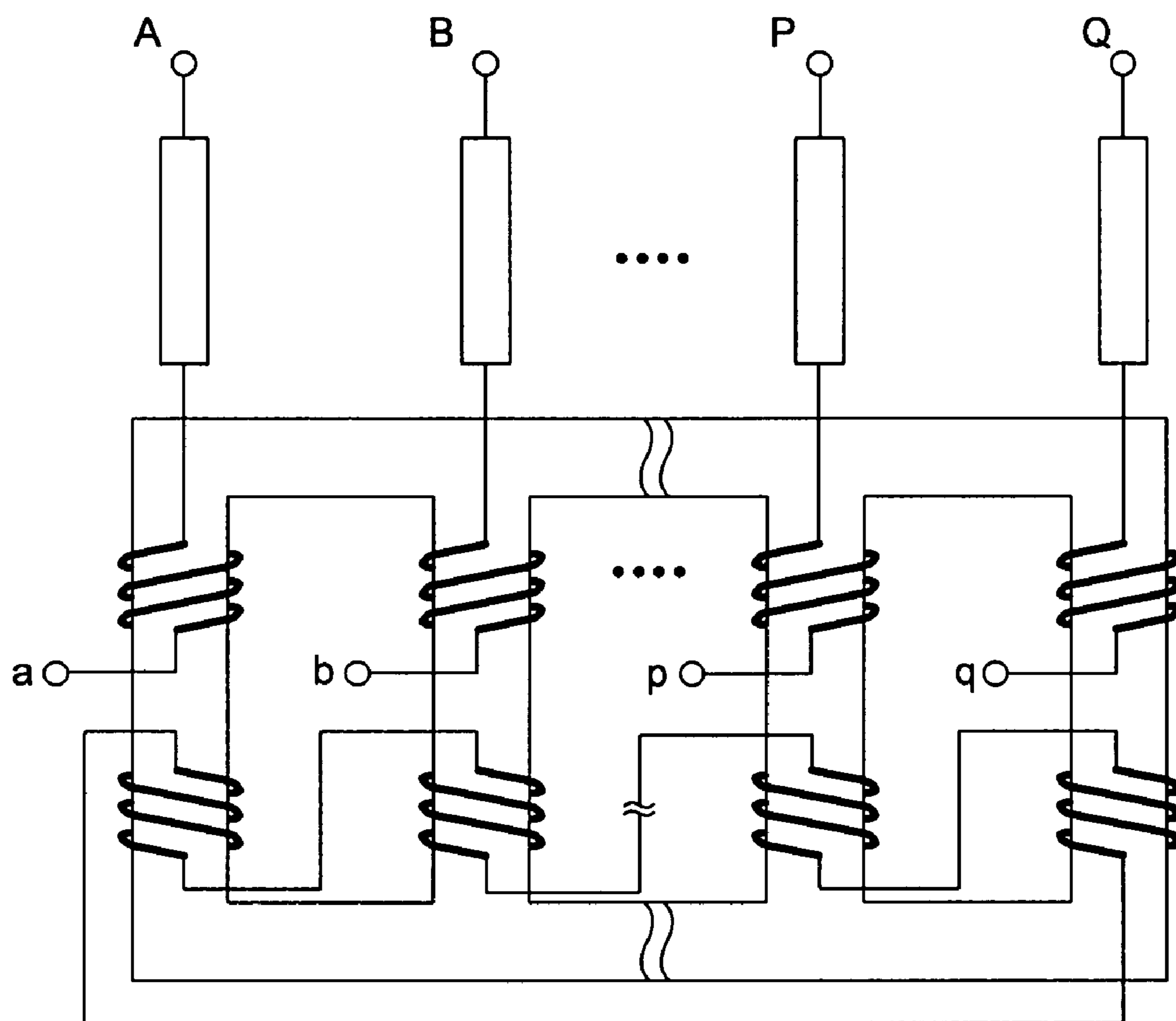
Multi-leg magnetic core with star-delta connection.
