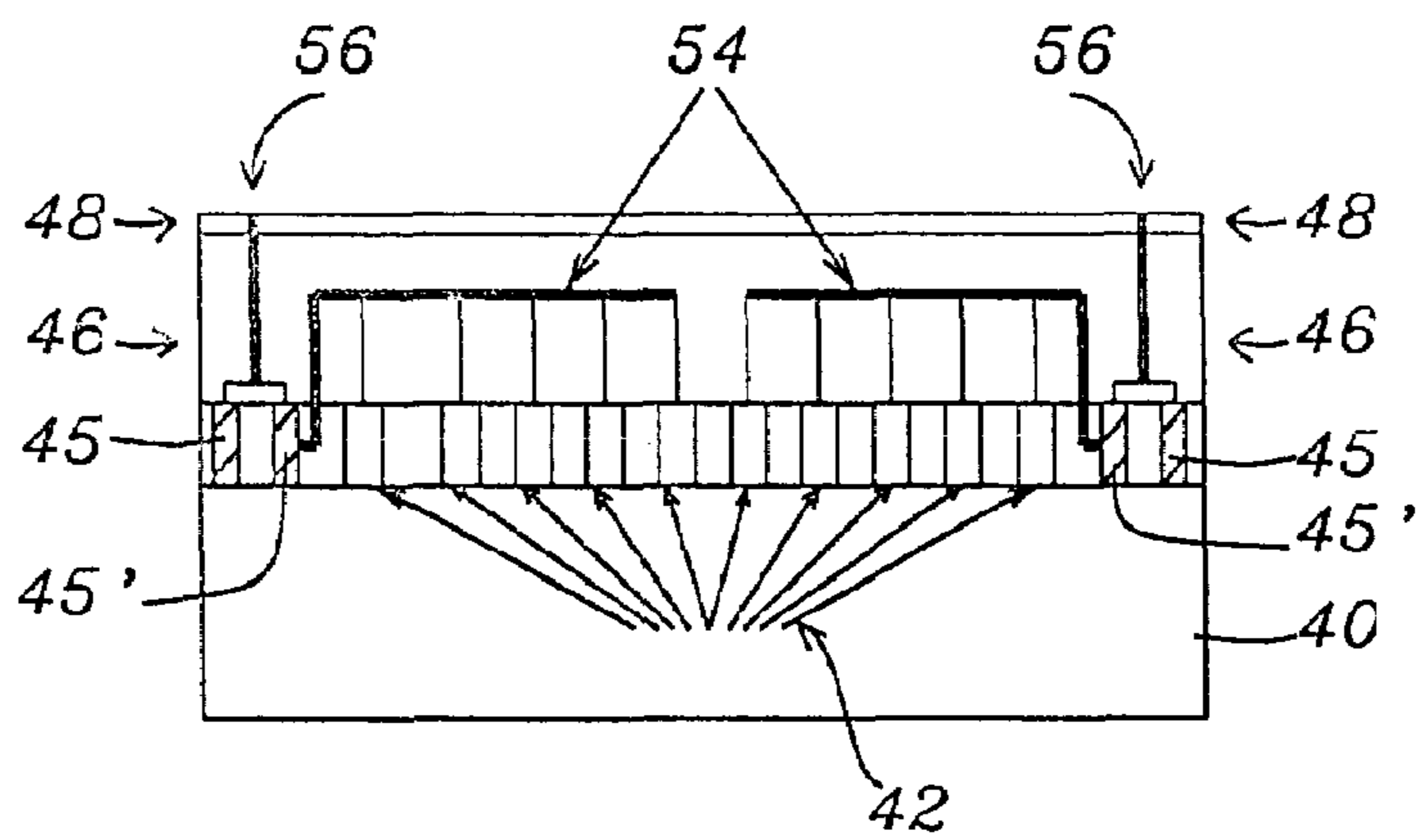
FIG. 2 - Prior Art
