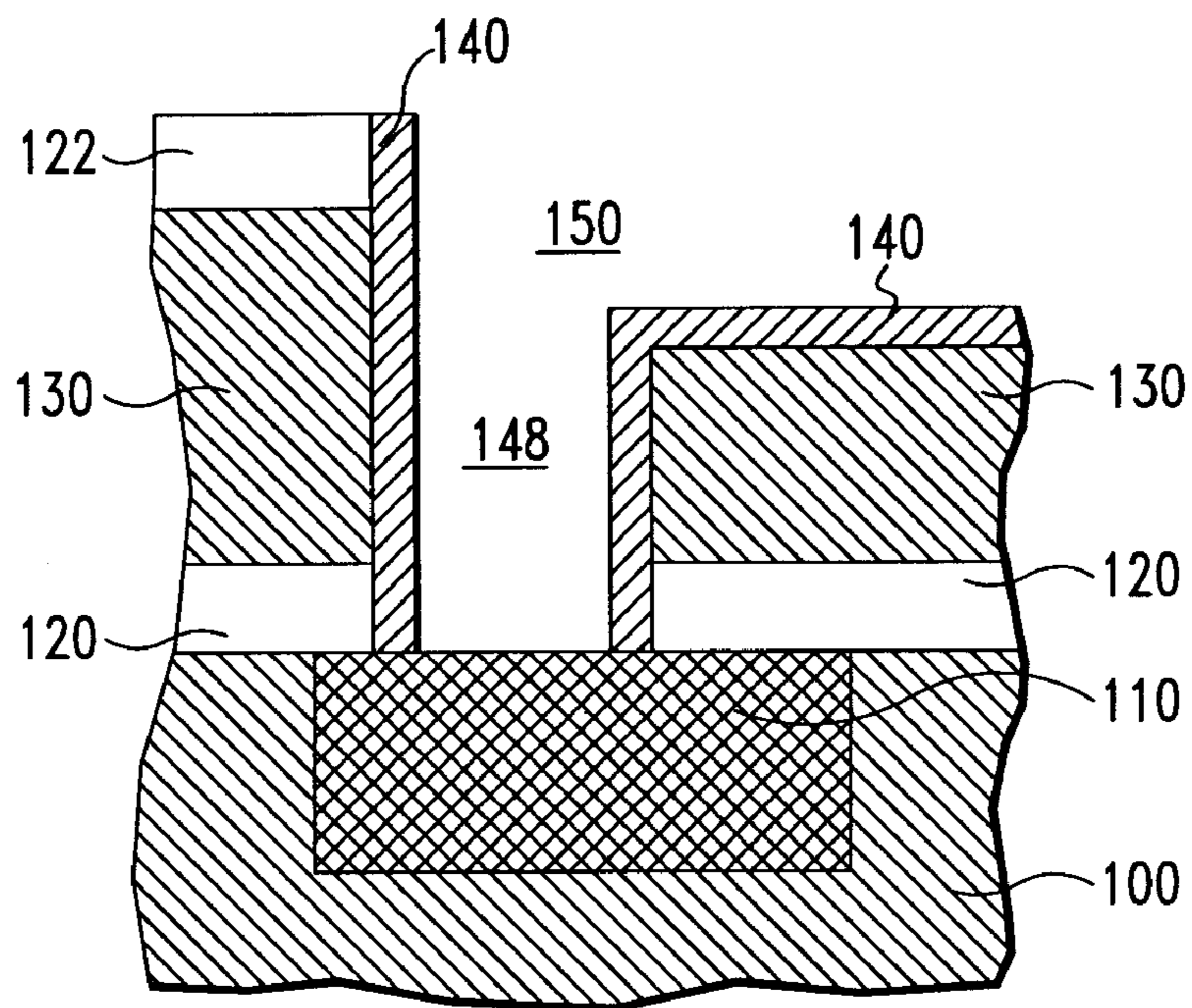
FIG. 1C Prior Art
