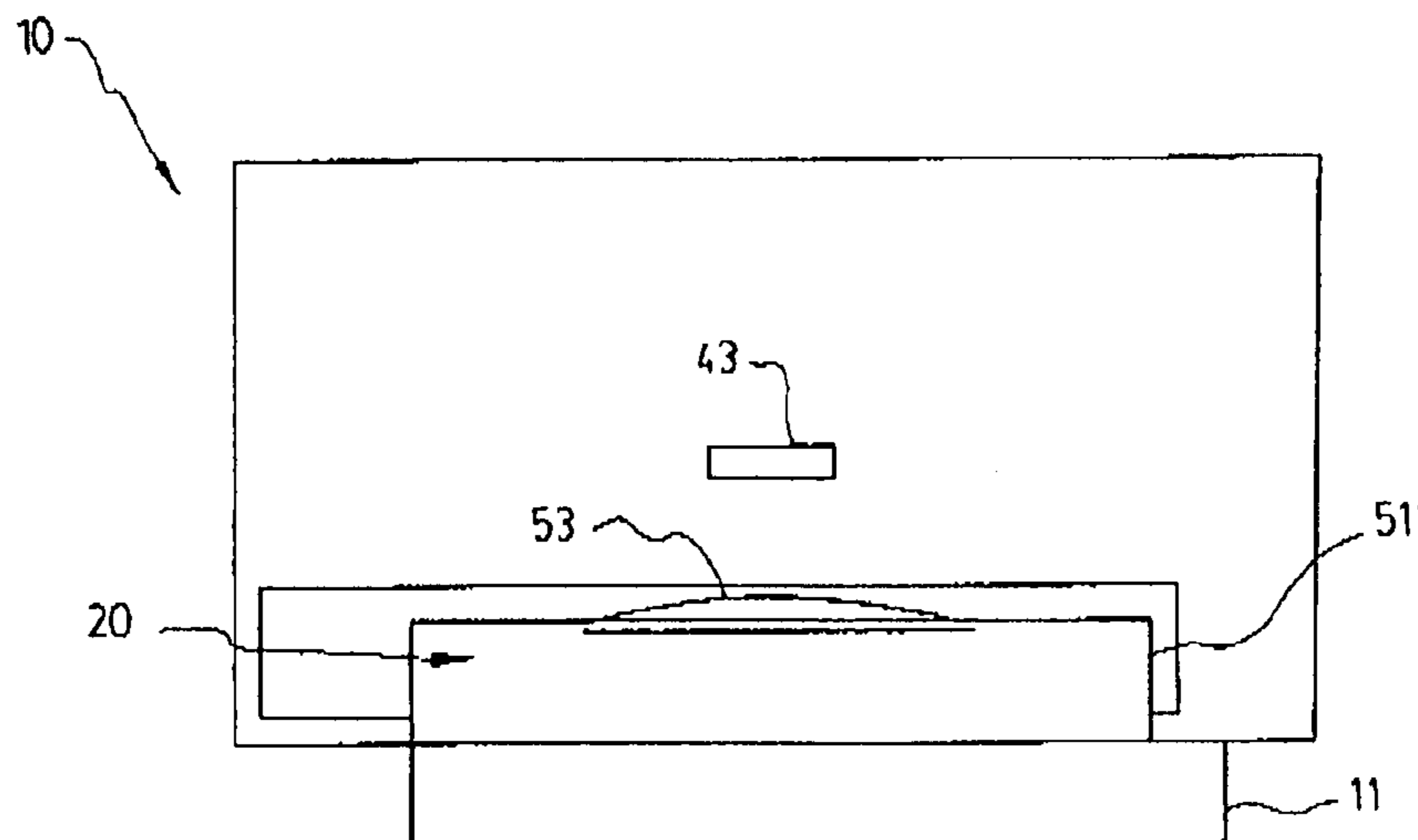
SIDE VIEW : SECOND PIXEL EMBODIMENT ( REFRACTIVE MICRO-LENS WITH PLANAR MIRROR )
