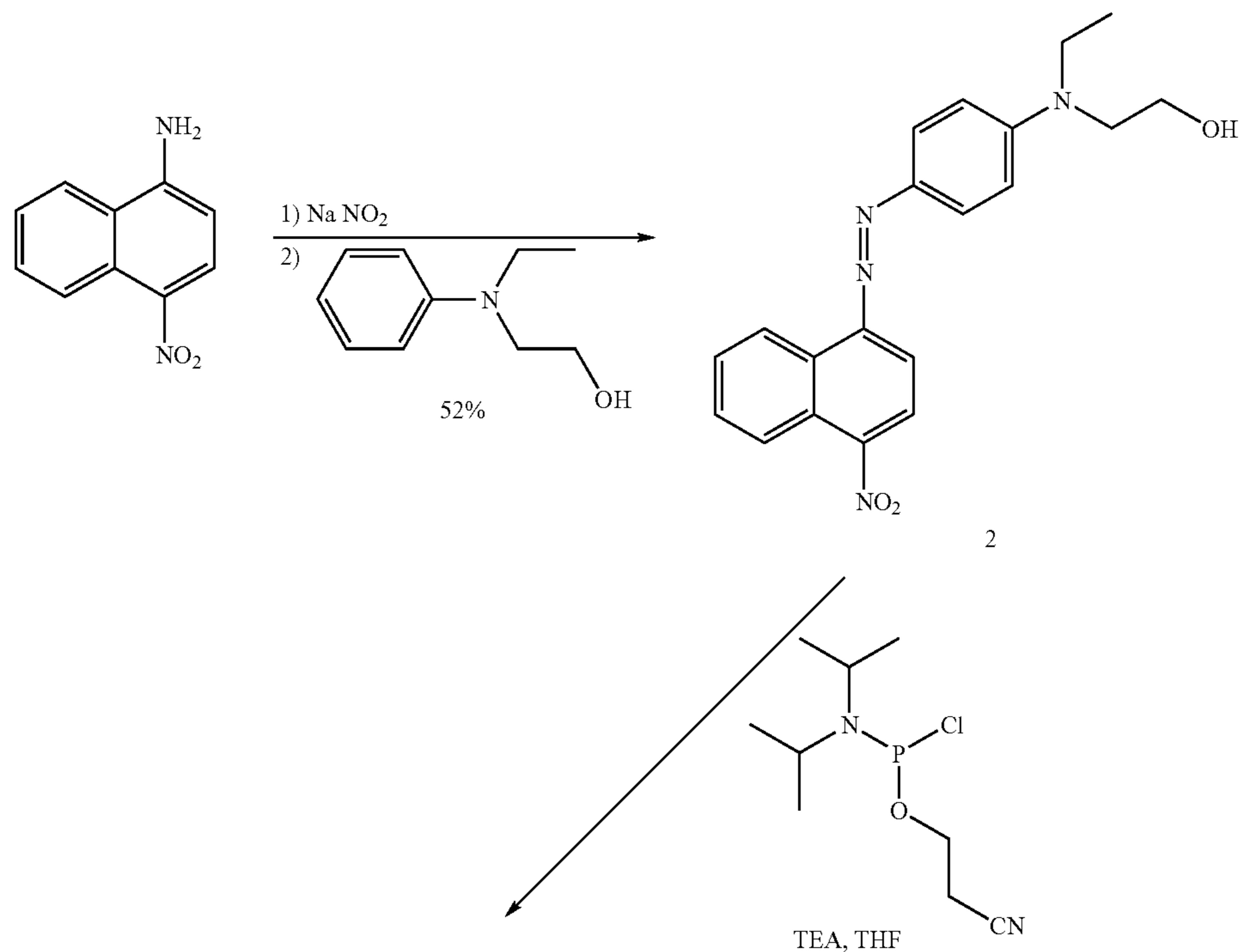
Scheme 1
