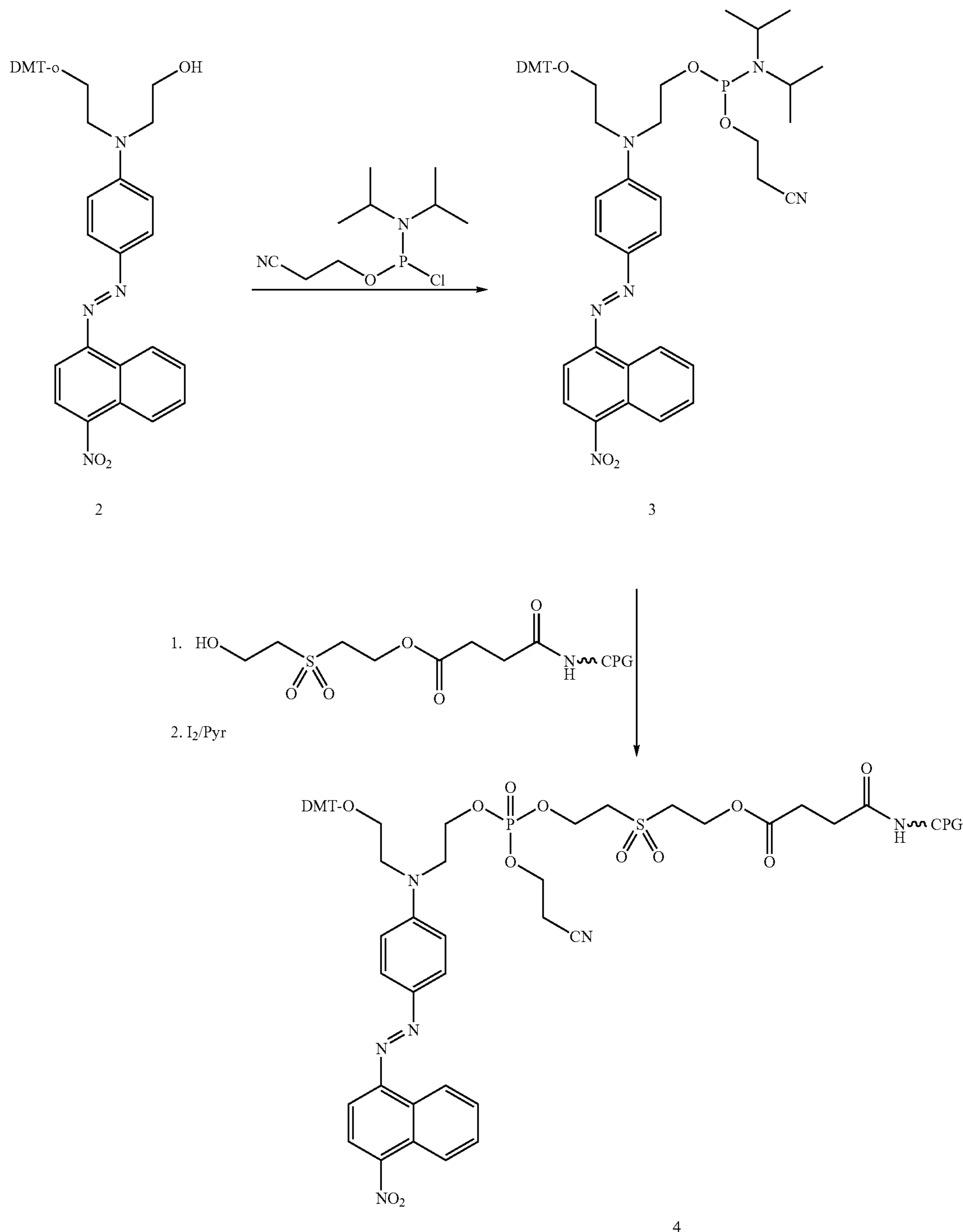
Scheme 3
