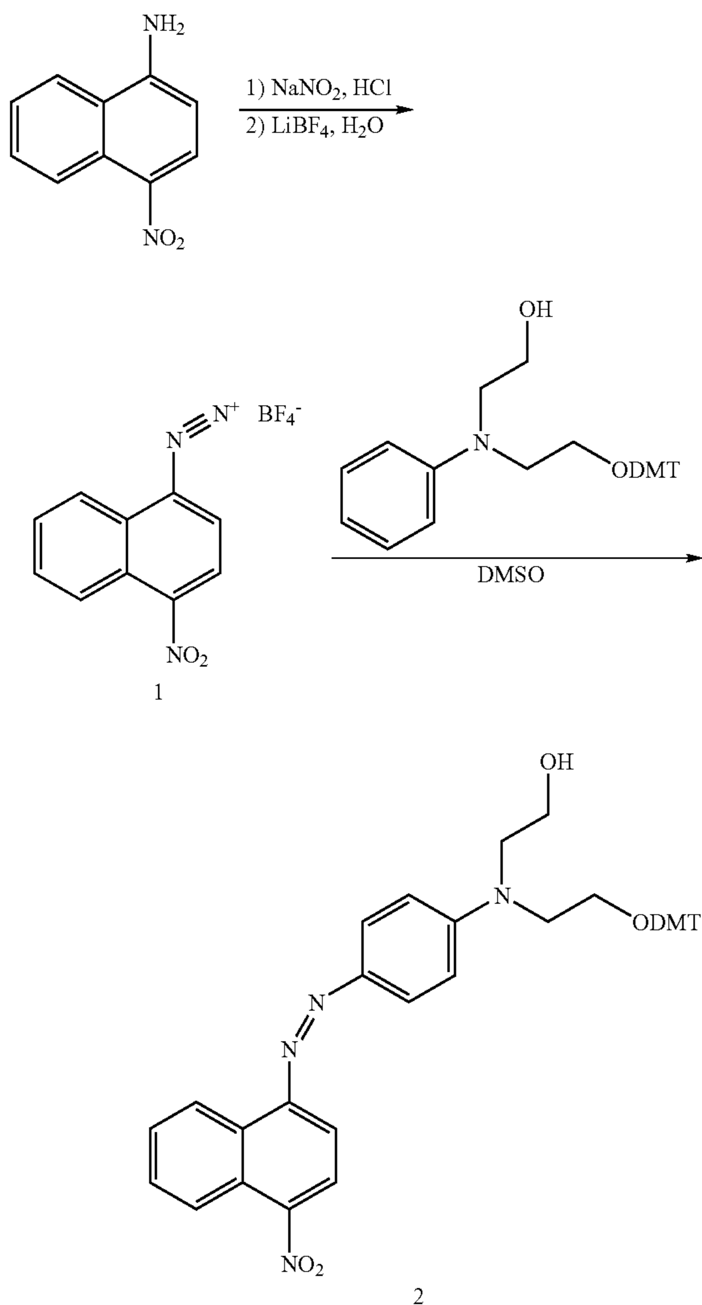
Scheme 2
