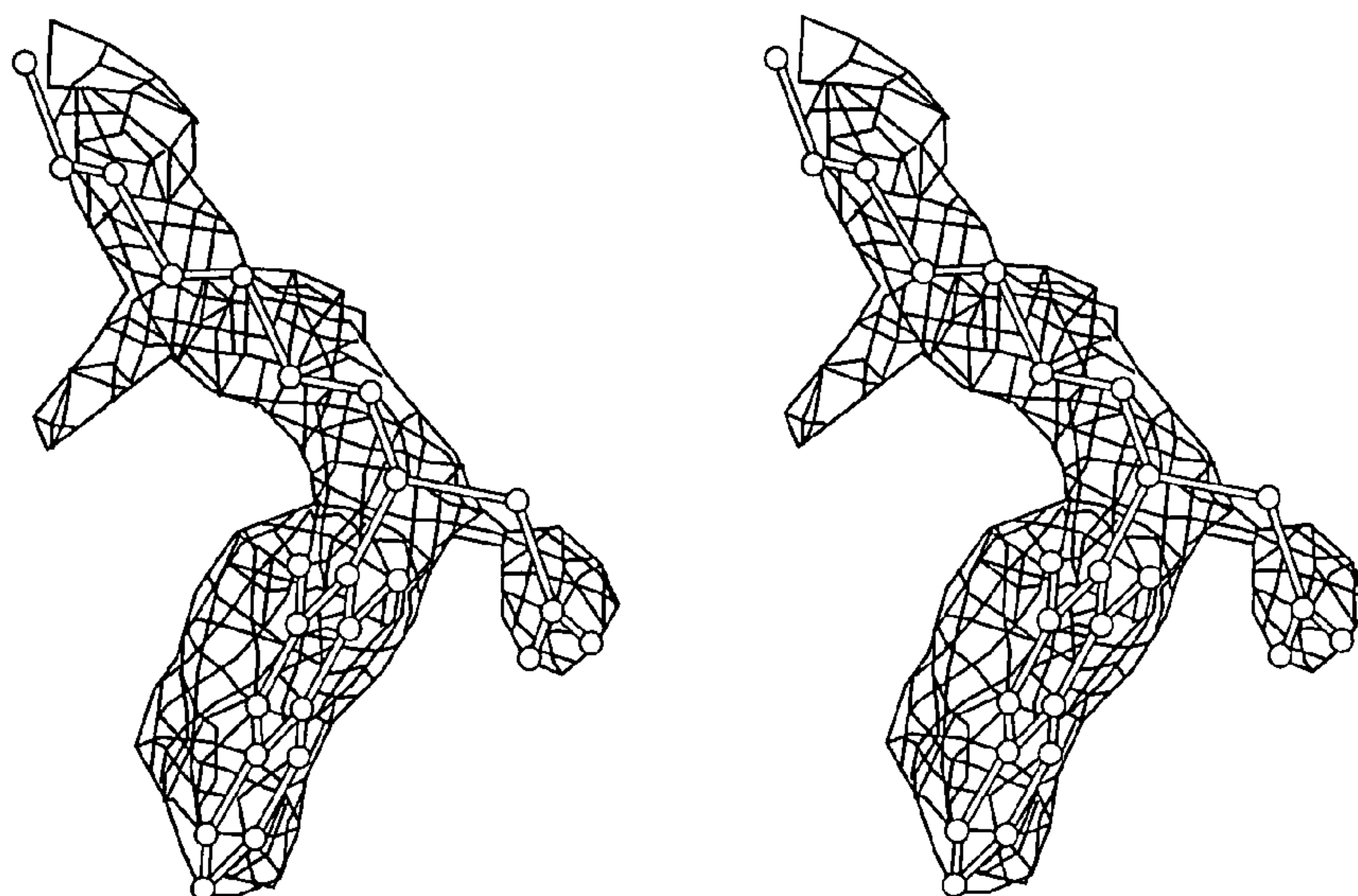
DIFFERENCE ELECTRON DENSITY (UNREFINED) OF NCP014 IN SITE 1A
