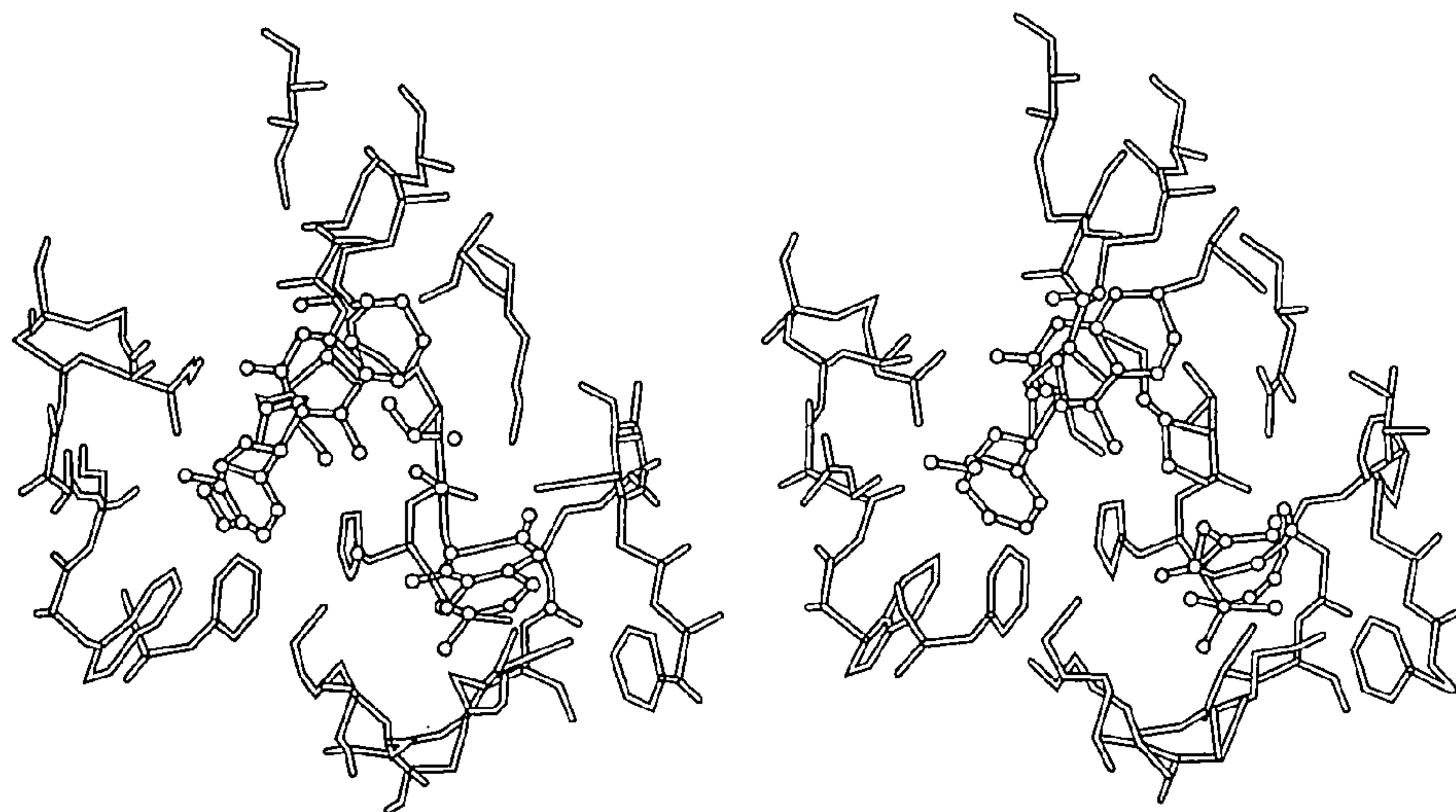
DETAILS OF NCP014 BINDING WITHIN THE 11A SITE
