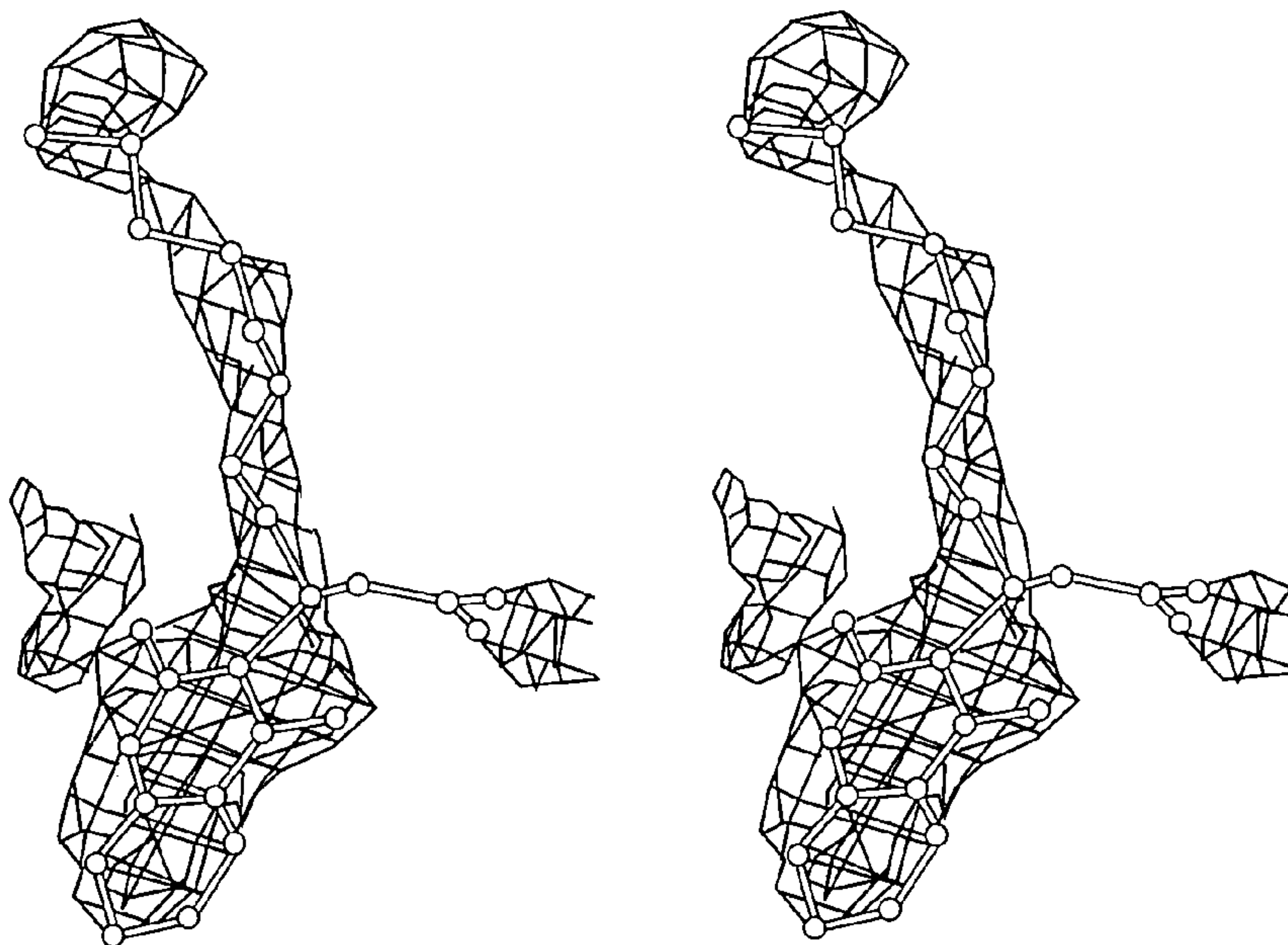
DIFFERENCE ELECTRON DENSITY (UNREFINED) OF NCP014 IN SITE 1B
