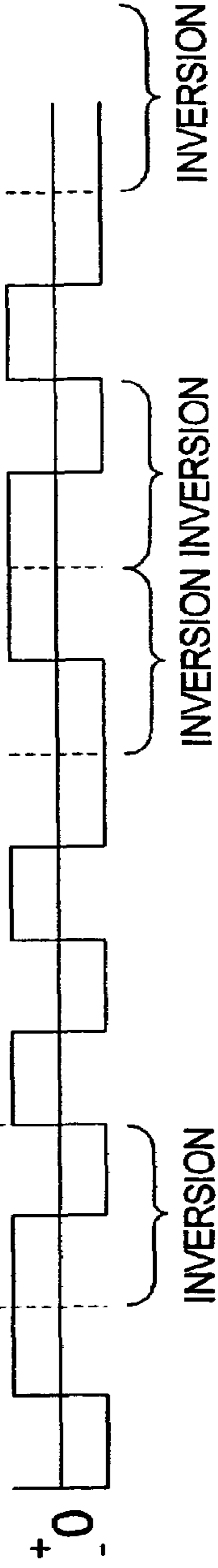
FIG. 16C MODULATING WAVE (DIFFERENTIAL CONVERSION)
