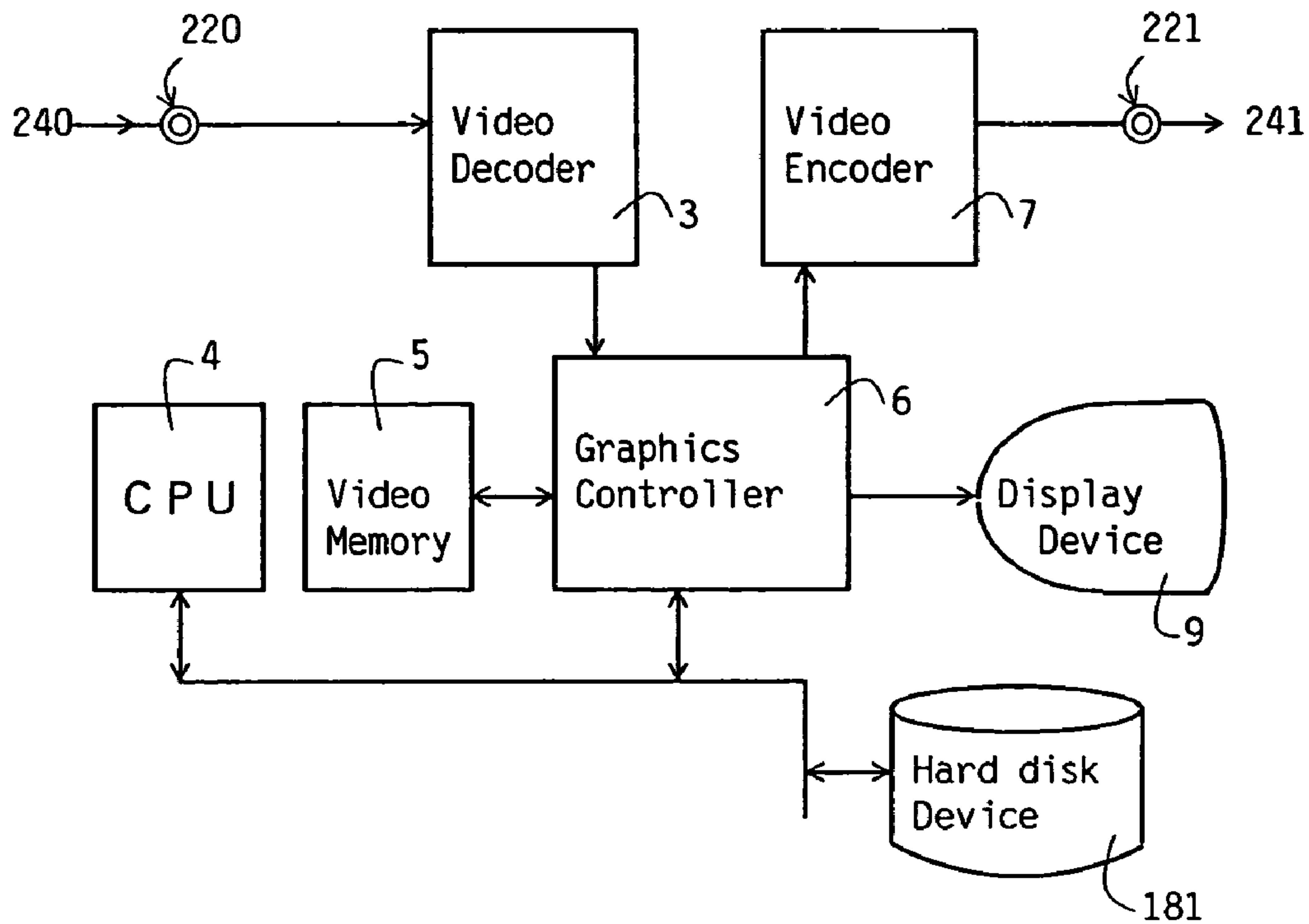
FIG. 7 (PRIOR ART)
