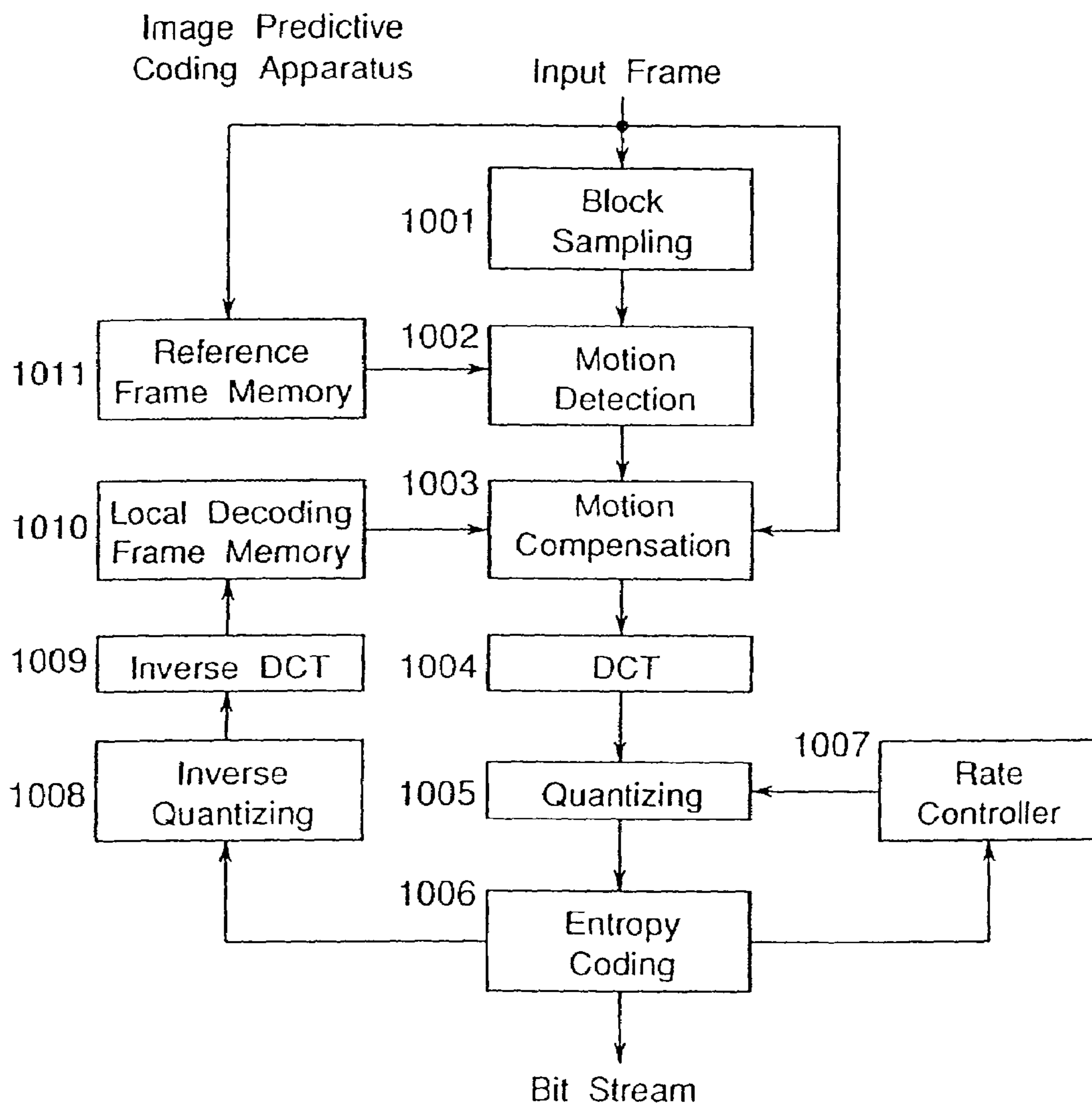
Fig. 14 PRIOR ART
