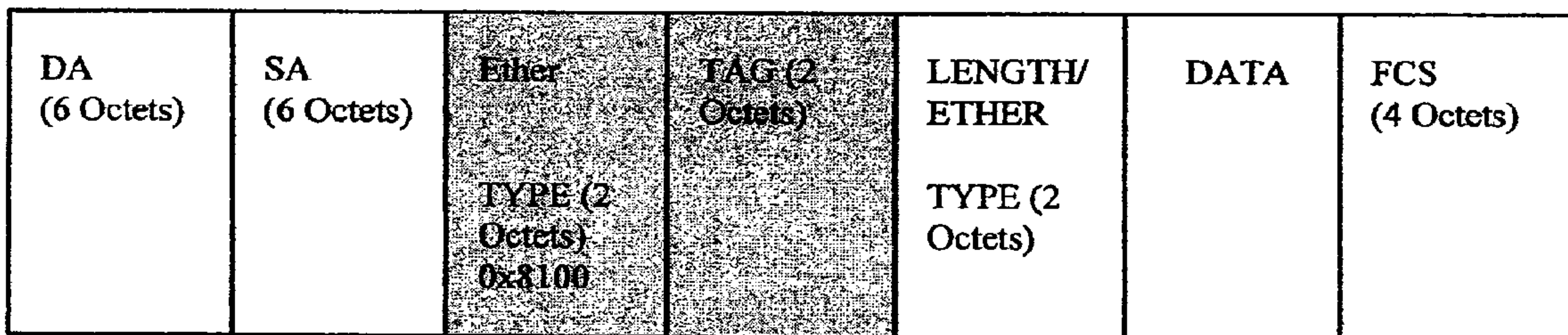
FIG. 3 (PRIOR ART)
