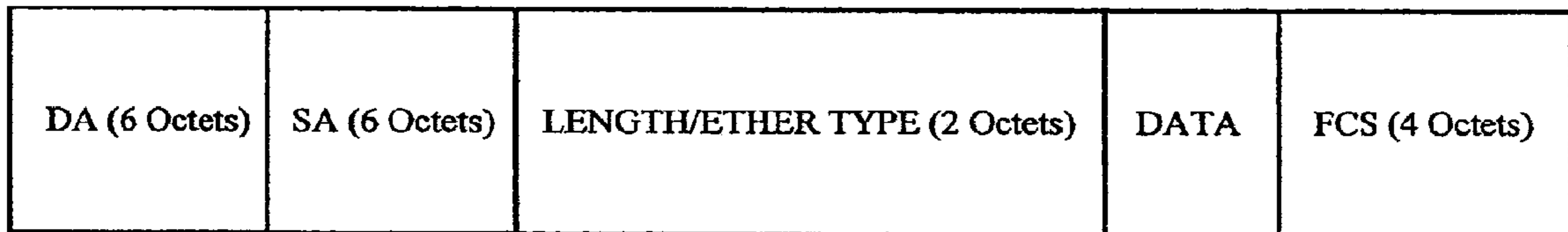
FIG. 2 (PRIOR ART)
