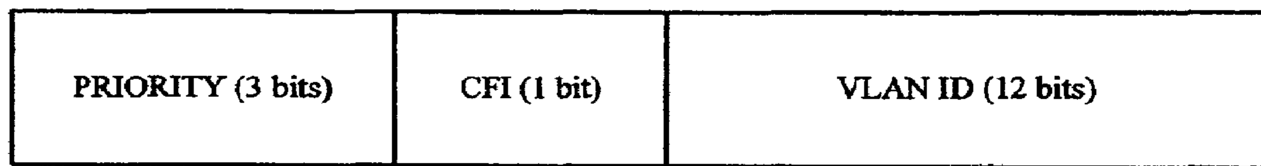
FIG. 4 (PRIOR ART)
