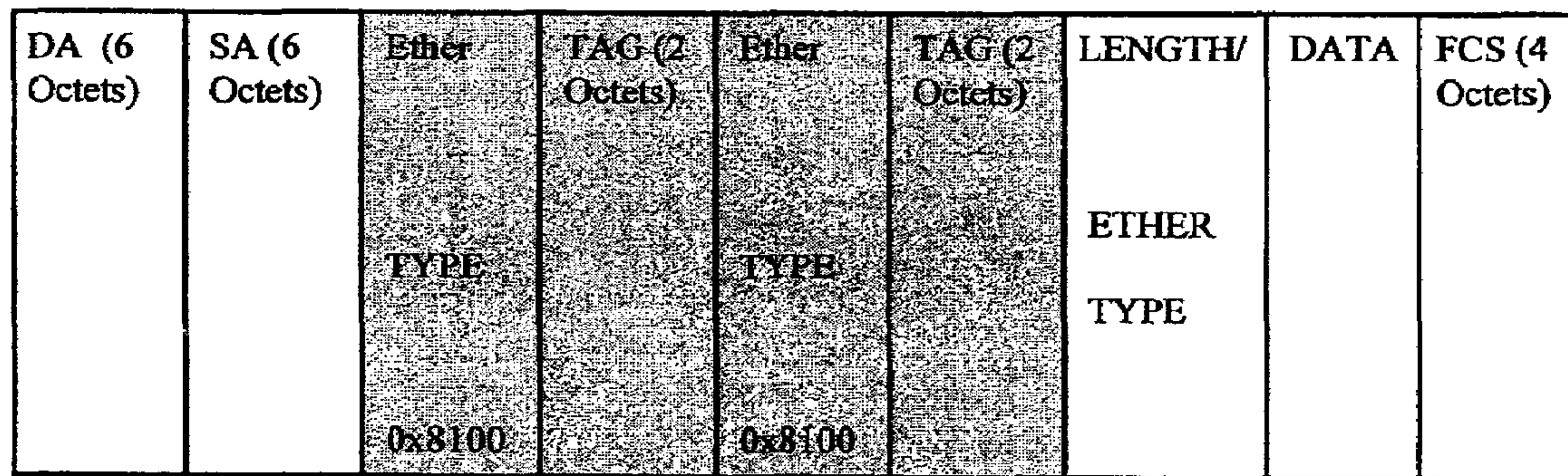
FIG. 5 (PRIOR ART)
