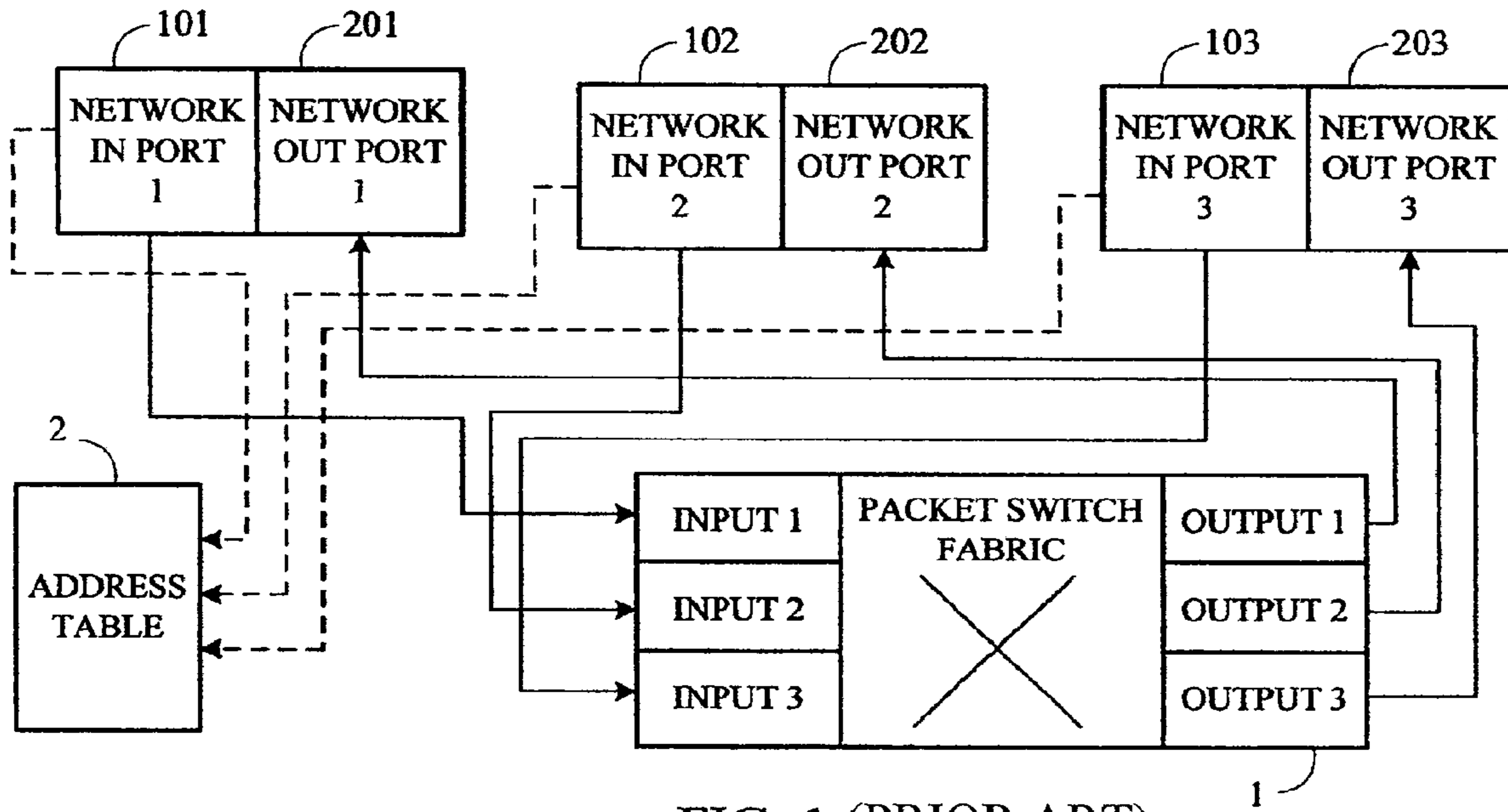
FIG. 1 (PRIOR ART)
