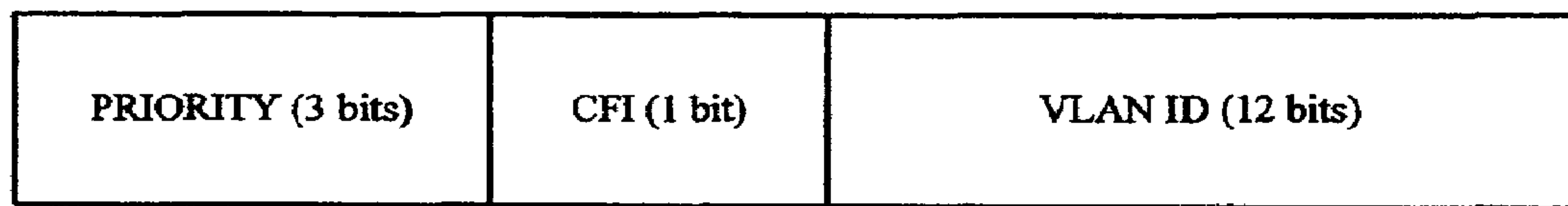
FIG. 4 (PRIOR ART)
