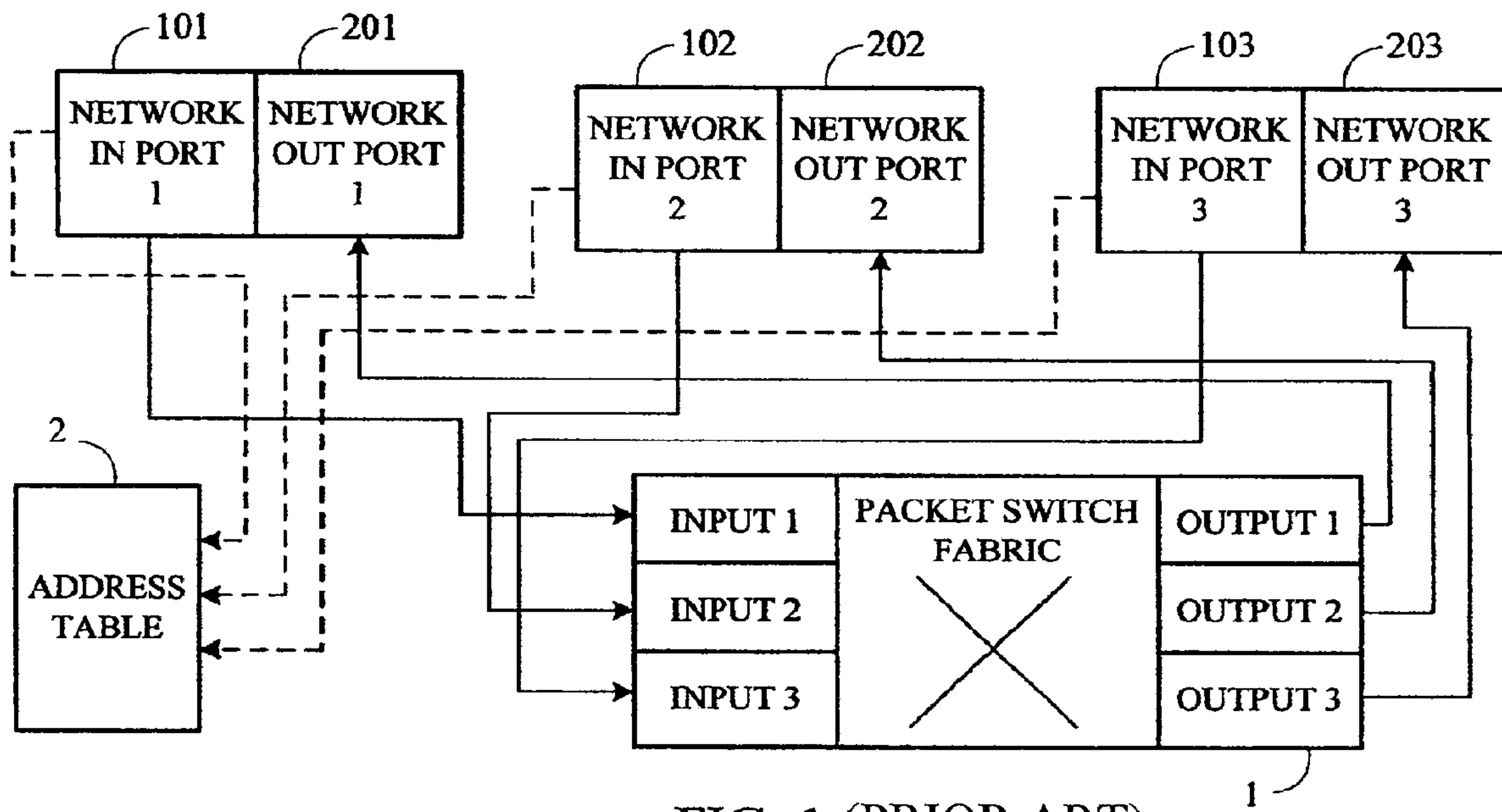
FIG. 1 (PRIOR ART)
