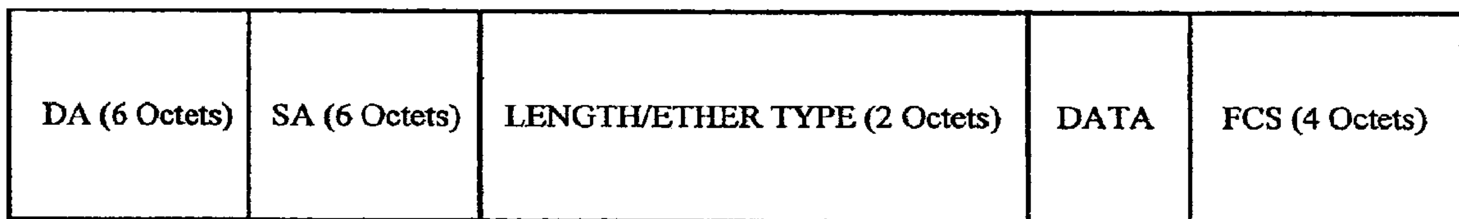
FIG. 2 (PRIOR ART)
