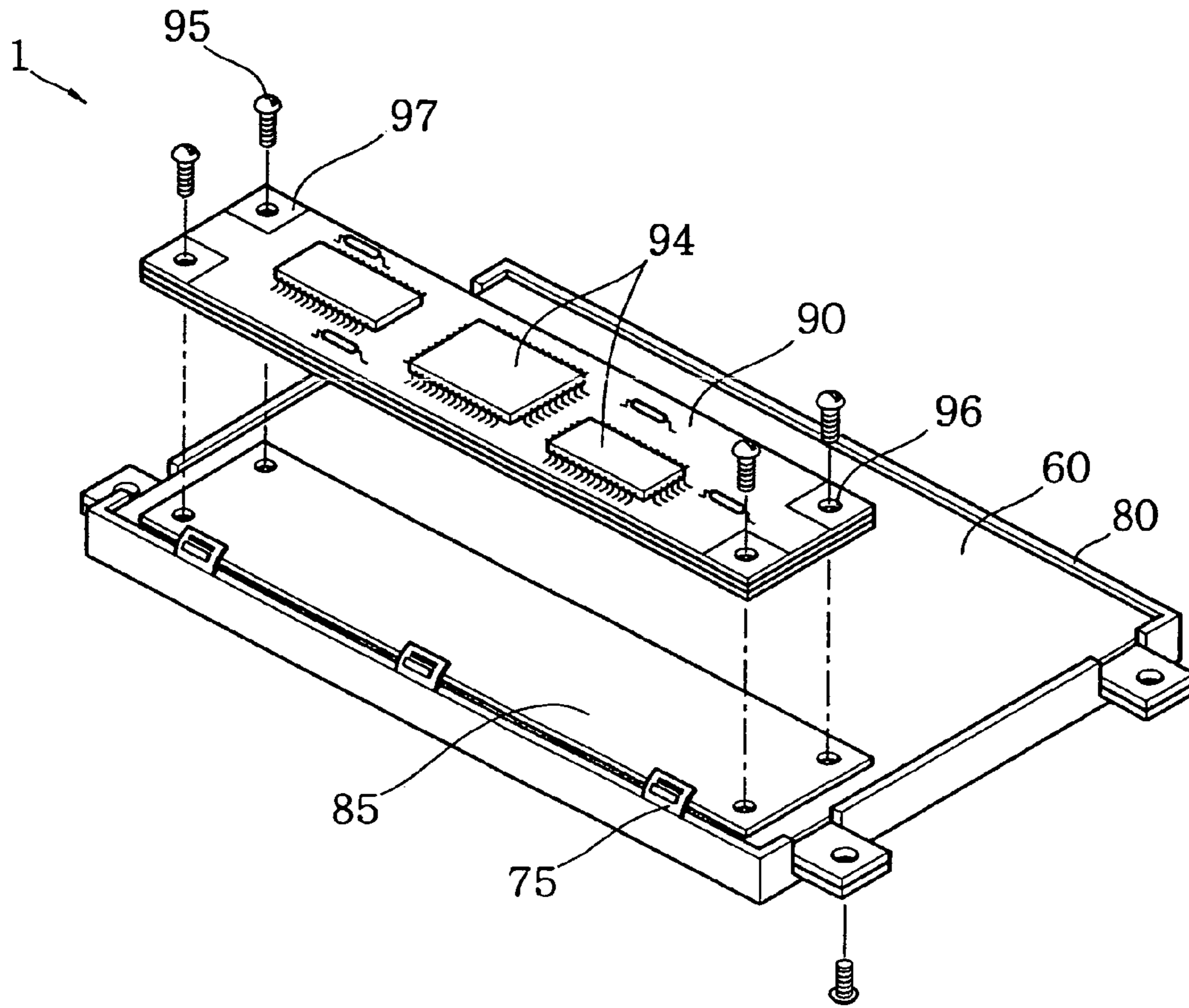
FIG. 2 (PRIOR ART)
