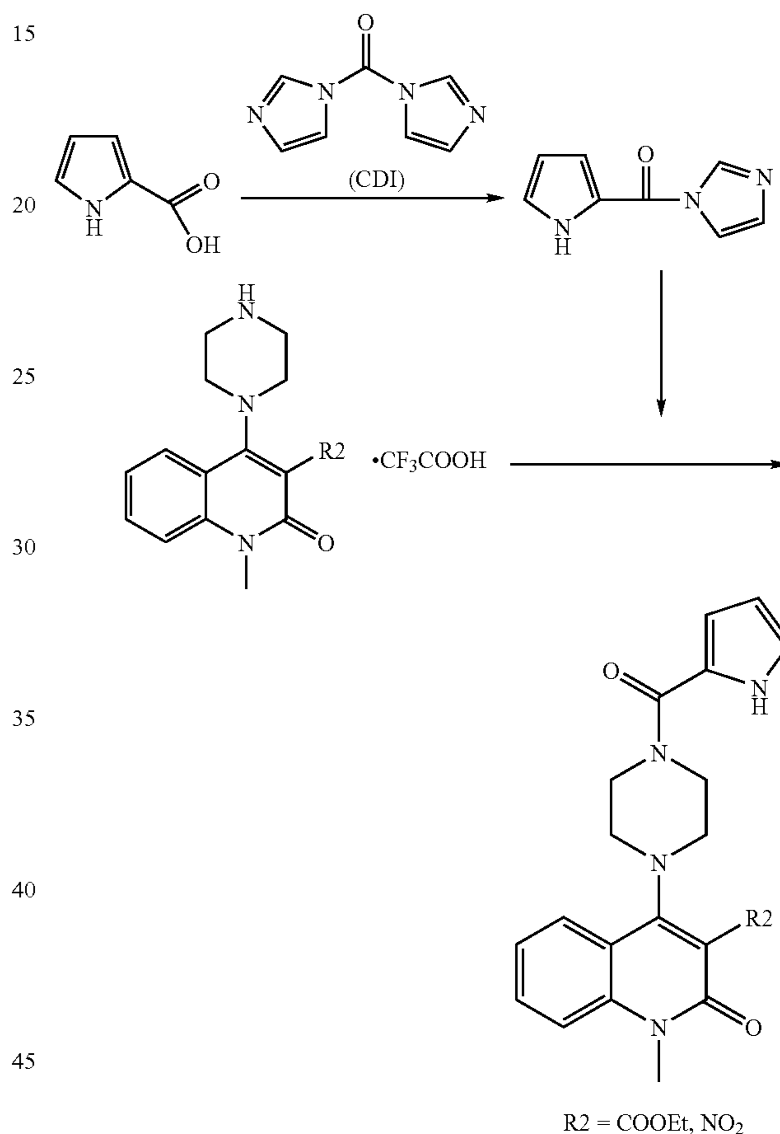
Reaction Scheme 17
