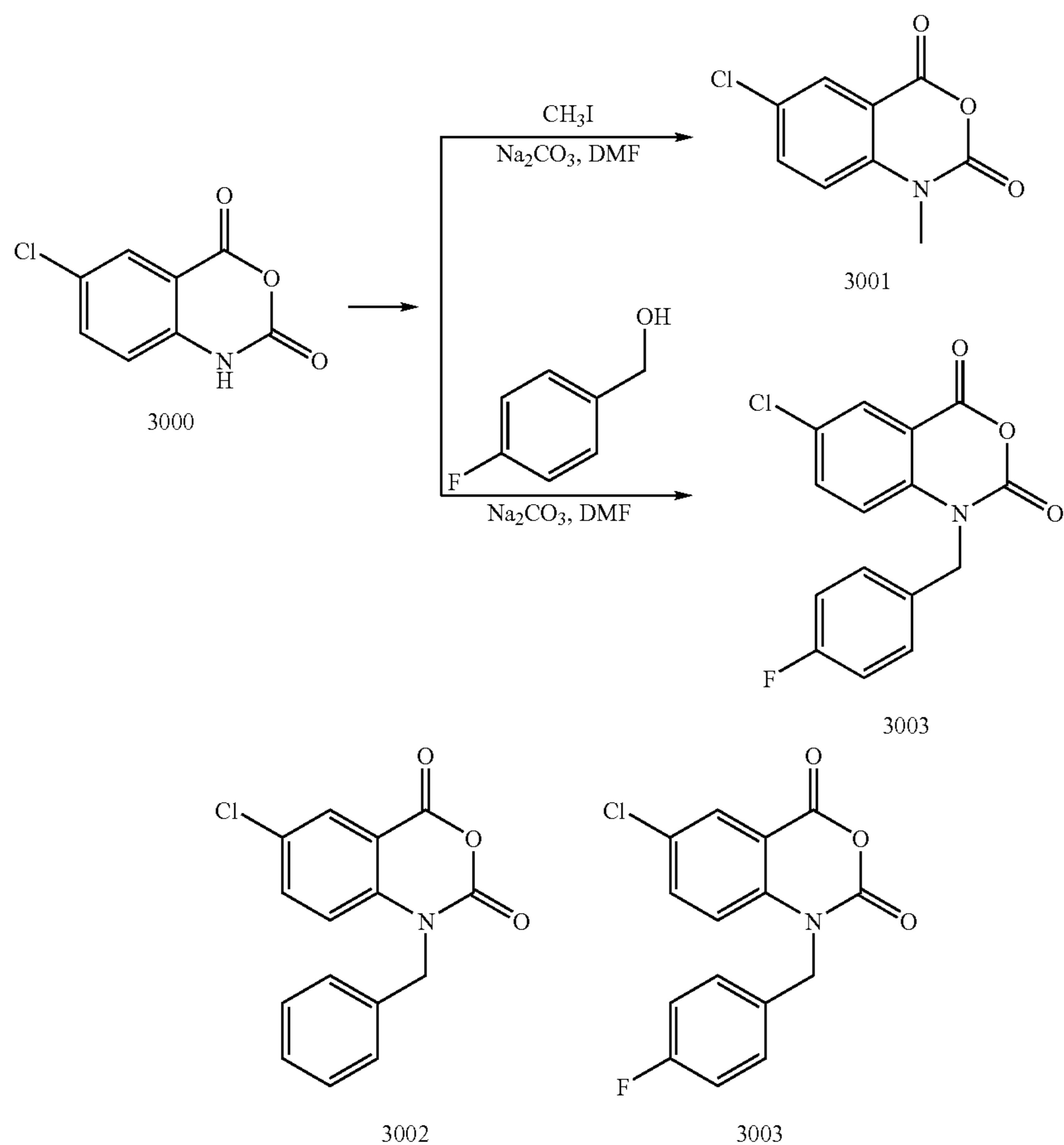
Reaction Scheme 26
