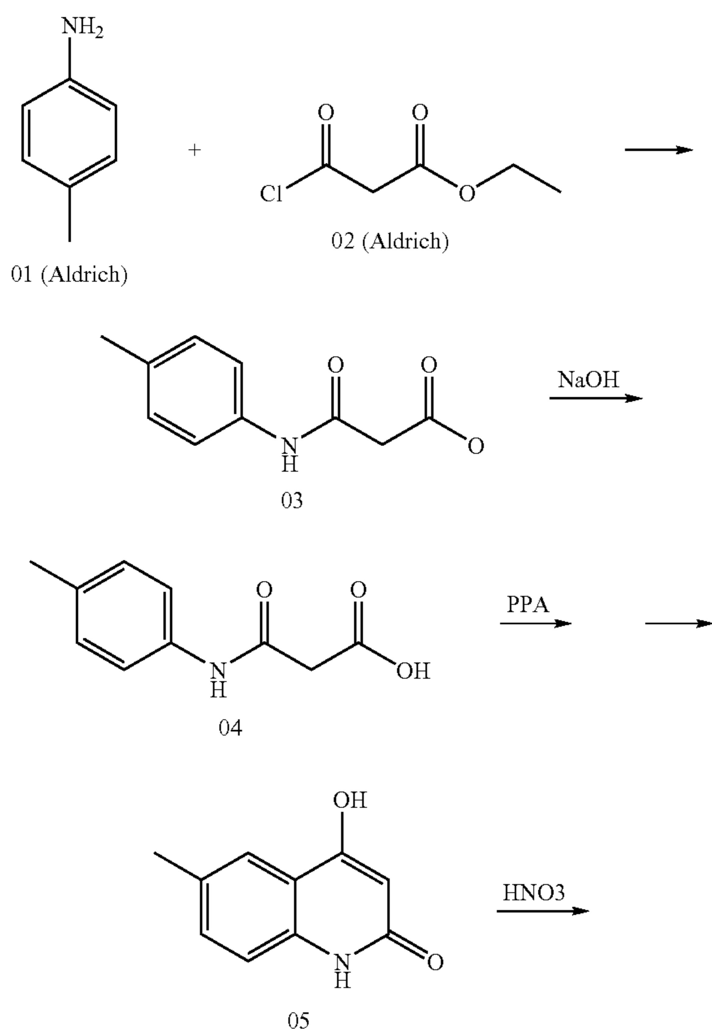
Reaction Scheme 25
