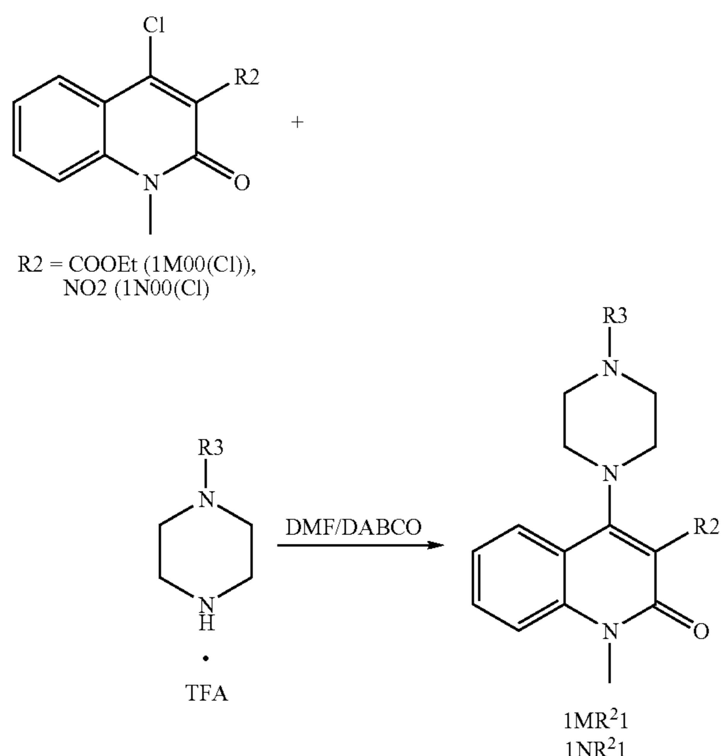
Reaction Scheme 16
