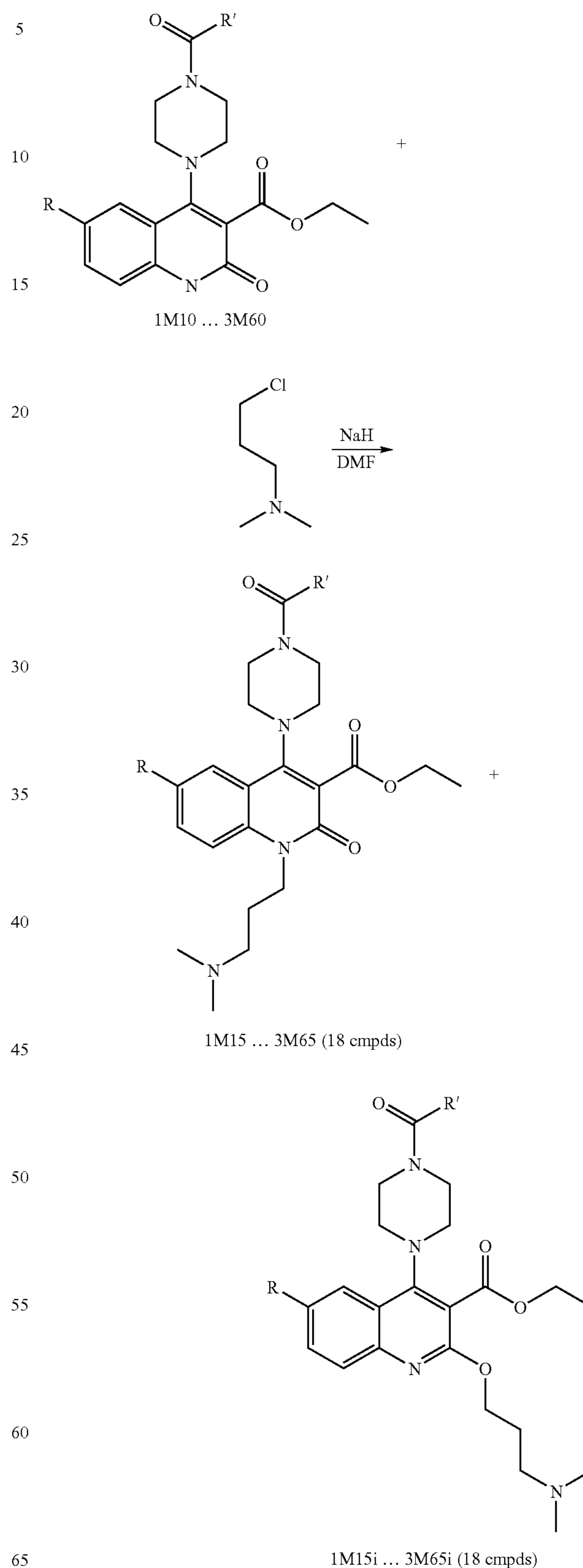
Reaction Scheme 24
