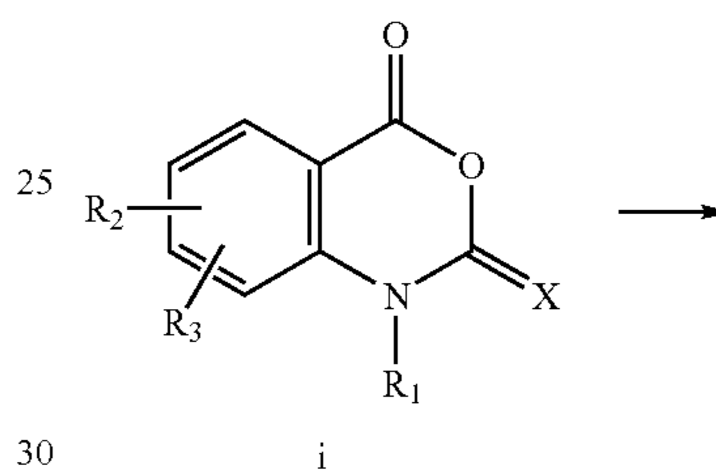
Reaction Scheme 1
