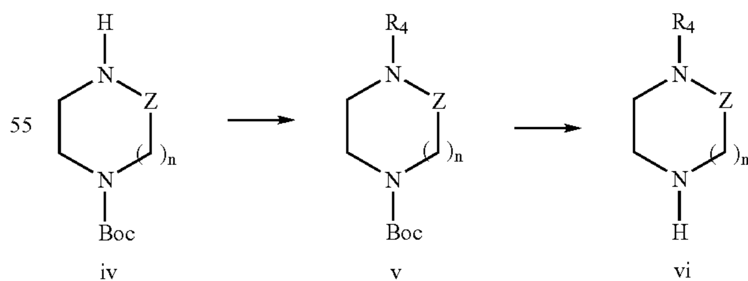
Reaction Scheme 2
