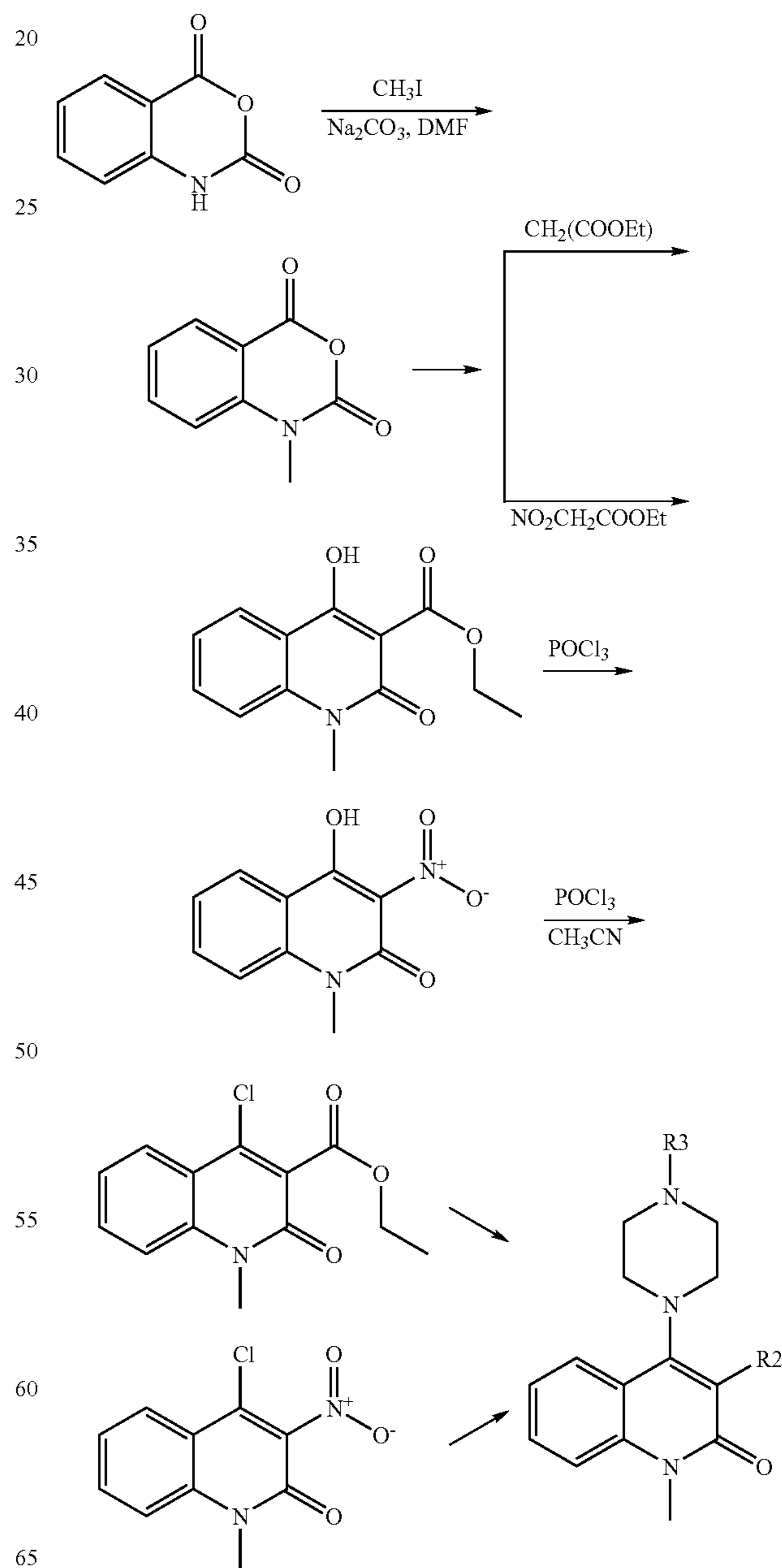
Reaction Scheme 9
