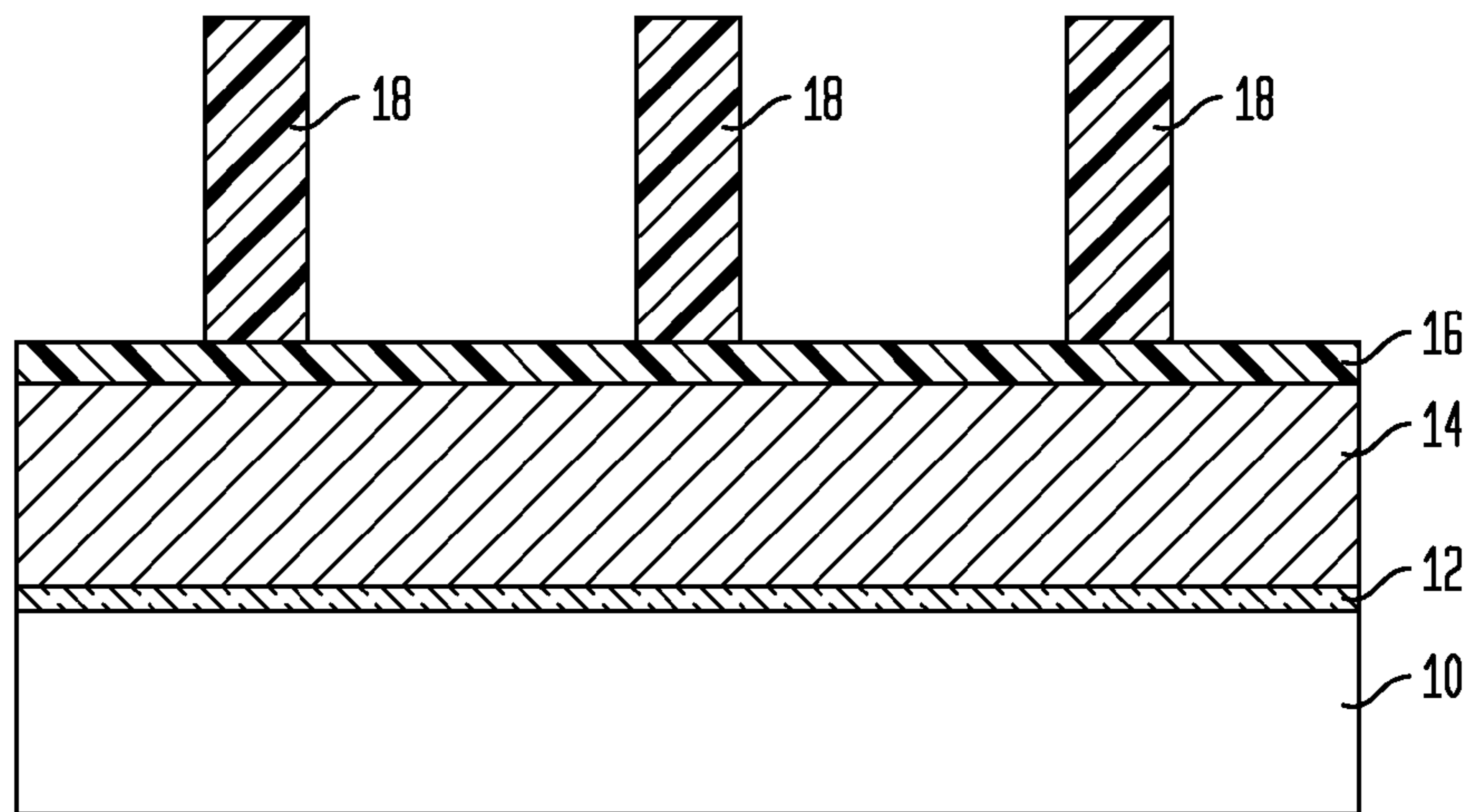
FIG. 1 (PRIOR ART)
