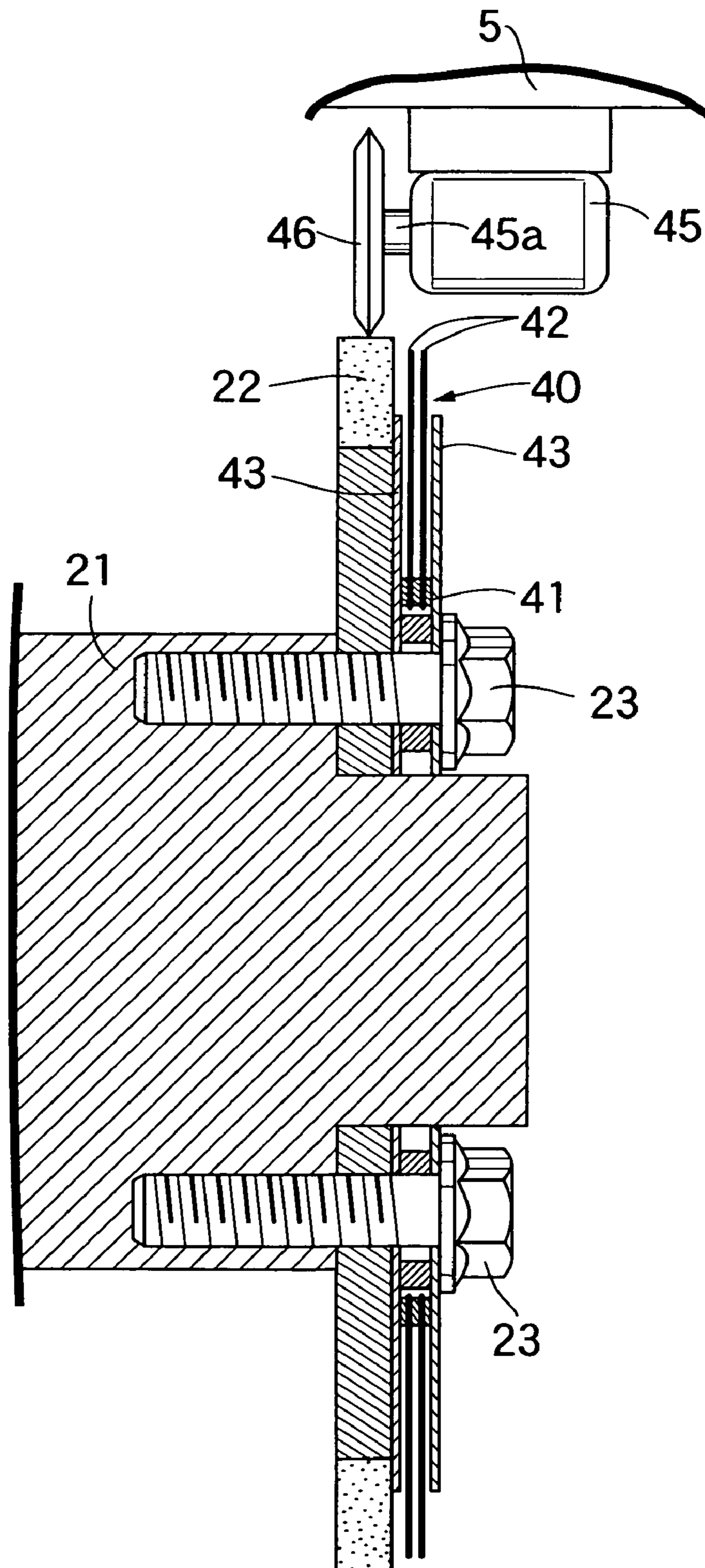
FIG.5 DURING DRESSING
