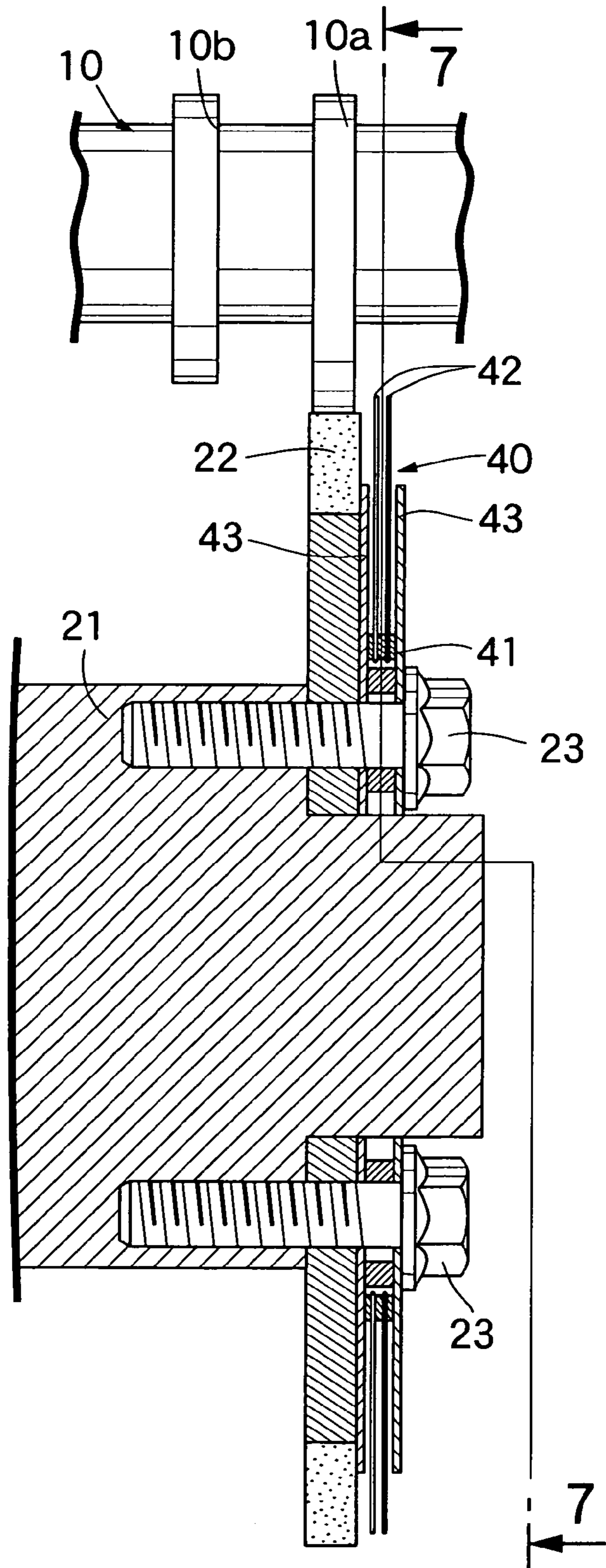
FIG.6 DURING GRINDING
