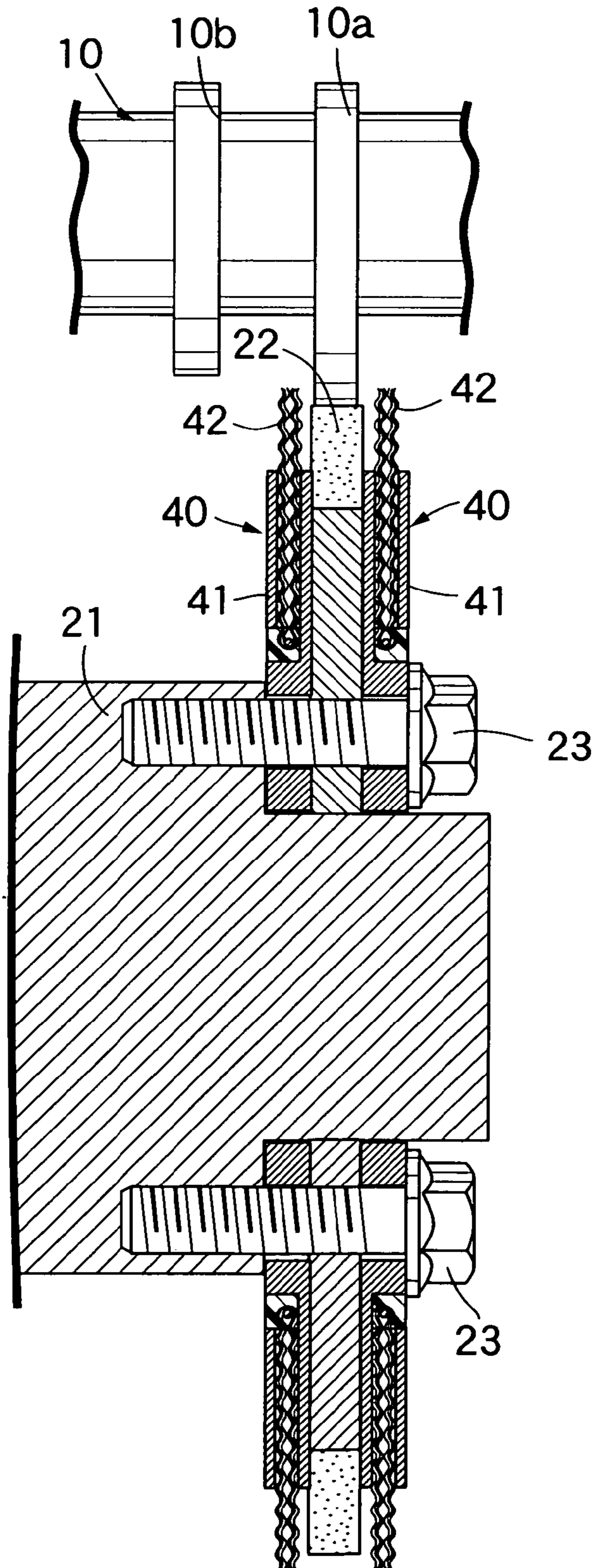
FIG. 12 DURING GRINDING
