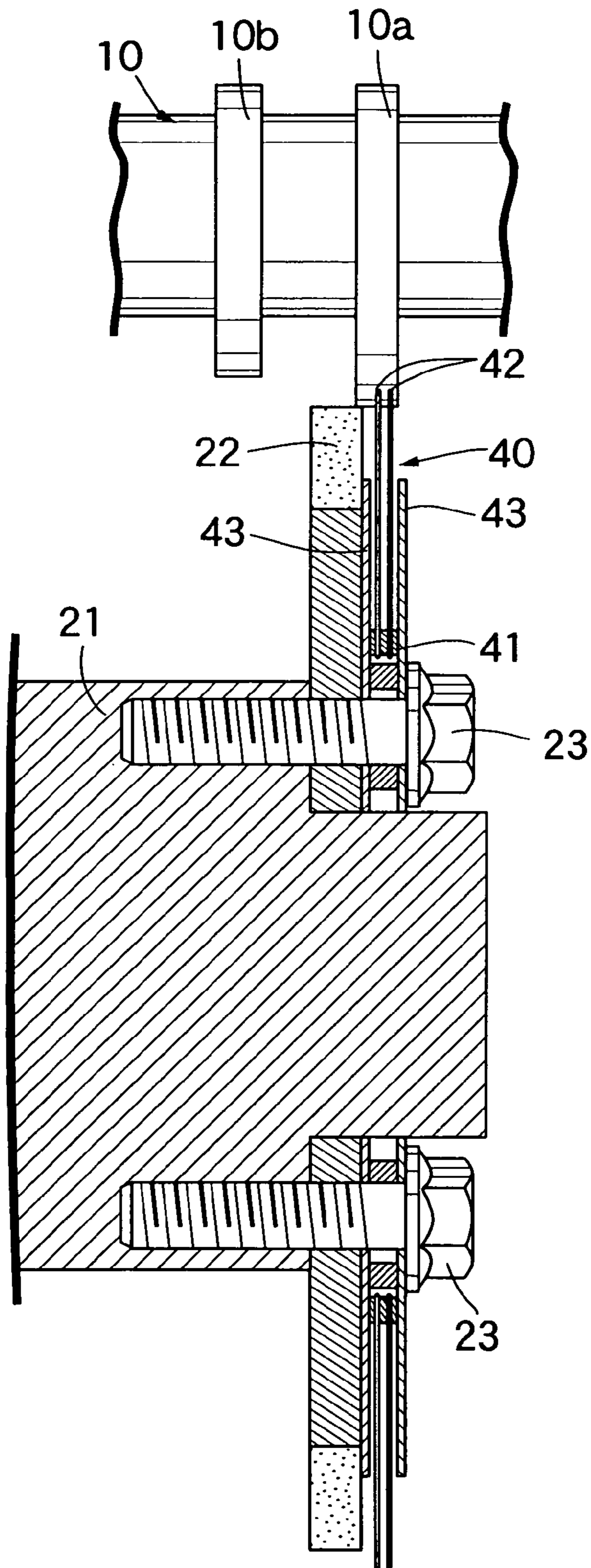
FIG. 8 DURING BRUSHING
