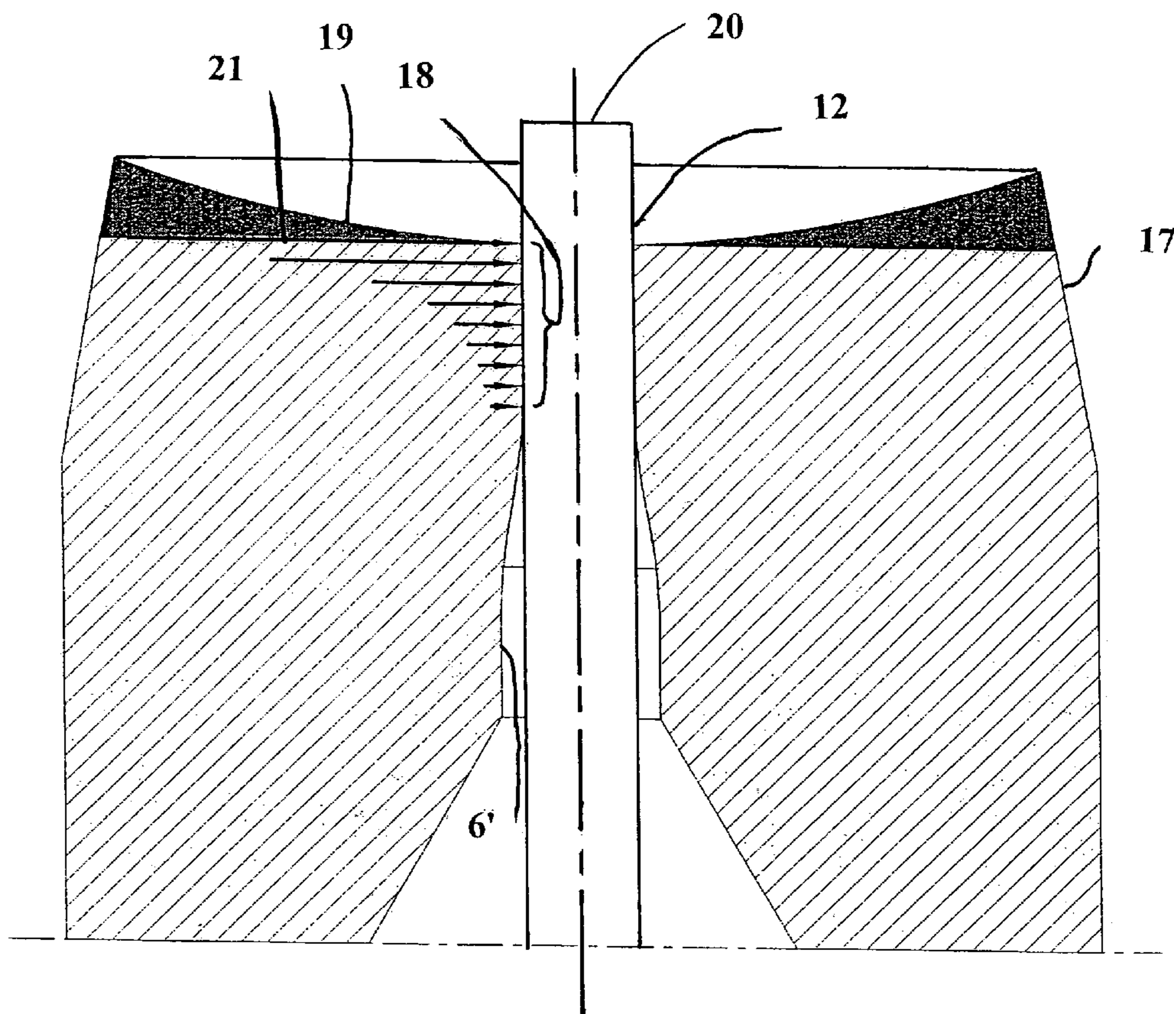
Fig.10 (Prior art)
