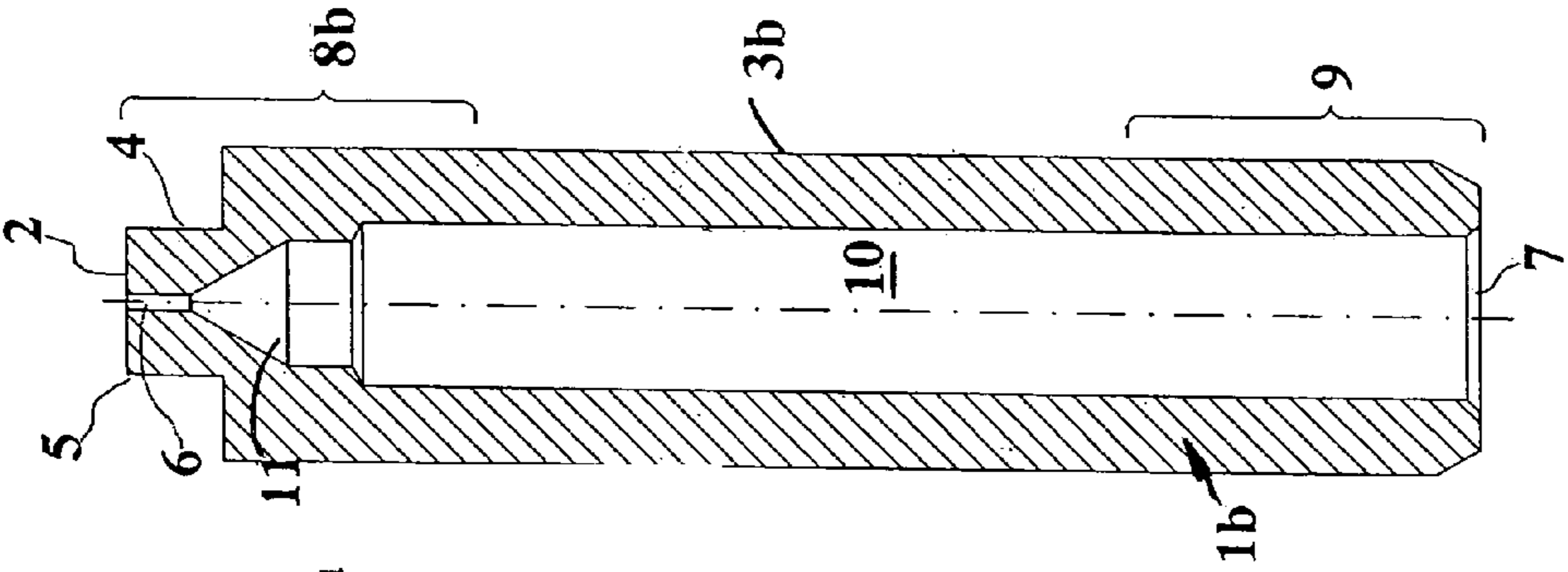
Fig. 3 (Prior art)
