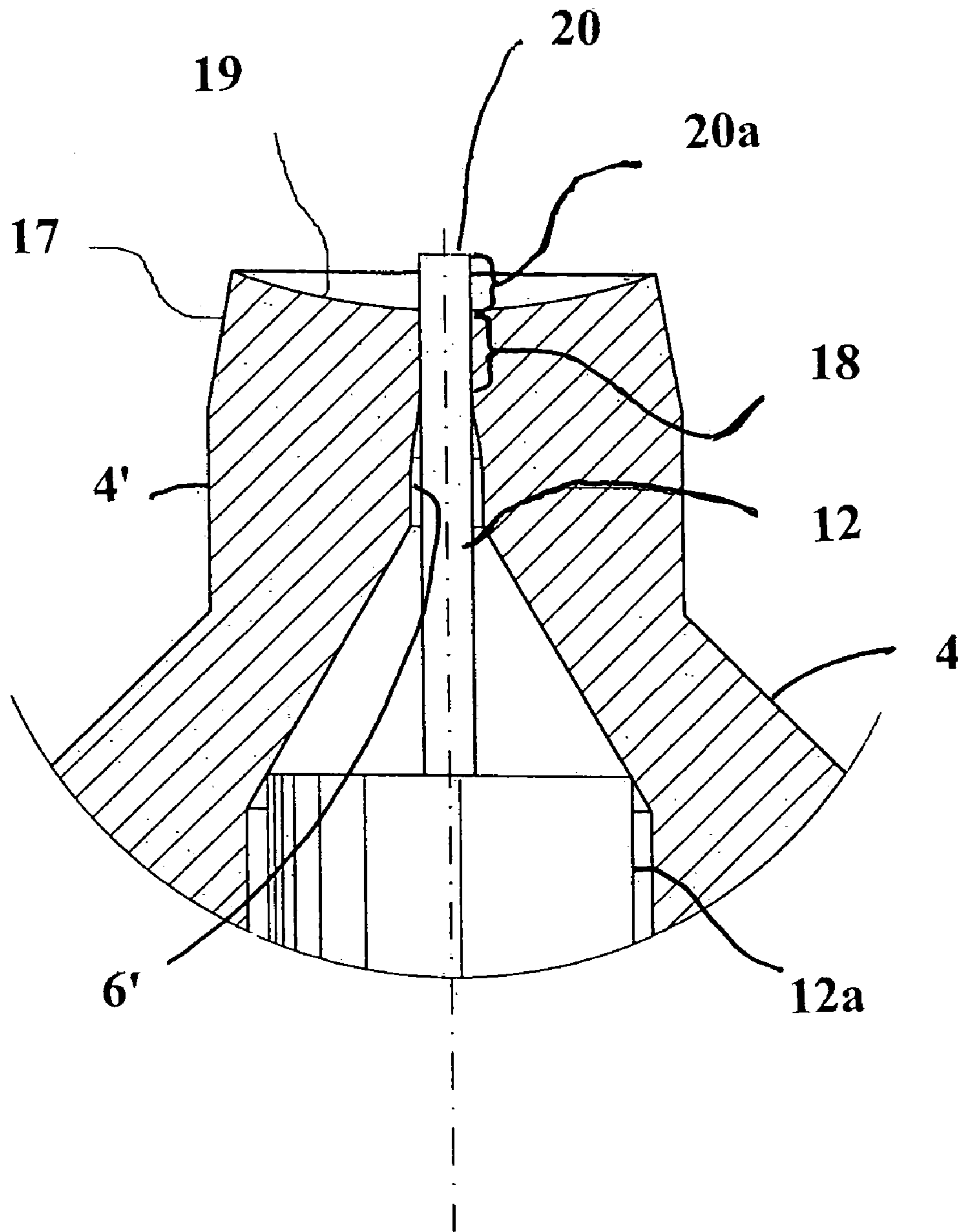
Fig. 8 (Prior art)
