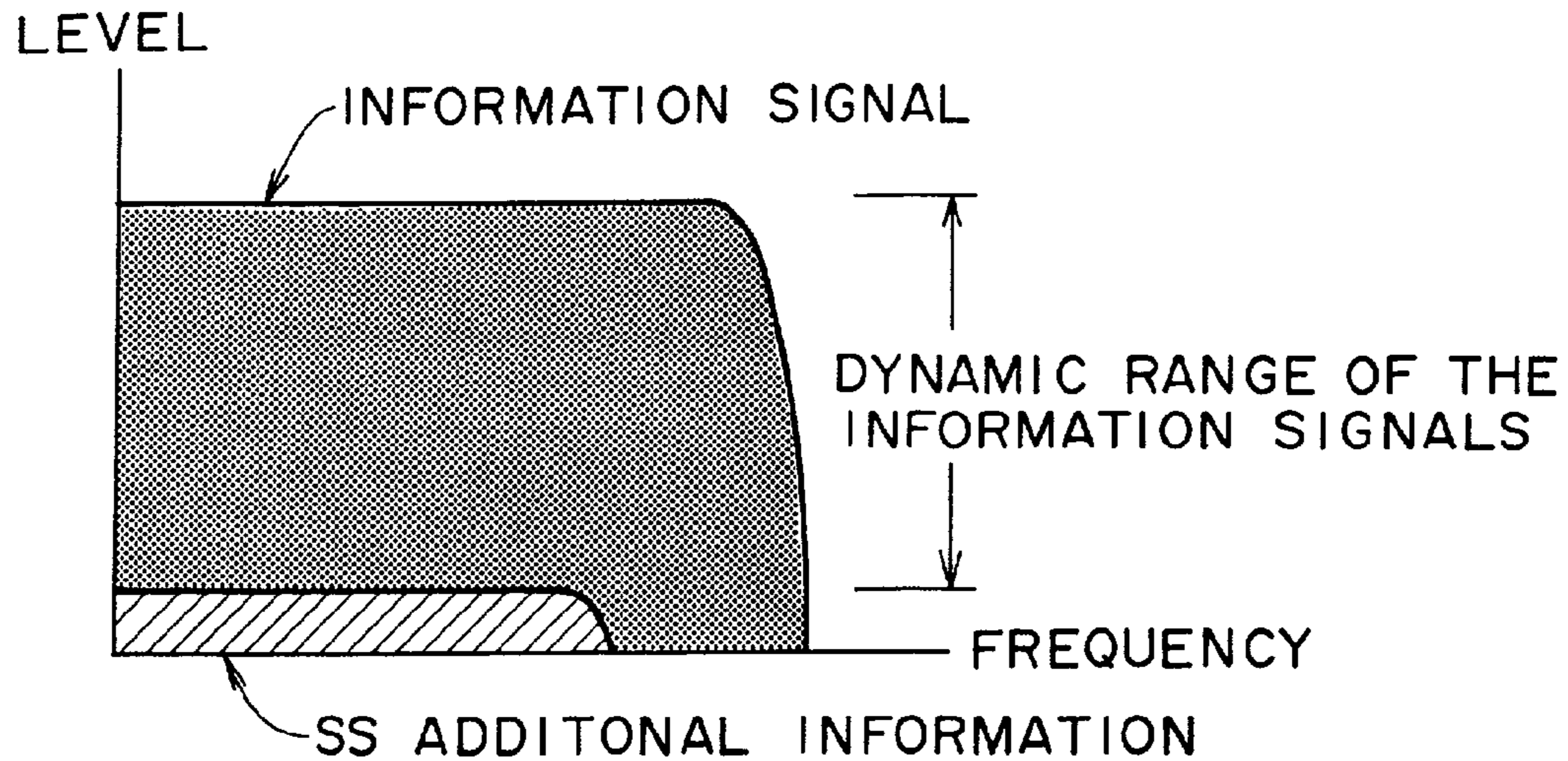
SPECTRUM OF INFORMATION SIGNALS TO WHICH THE SS ADDITIONAL INFORMATION IS ADDED
