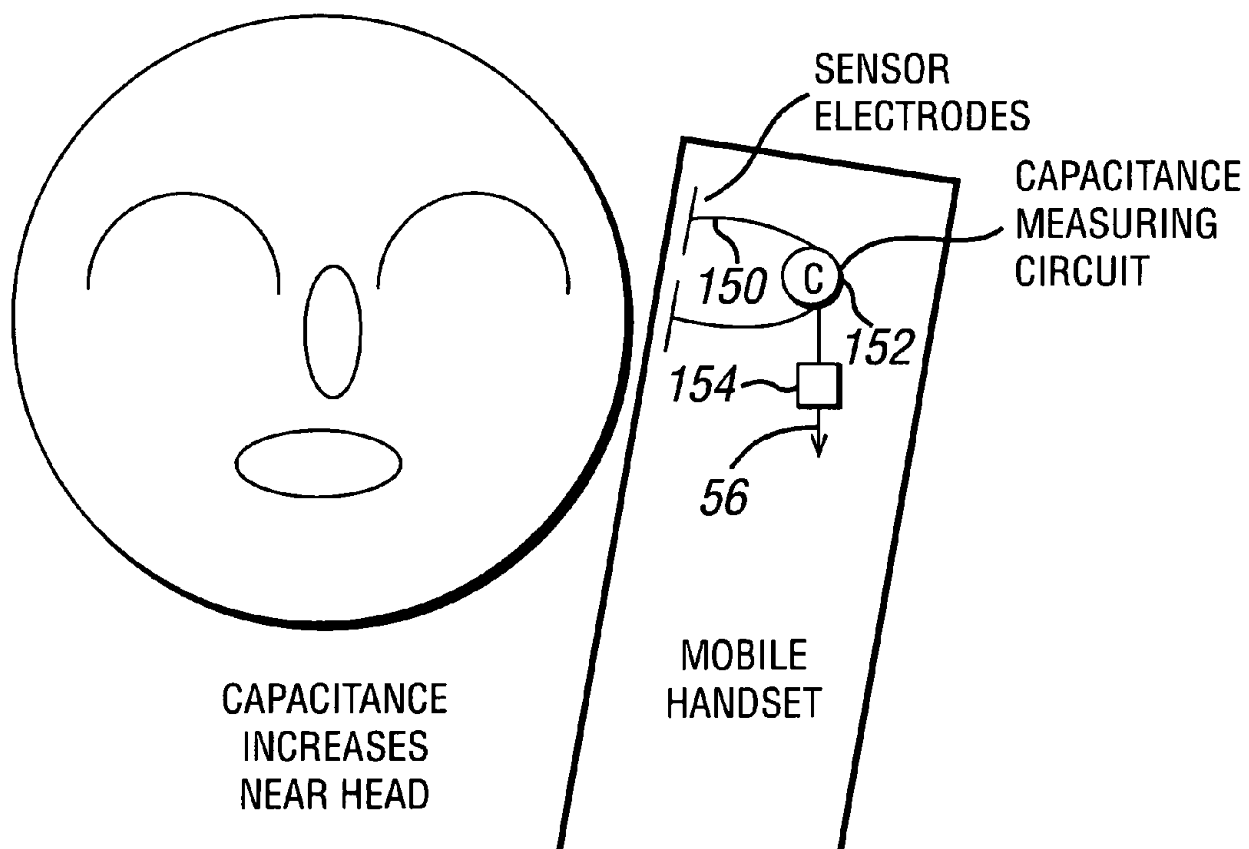
FIG. 5 CAPACITIVE HEAD PROXIMITY DETECTION
