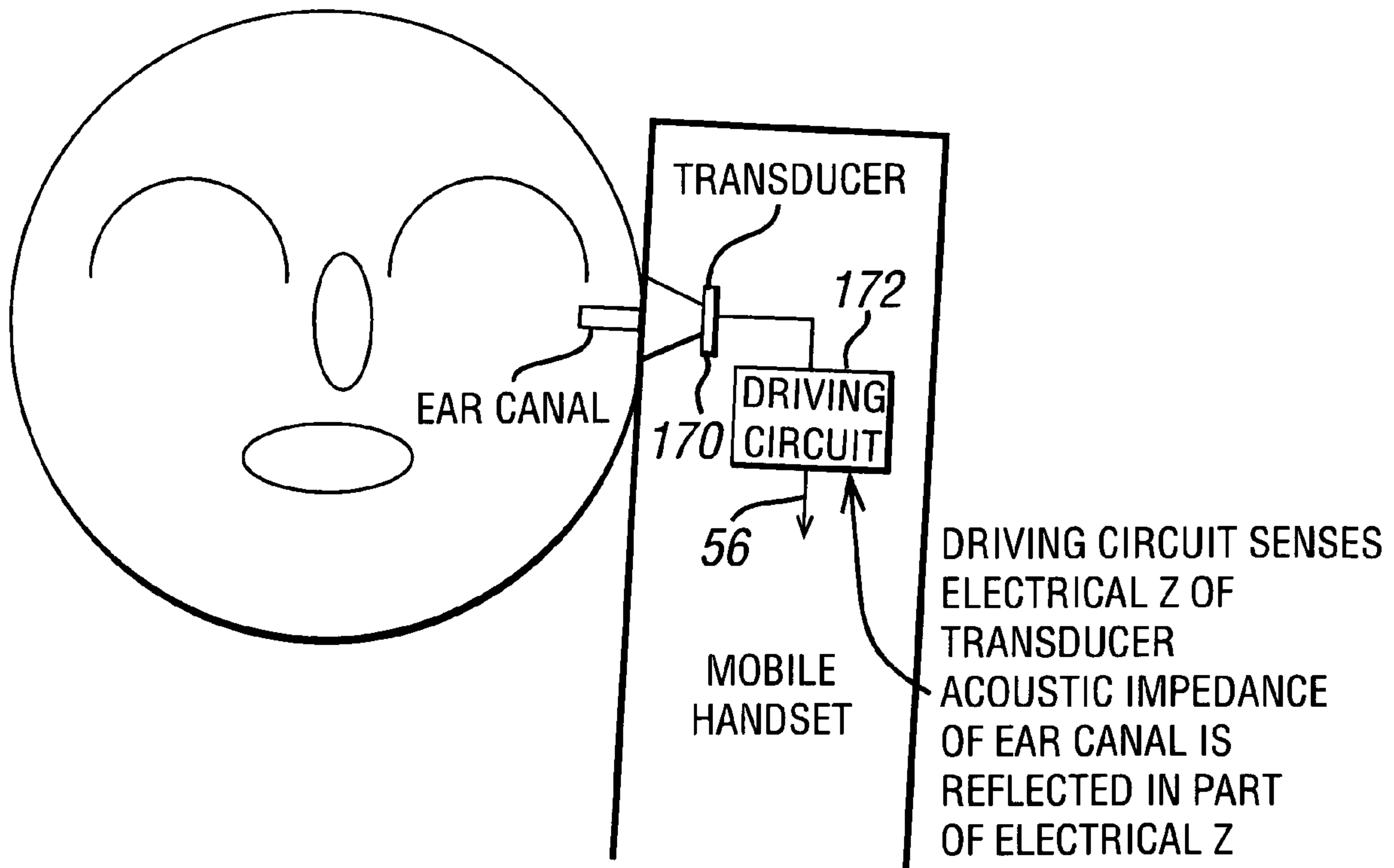
FIG. 7 ACOUSTIC IMPEDANCE EAR DETECTION
