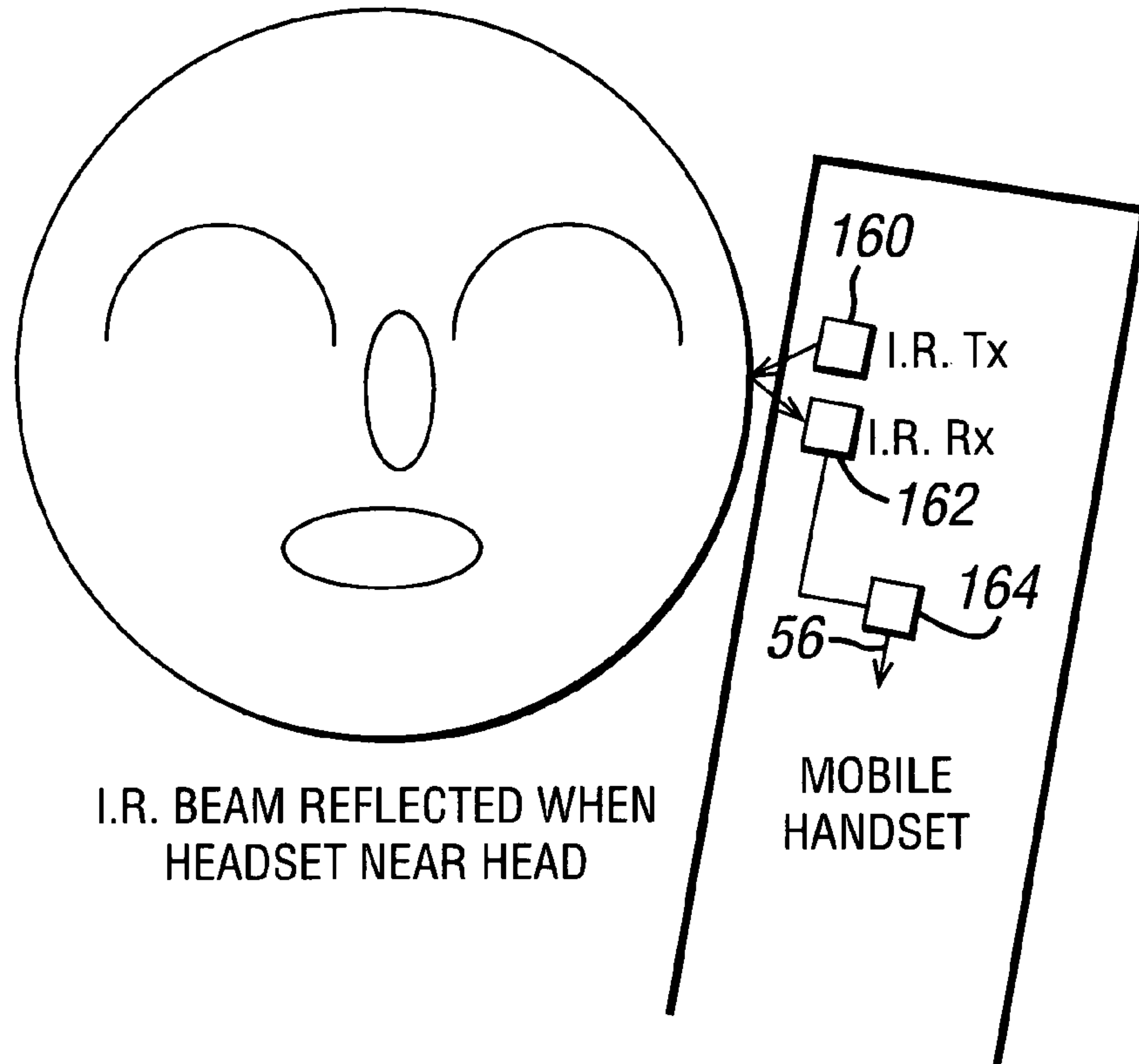
FIG. 6 I.R. HEAD PROXIMITY DETECTION
