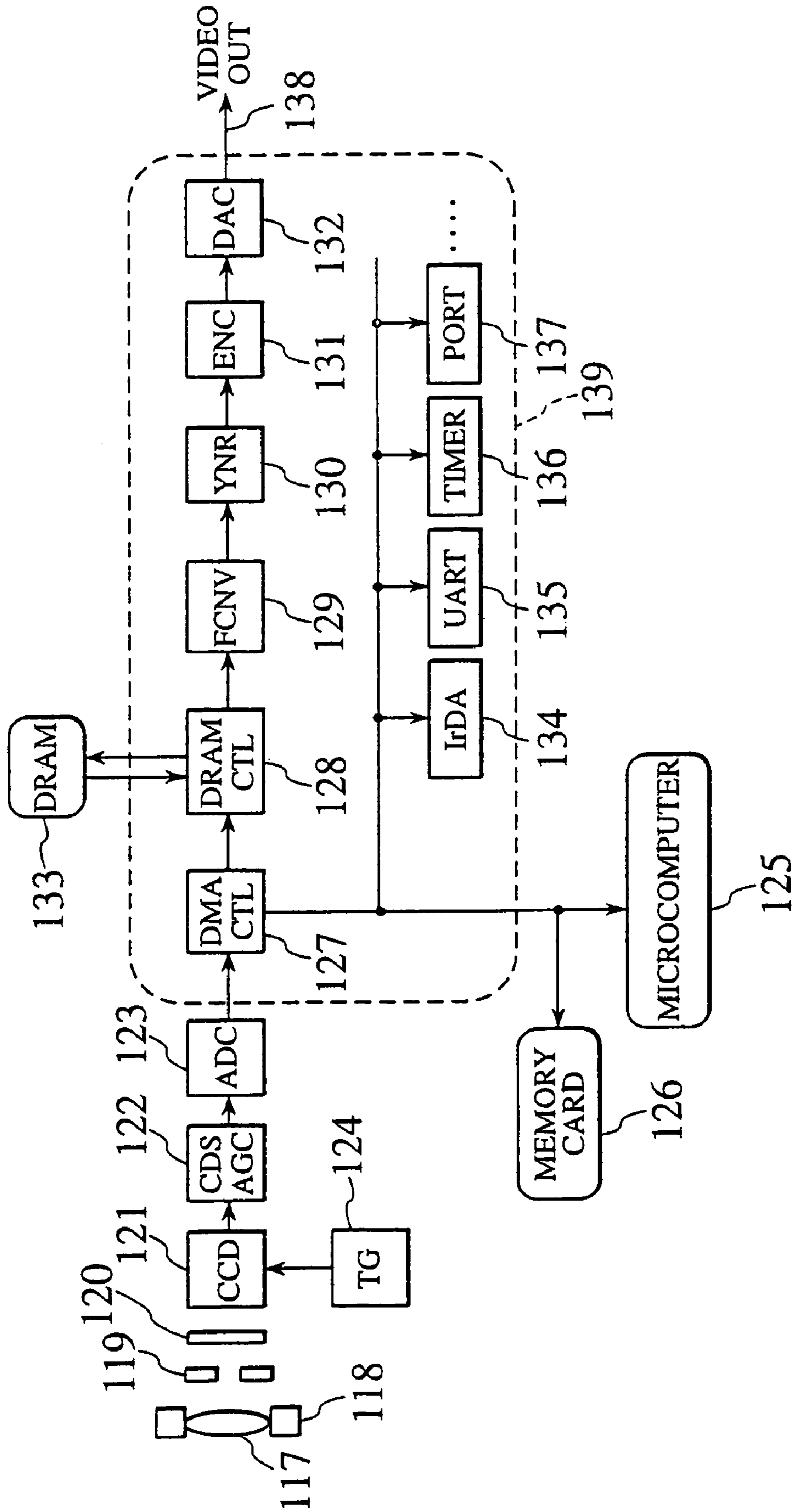
FIG. 3 PRIOR ART
