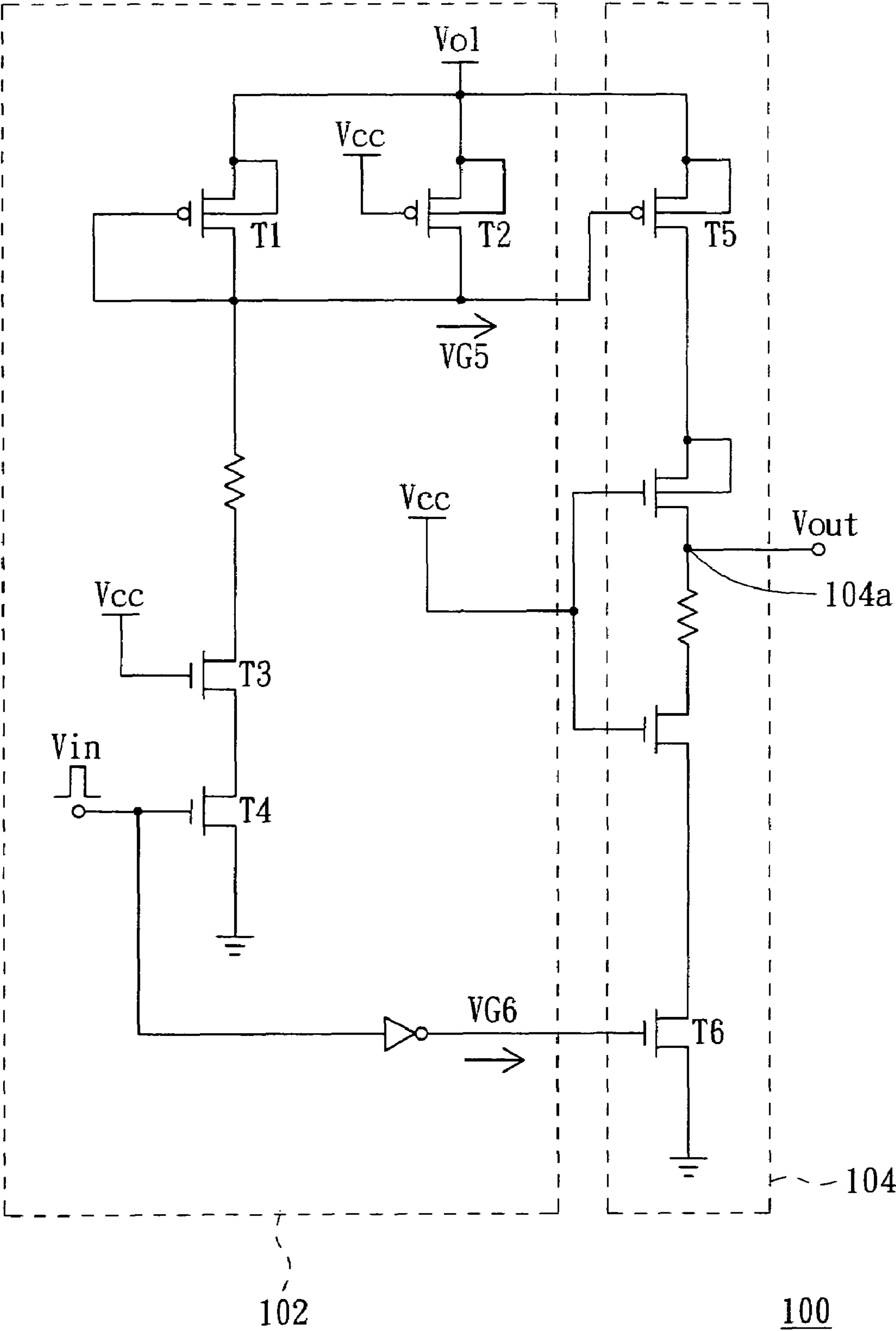
FIG. 1 (PRIOR ART)
