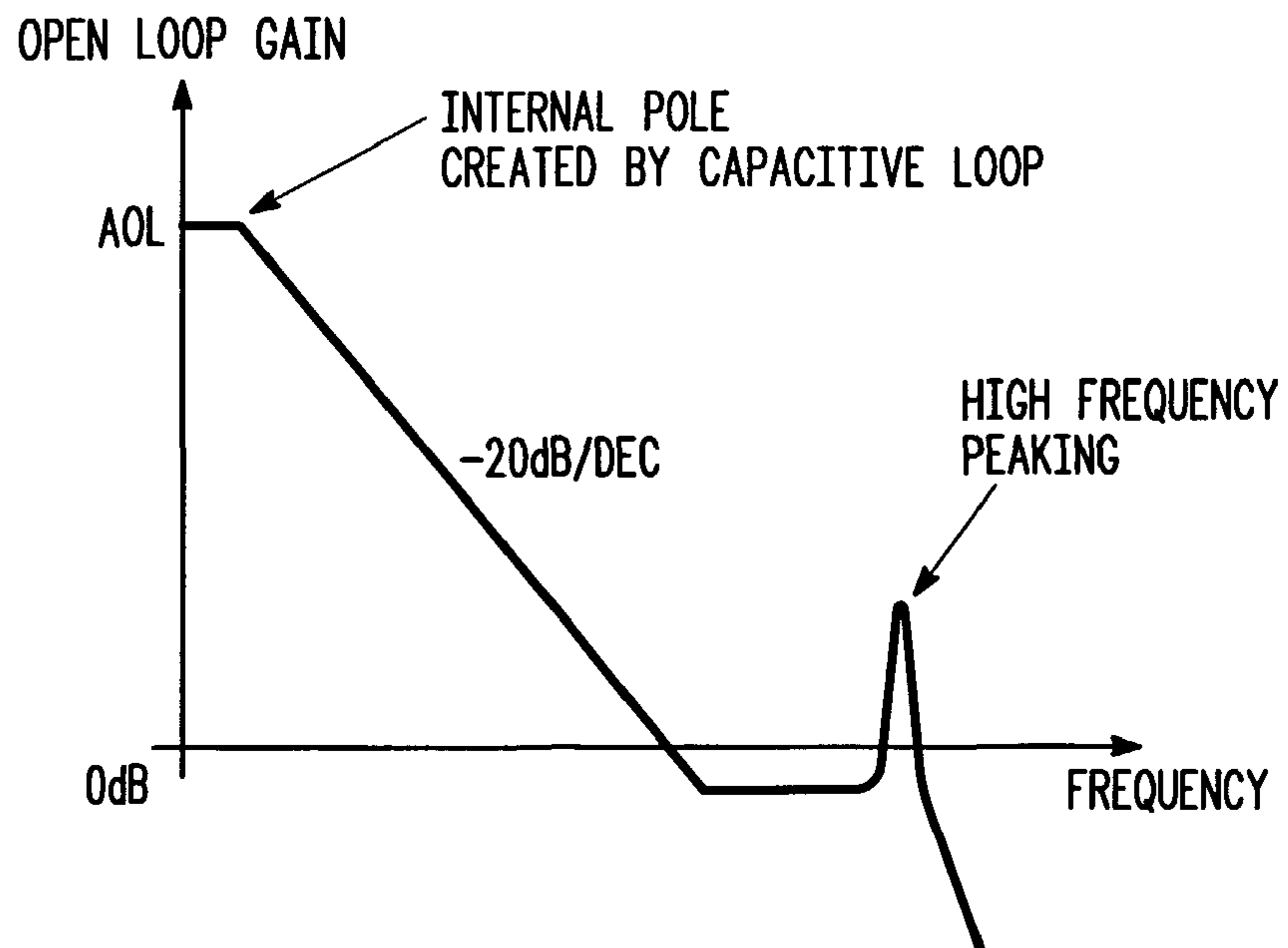
FIG. 4 -PRIOR ART-
