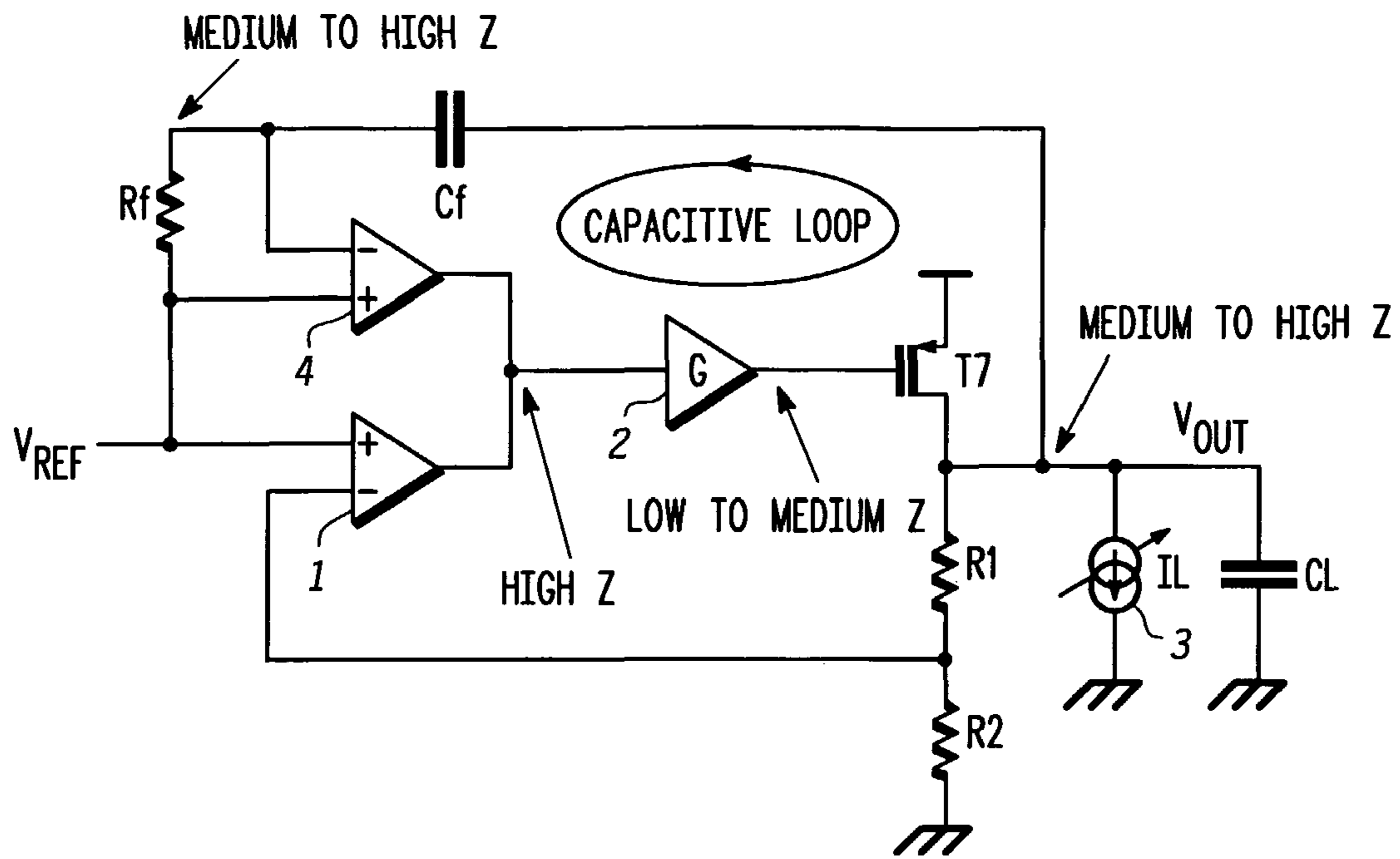
FIG. 3 -PRIOR ART-
